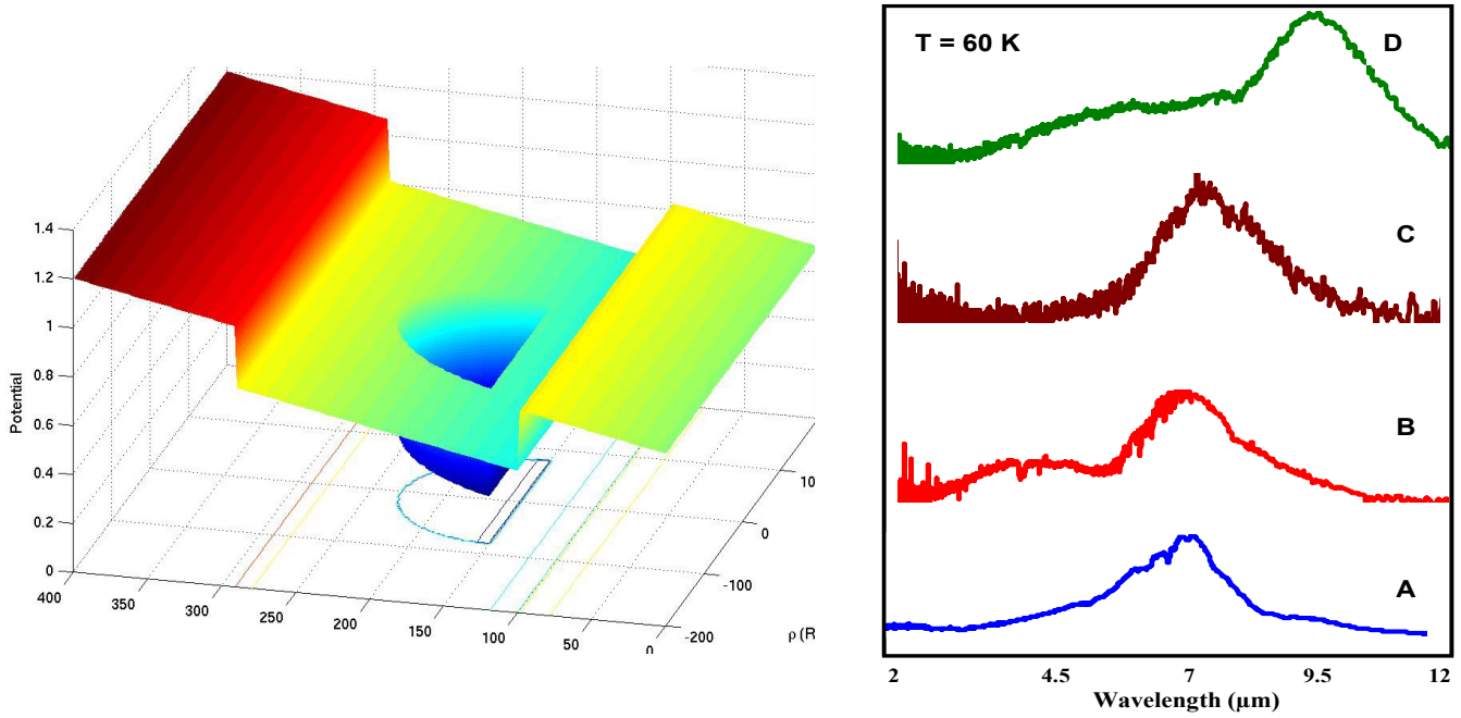
Fig. 3: (a) Potential profile in a typical dots in a well structure and (b) normalized photoresponse per watt for DWELL sensors with different well widths. The wavelength shifts progressively from 7.3 μm to 9.7 μm.
