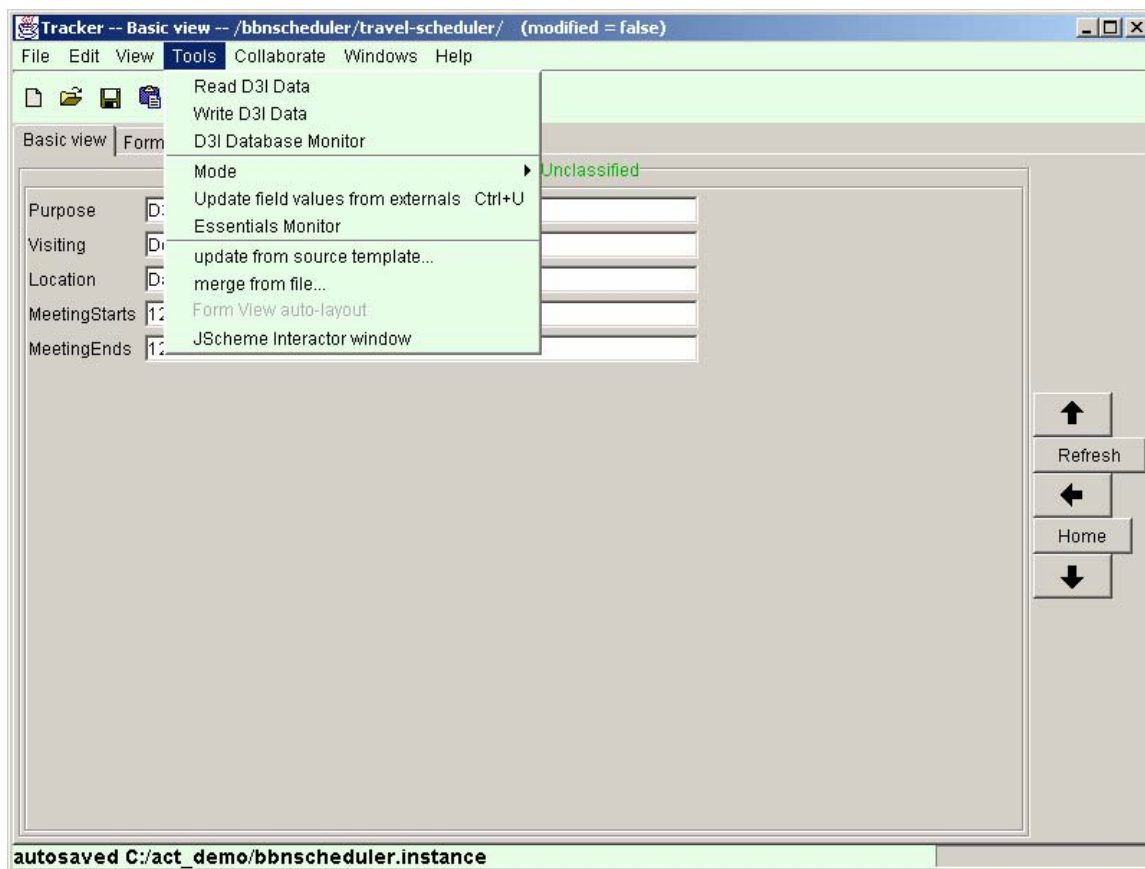
Figure 23 - D3i API
