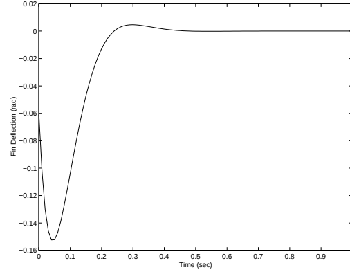
Figure 5 Fin Deflection for Feedback Linearization with Linear Quadratic Design
