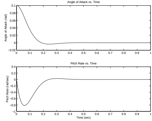
Figure 4 State Responses for Feedback Linearization with Linear Quadratic Design
