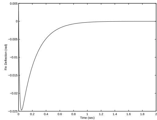
Figure 15 Fin Deflection with Predictive Control Design
