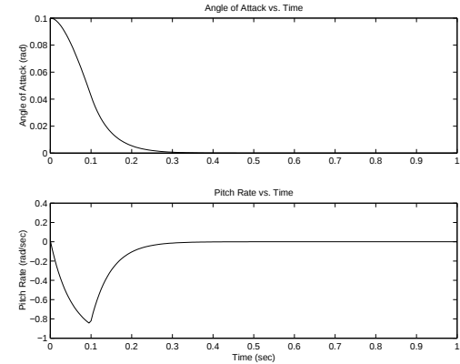
Figure 6 State Responses for Feedback Linearization with Sliding Mode Design
