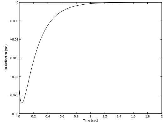
Figure 13 Fin Deflection with Back-Stepping Design
