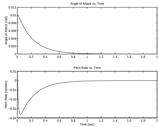
Figure 14 State Responses with Predictive Control Design
