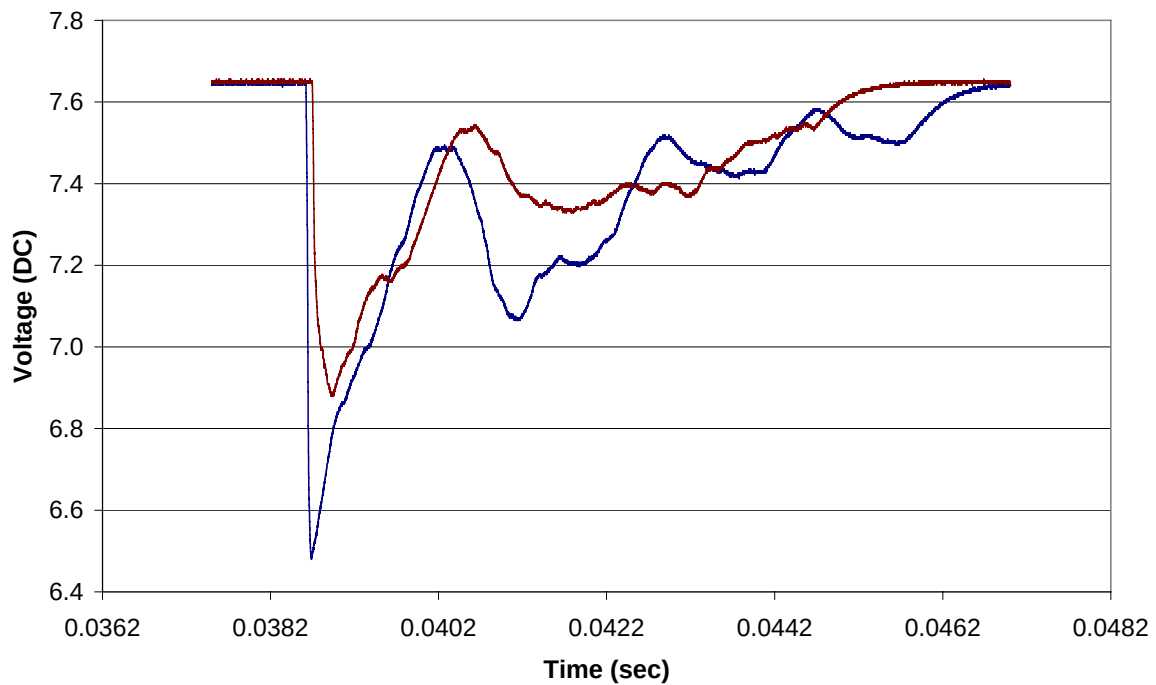
Figure E.11 Two ion probe traces when both sensors are 1.65 mm above the wall in the flow and 15 cm apart.
