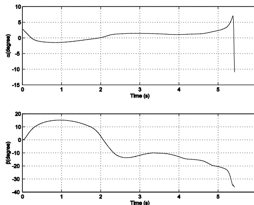
Figure 10. Missile Angles of Attack and Sideslip Time Histories
