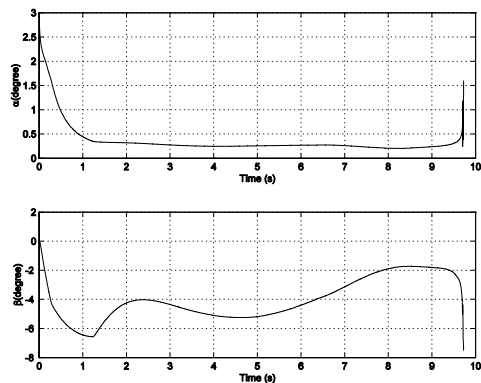
Figure 15. Missile Angles of Attack and Sideslip Time Histories
