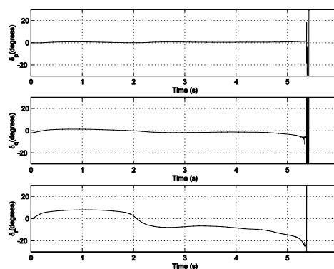
Figure 12. Time Histories of Fin Deflections
