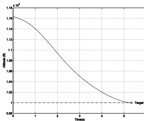
Figure 19. Missile and Target Altitude Time Histories, Solid Line: Missile, Dashed Line: Target
