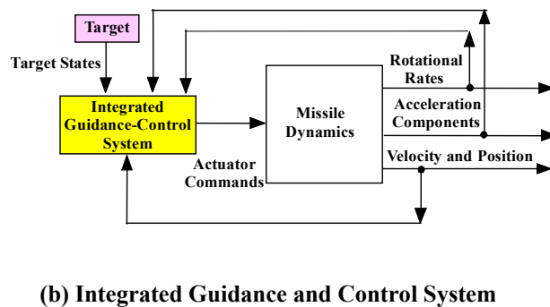
Figure 1. Conventional and Integrated Guidance-Control Systems.
