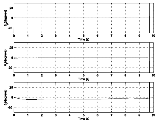
Figure 7. Time History of Fin Deflections
