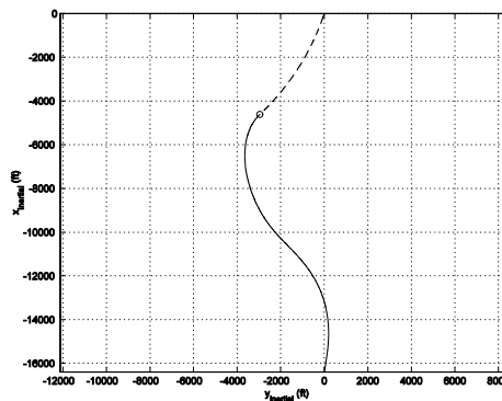
Figure 18. Horizontal Plane Trajectories of the Missile and the Target, Solid Line: Missile, Dashed Line: Target
