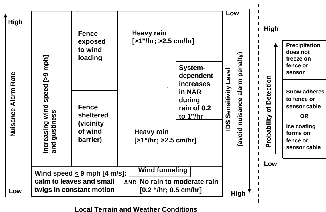
Figure B2. Weather and terrain influences on fence-mounted IDSs, showing (left) the tradeoff between IDS sensitivity setting and occurrence of environment-related nuisance alarms, and (right) the effect of frozen precipitation on probability of detection.
