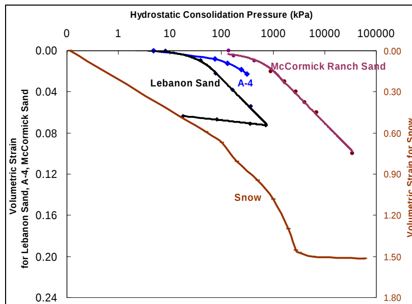
Figure 26. Pressure-volume relationship of Lebanon Sand compared with some other granular materials.
