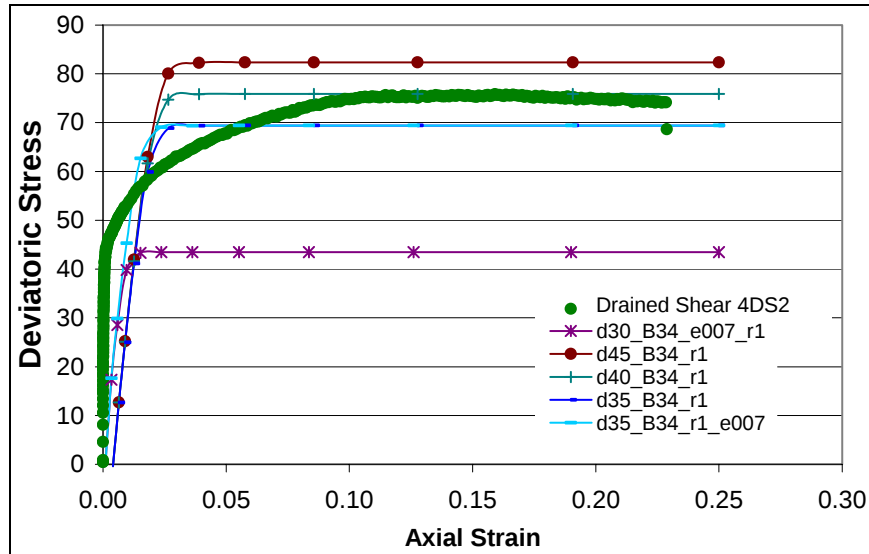
Figure E2. Comparison of changed initial volumetric plastic strain to laboratory data and unchanged volumetric plastic strains for 28 kPa (4 psi) confining pressure. There were no simulations performed for the change in initial volumetric plastic strain for 14 and 40 kPa (2 and 6 psi) confining pressures.
