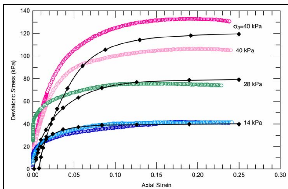
Figure 22. Comparison of final model parameters (Table 6) with laboratory data for 14, 28, and 40 kPa confining pressure.
