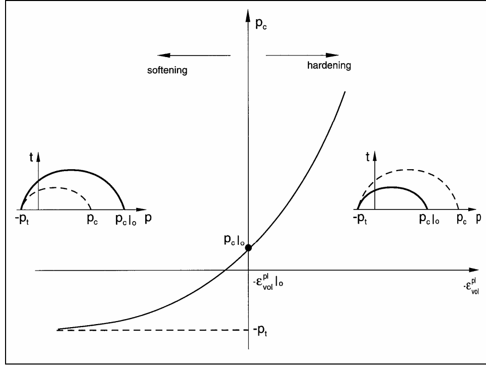
Figure 4. Cap contraction or expansion reflecting the softening (left) or hardening (right) of the material. (After HKS 2002.)
