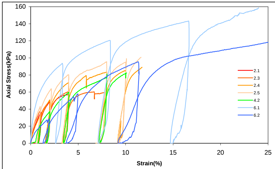
Figure 19. Triaxial, undrained shear data for samples representing specific thawing conditions of an average moisture content of 13% and a dry density of 1760 \text{ kg/m}^3 . Legend indicates test number from Table 4 and confining pressure in psi.
