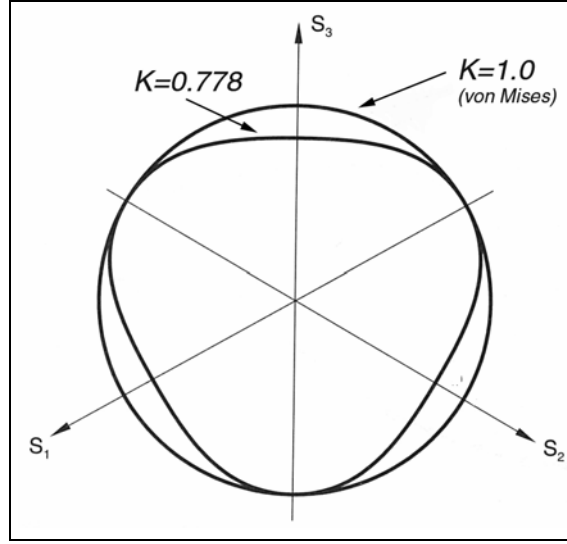
Figure 2. Modified Drucker-Prager yield surface in deviatoric space. (After HKS 2002.)
