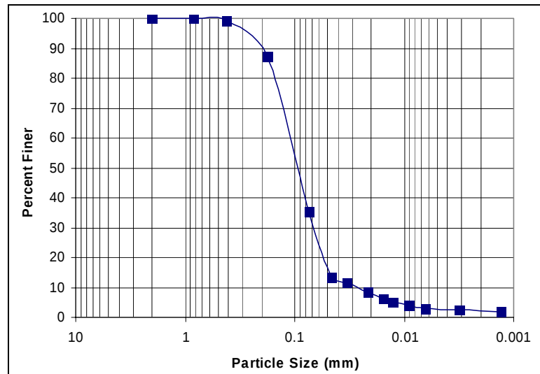
Figure 6. Lebanon Sand grain size analysis, with D_{10} = 0.027 , C_u = 4.579 .
