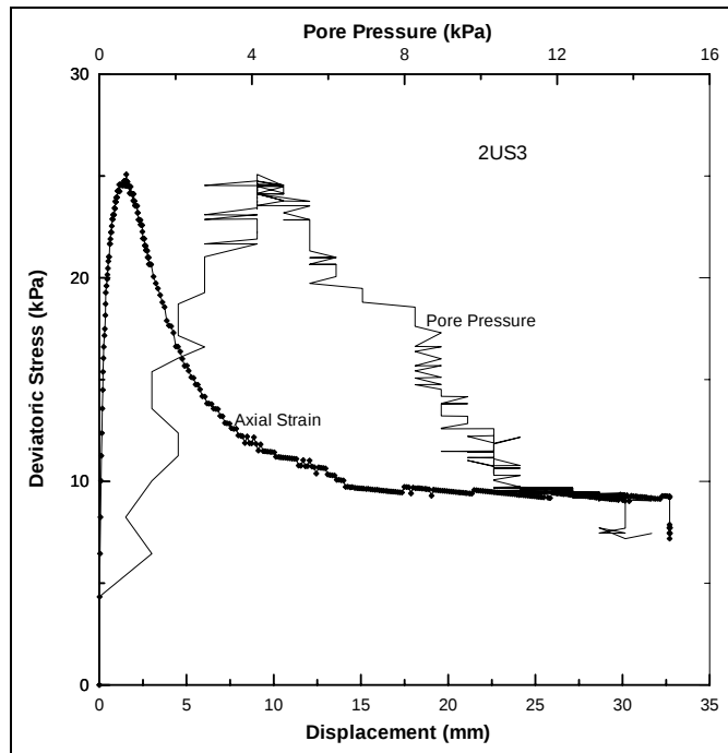
Figure B1. Deviatoric stress versus displacement and pore water pressures for the saturated undrained triaxial tests.
