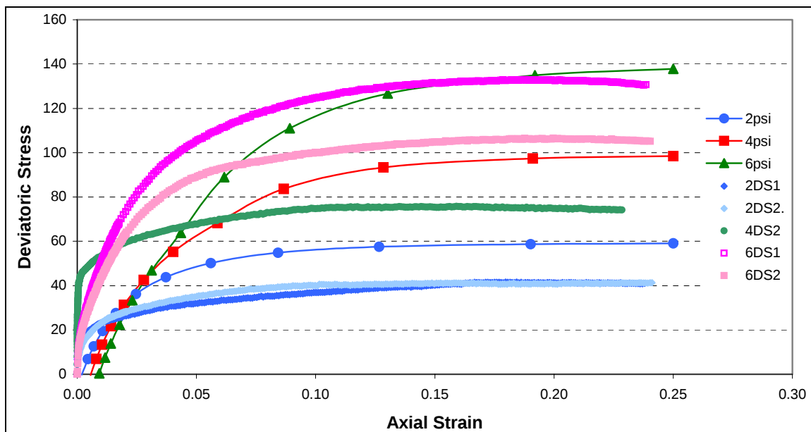
Figure E5. Comparison of final model parameters with laboratory data for 2, 4, and 6 psi confining pressure.
