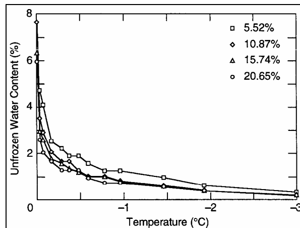
Figure A4. Warming data from unfrozen water content test on four samples tested with thawed gravimetric water contents.
