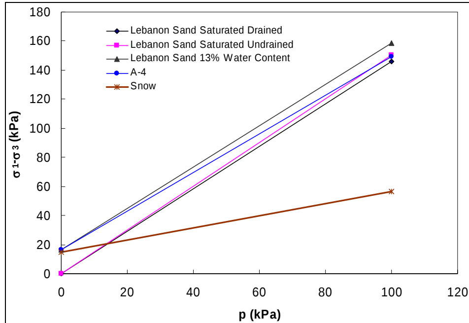
Figure 27. Drucker–Prager shear failure comparison of Lebanon Sand tested at different conditions, A-4 silt (saturated, drained), and snow.
