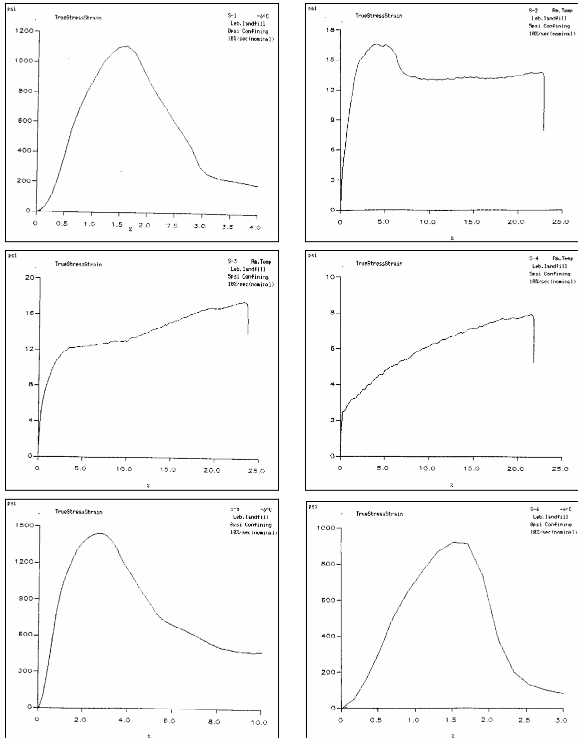
Figure A1. Stress-strain plots from the frozen cores.
