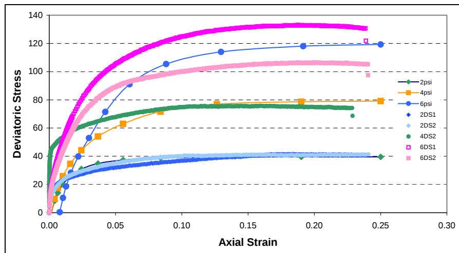
Figure E3. Comparison of new cohesion and beta graphs with laboratory data for 2, 4, and 6 psi confining pressure ( d = 1.0 \times 10^{-5} , \beta = 55.8^\circ , e_{vol} = 0 , e = 0.45 ).
