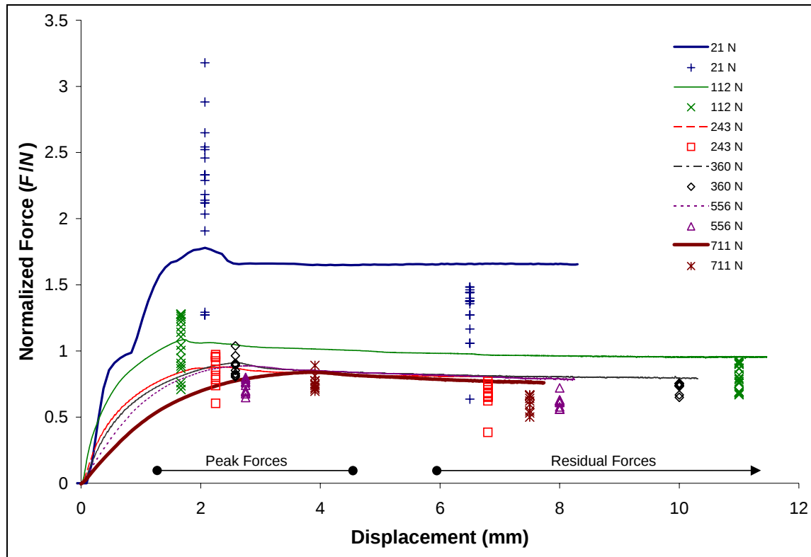
Figure 24. Comparison of finite element simulations of the direct shear test with laboratory data.
