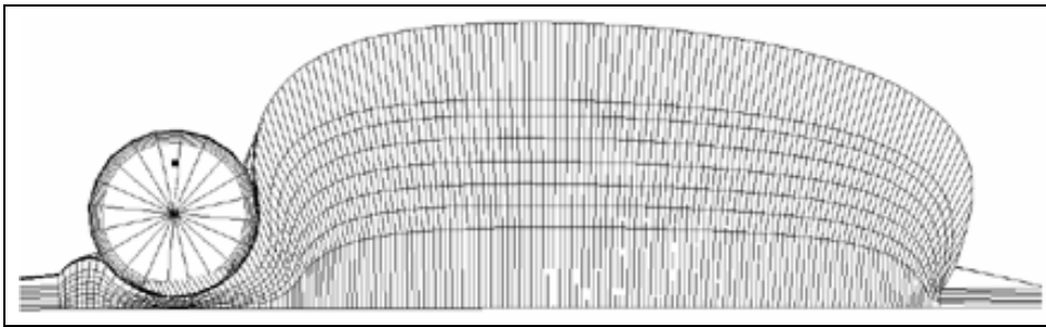
Figure E4. 3-D ABAQUS simulation of a tire in soft soil with large expansion caused by shearing of zero cohesion material (vertical exaggeration for illustration).
