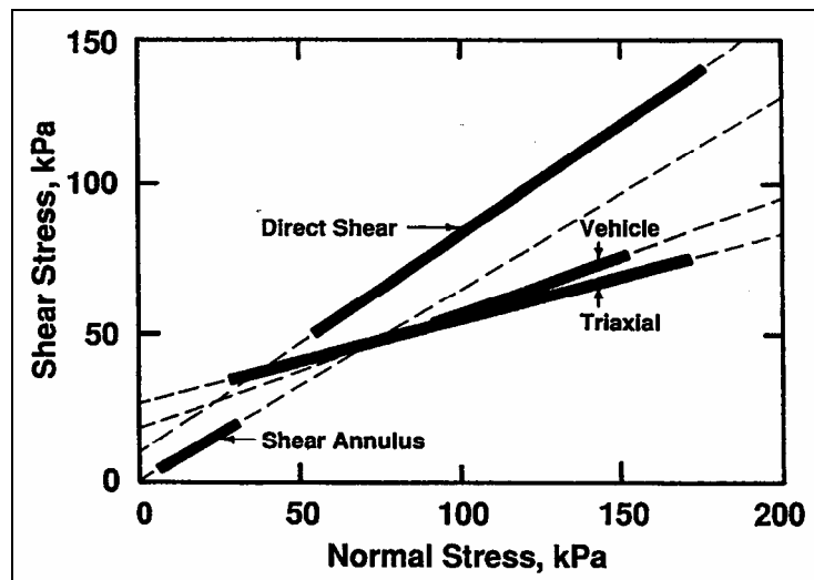
Figure A9. Comparison of failure envelopes for each test method. Solid lines mark the range of normal stress for each test.
