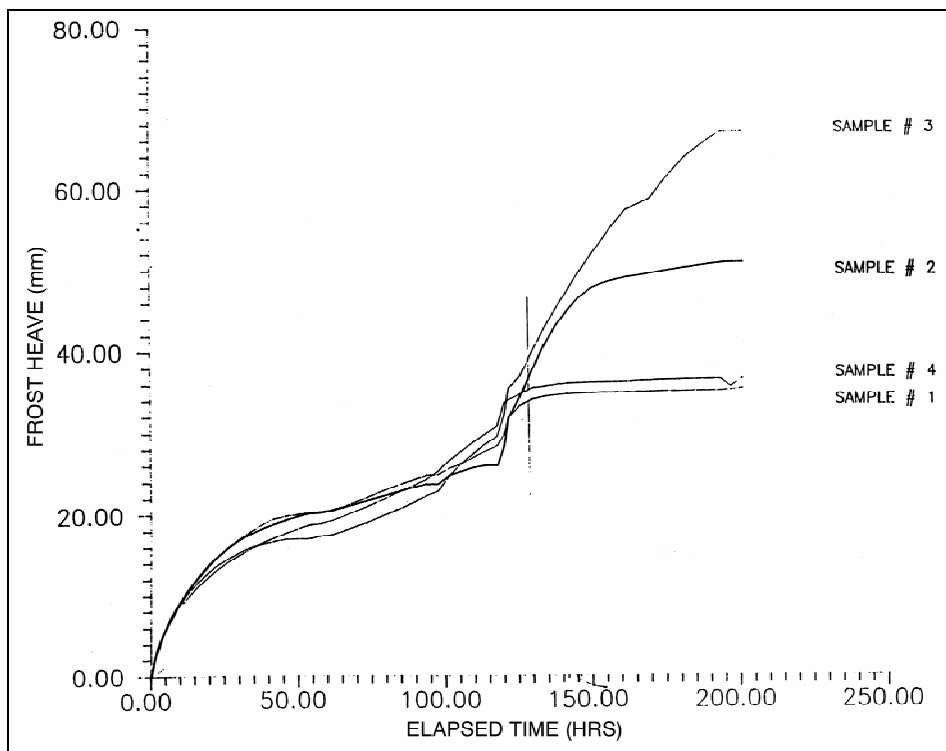
Figure A7. Frost heave test results.
