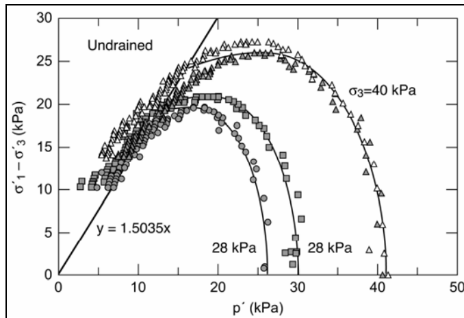
Figure 14. Stress paths for undrained shear tests, d = 0 , \beta = 56.4^\circ .
