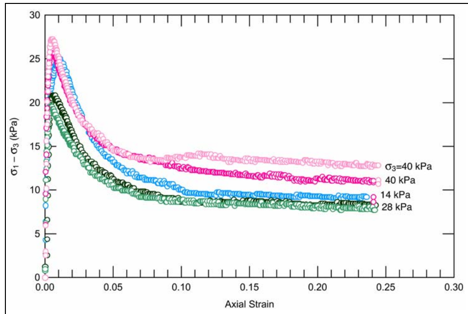
Figure 12. Consolidated, undrained triaxial tests.
