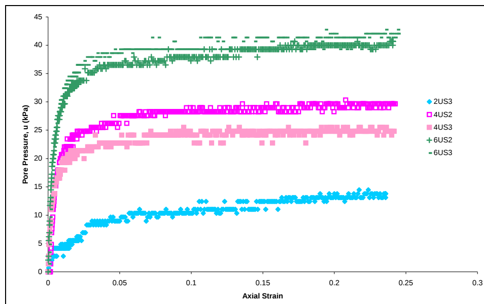
Figure 13. Undrained triaxial tests pore pressure measurements.
