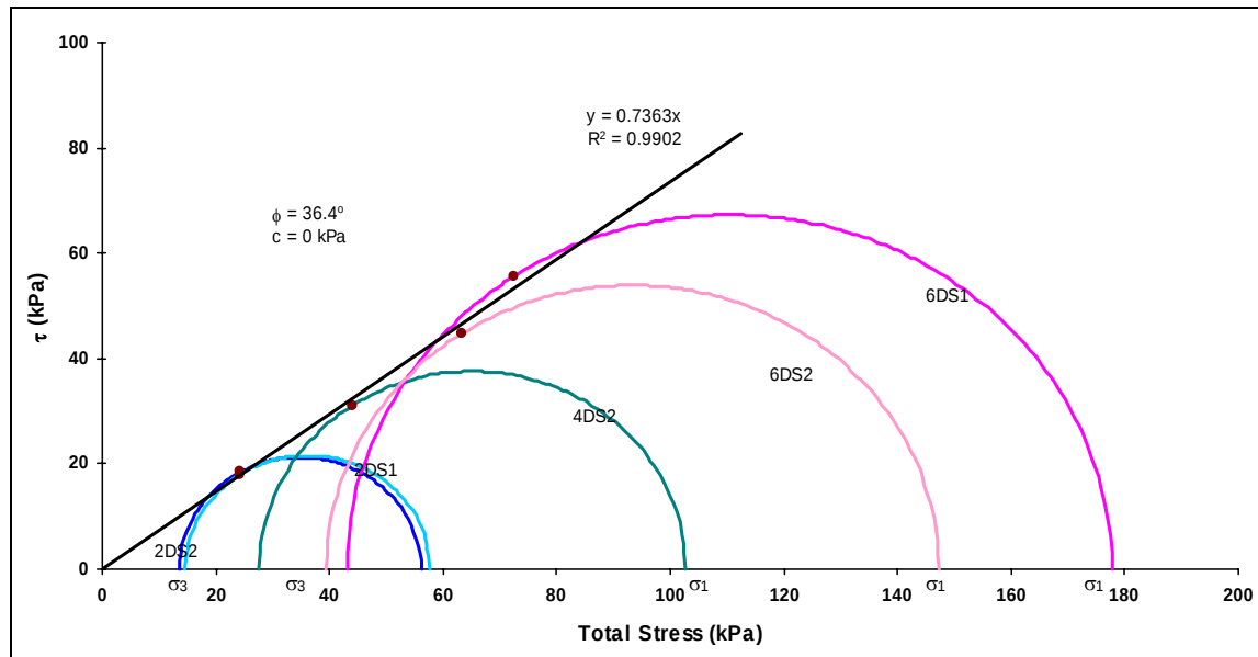
Figure 11. Mohr circle analysis for drained triaxial tests, c = 0 kPa, \phi = 36^\circ .
