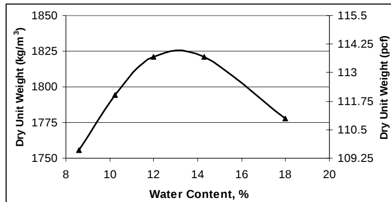
Figure 7. Compaction curve, with maximum density = 1826 \text{ kg/m}^3 ( 114 \text{ lb/ft}^3 ) and optimum moisture content = 13%.
