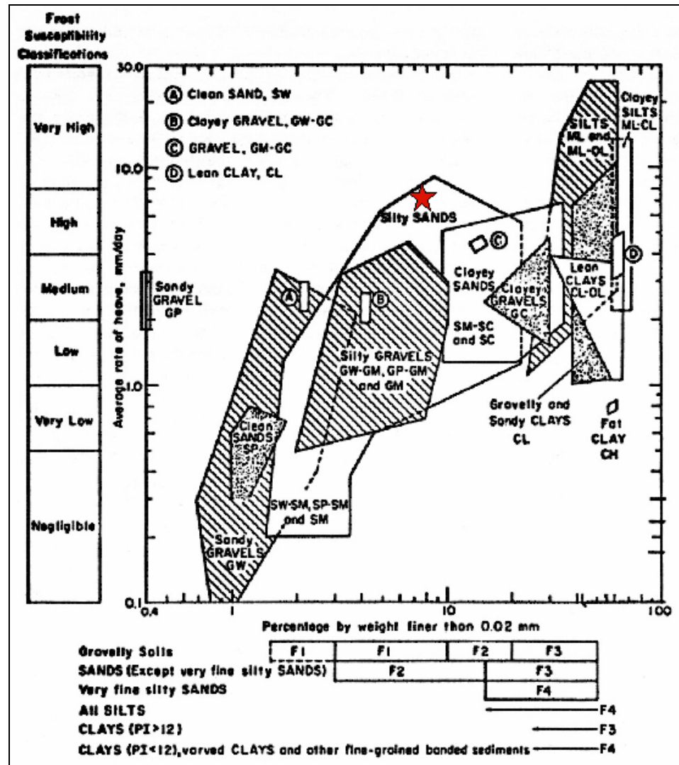
Figure A8. Lebanon Sand (red star) position on frost-susceptibility chart.
