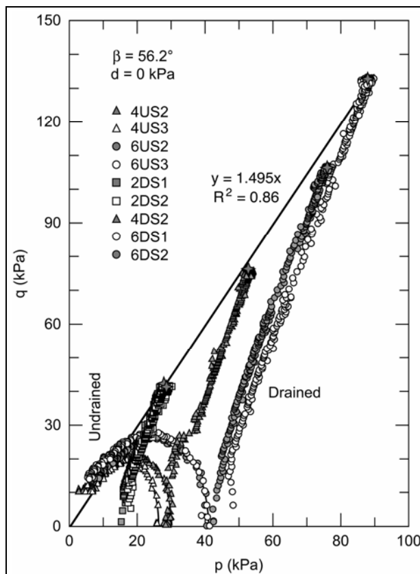
Figure 15. Test data for all of the saturated triaxial tests (drained and undrained).
