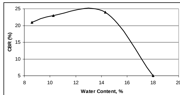
Figure 8. Soil strength from California Bearing Ratio (CBR) tests at various moisture contents.
