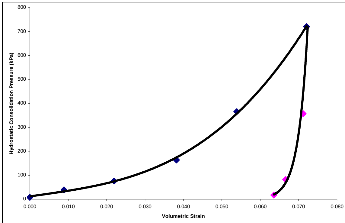
Figure 17. Hydrostatic compression vs. volumetric strain.
