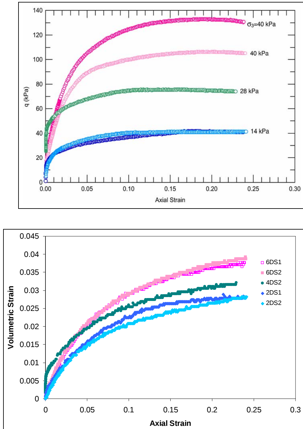
Figure 9. Drained triaxial tests.
