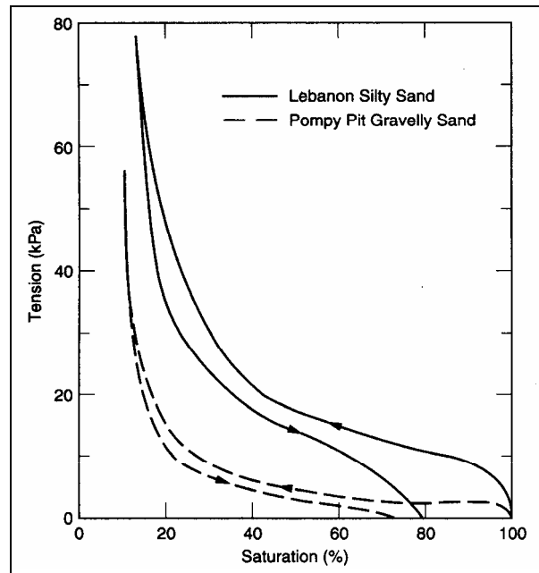
Figure A6. Laboratory moisture tension test.
