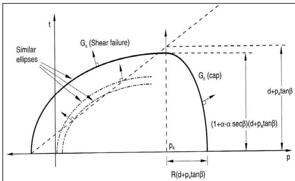
Figure 5. Modified CDP flow potential in the p - q plane. (After HKS 2002.)
