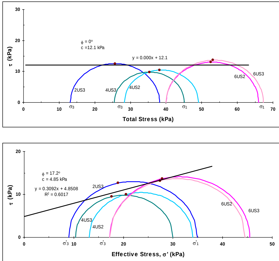
Figure 16. Mohr circle analysis for undrained triaxial tests; c = 12.1 kPa and \phi = 0^\circ for total stress (top), and c = 4.8 kPa and \phi = 17^\circ for effective stress (bottom).
