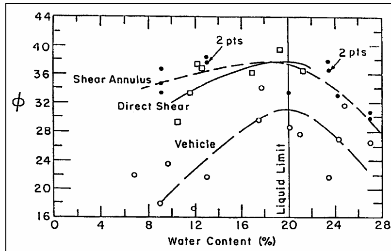
Figure A10. Calculated \phi' with water content.
