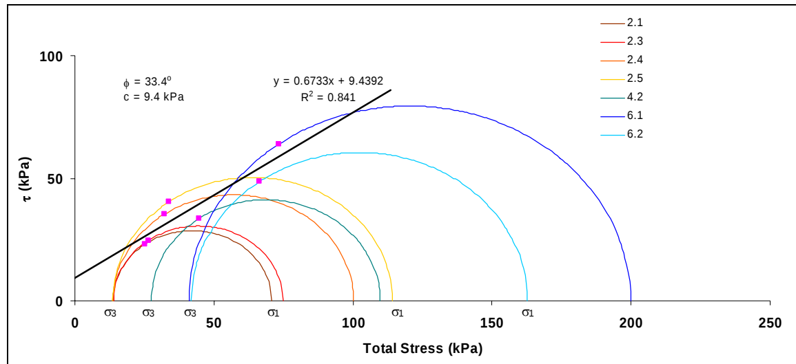
Figure 21. Mohr's circle analysis for samples at 13% moisture content; c = 9.4 kPa, \phi = 33^\circ .
