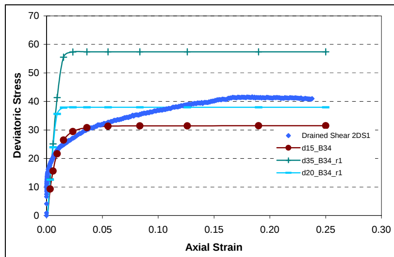
Figure E1. Comparison between results from simulation runs using higher cohesions (15, 20, and 35 kPa) with changed eccentricity (0.1) and laboratory data for 14 kPa (2 psi) confining pressure. The plots for the 28- and -40 kPa (4 and 6psi) confining pressures exhibited the same behavior as the 14-kPa plot.
