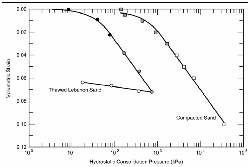
Figure 18. Pressure-volume relationship of Lebanon Sand compared to compacted sand.
