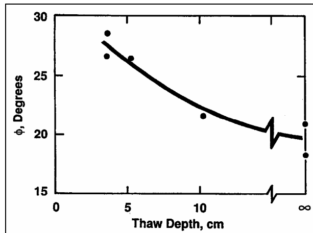
Figure A11. Calculated \phi' from the CIV test with thaw depth.
