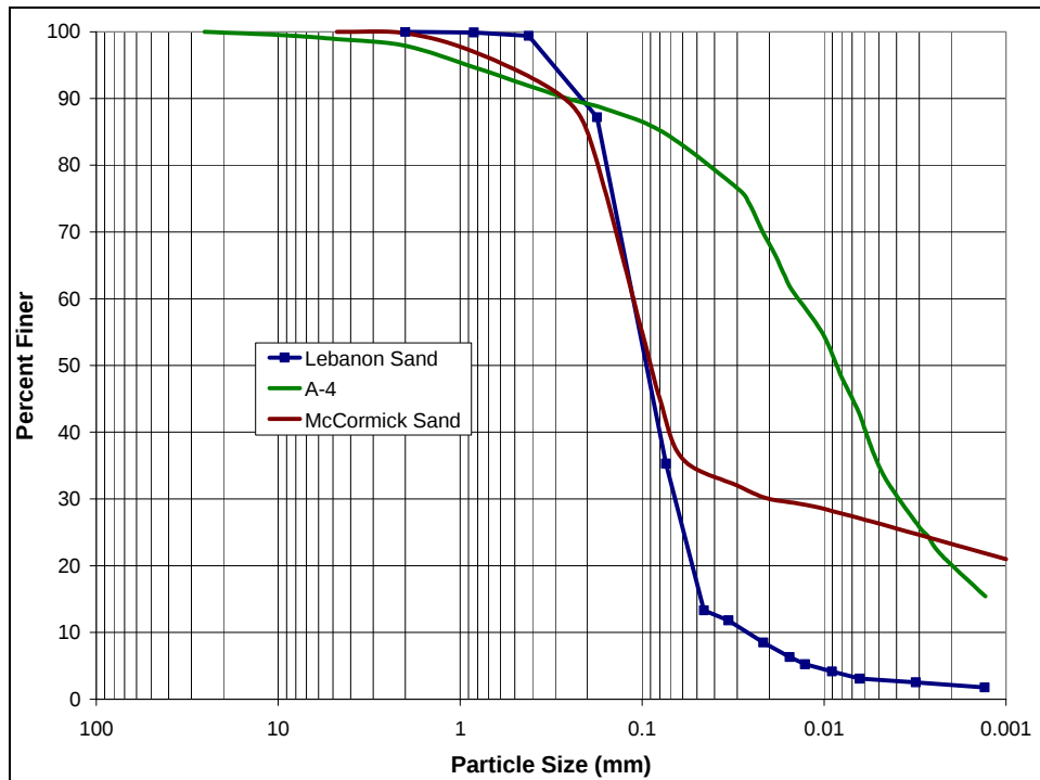
Figure 25. Lebanon Sand grain size analysis, D_{10} = 0.027 , C_u = 4.579 , compared with the McCormick Sand and A-4 silt.
