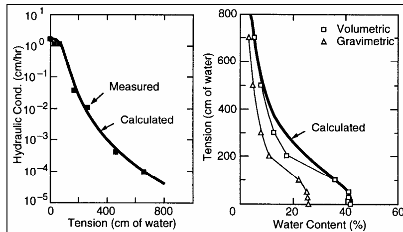
Figure A3. Hydraulic conductivity and moisture retention for Lebanon Sand.
