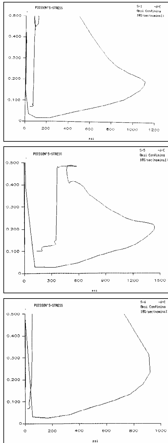
Figure A2. Poisson's ratio versus stress plots for S-1, S-5, and S-6 tests.
