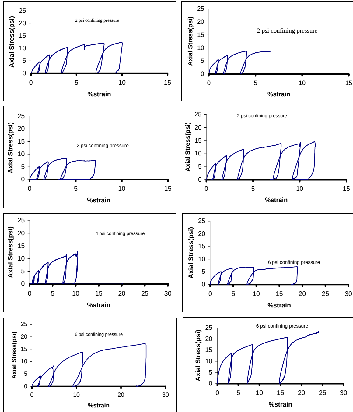
Figure C1. Unsaturated triaxial tests (undrained).
