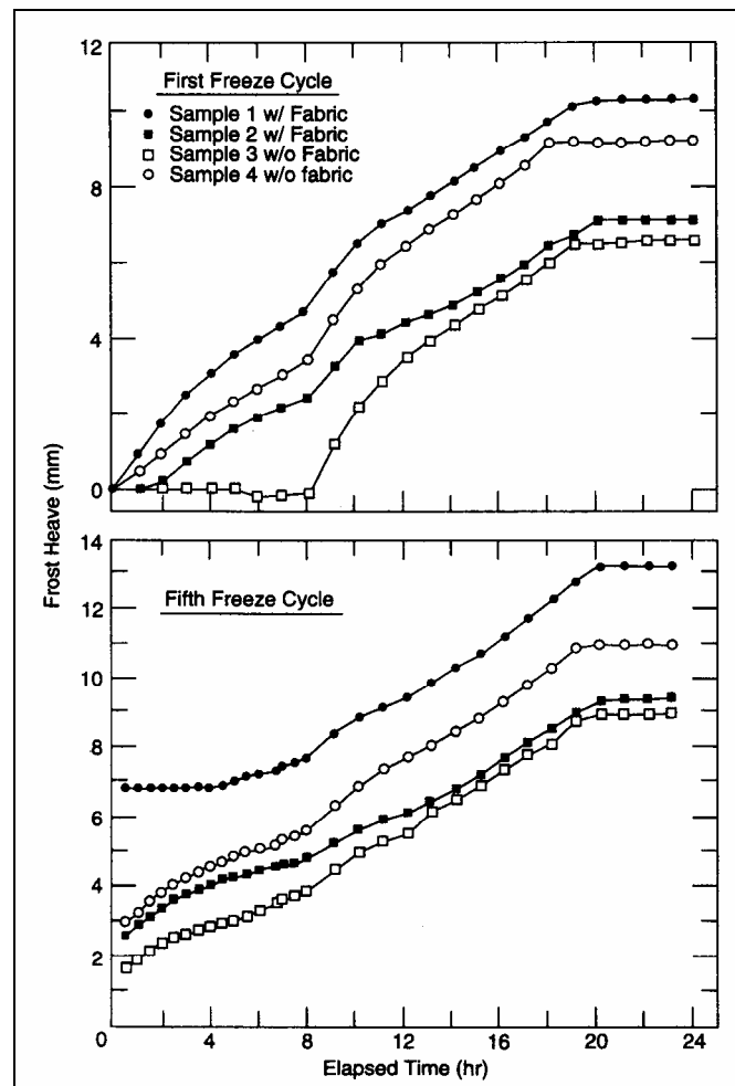
Figure A5. Laboratory frost heave test data.
