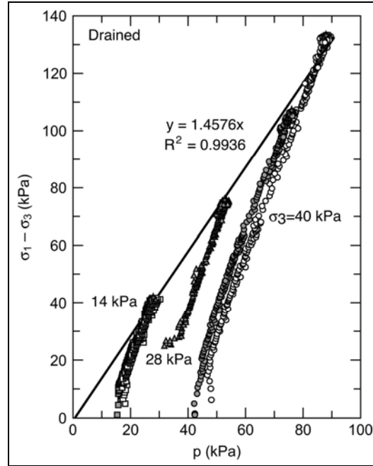
Figure 10. Shear failure line for Lebanon Sand drained shear tests, d = 0 , \beta = 55.6^\circ .
