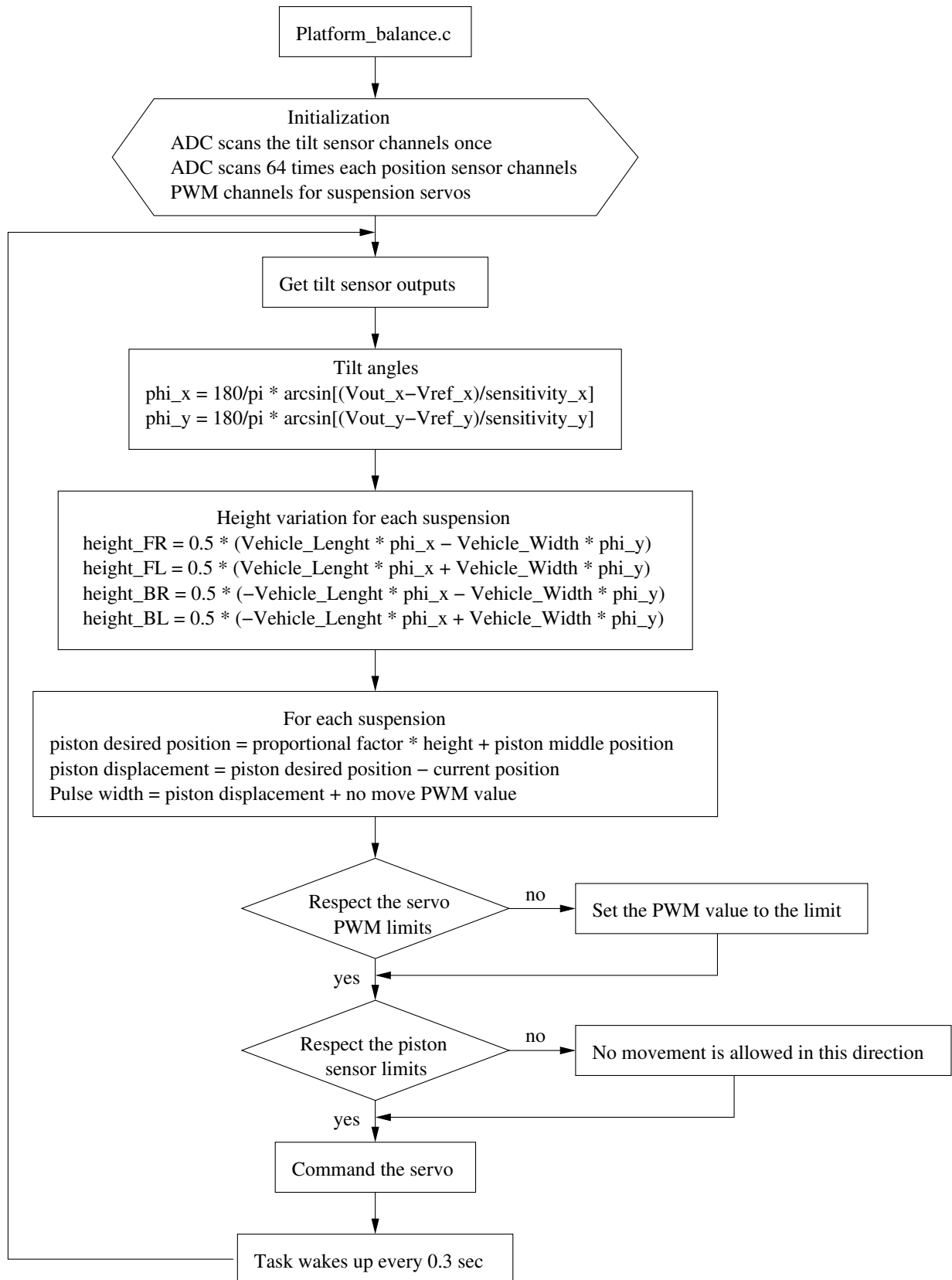
Figure 14: Platform balance diagram
