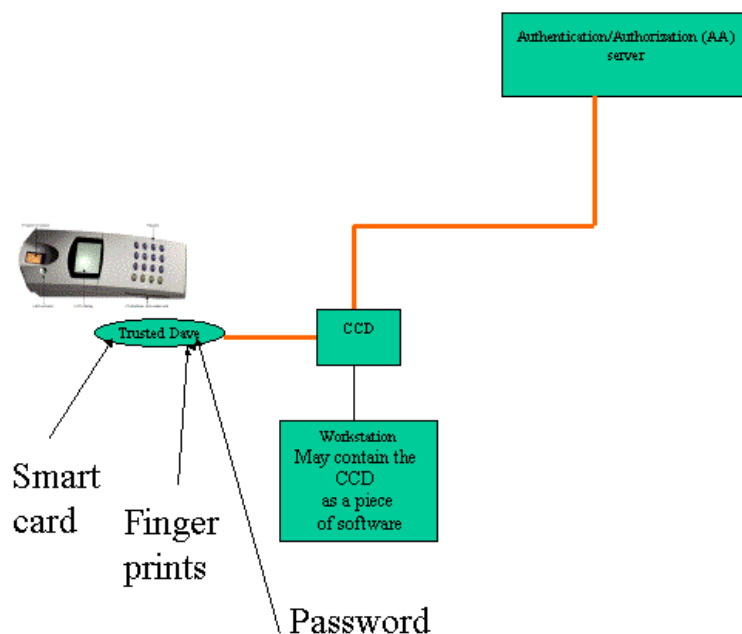
Figure 6- Basic System
