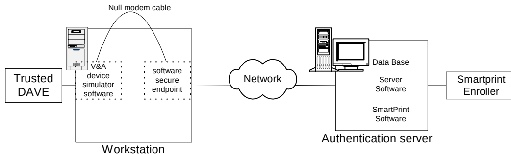
Figure 5-Functional Overview
