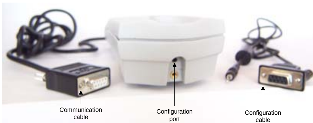
Figure 3 - V&A Device Communication and Configuration
