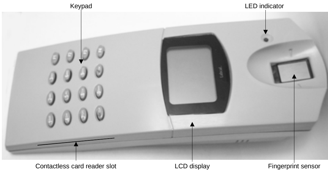
Figure 2-V&A device (Trusted DAVE)
