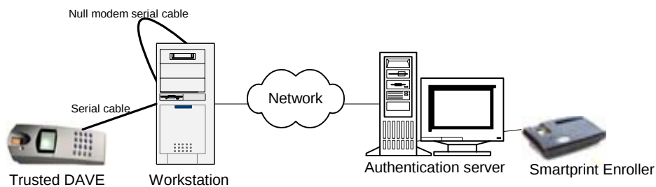
Figure 1-Demonstration System
