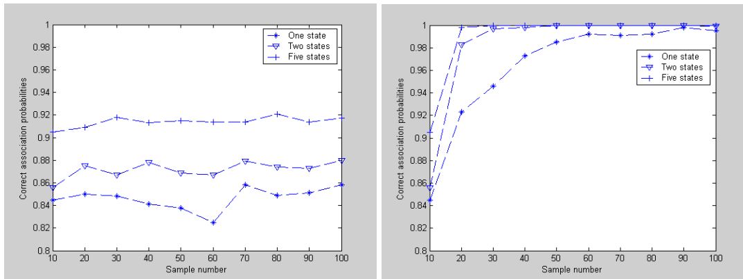
Figure 6. Correct association probability for the single target. The testing threshold is 2.05. (a) The variance in the testing variable changes with the sample number; (b) The variance in the testing variable is fixed.
