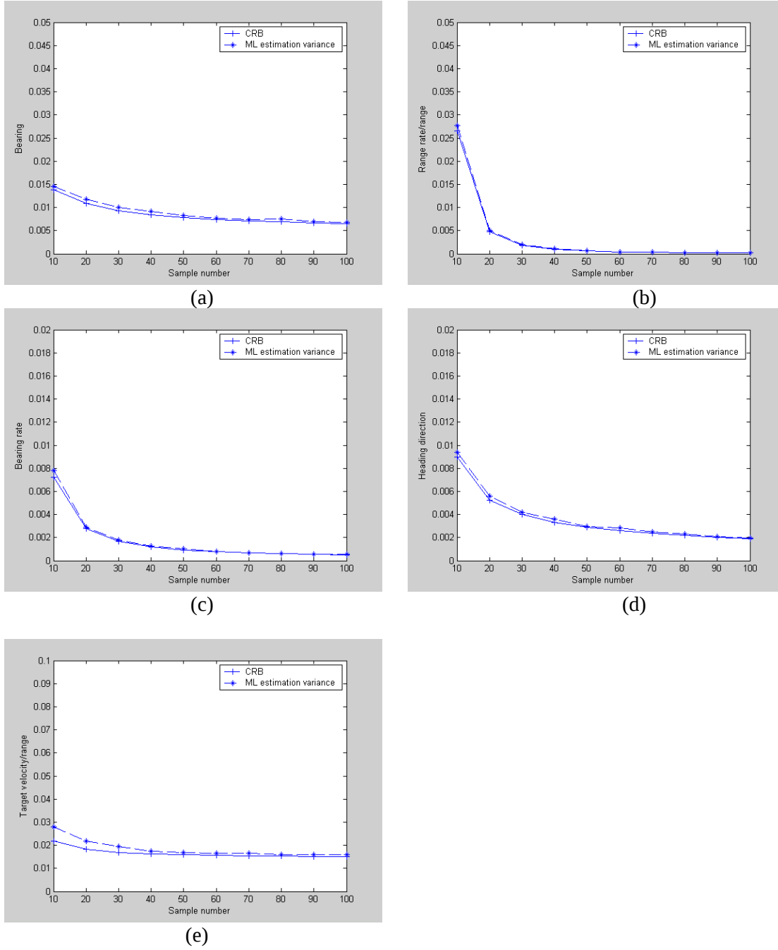
Figure 4. Comparison of the ML estimator and CRB for ESM tracking: (a) bearing; (b) range rate/range; (c) bearing rate; (d) heading direction; (e) target velocity/range.
