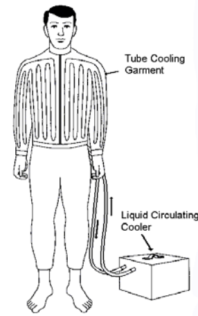
Figure 5. Liquid Circulating Microclimate Cooling System
