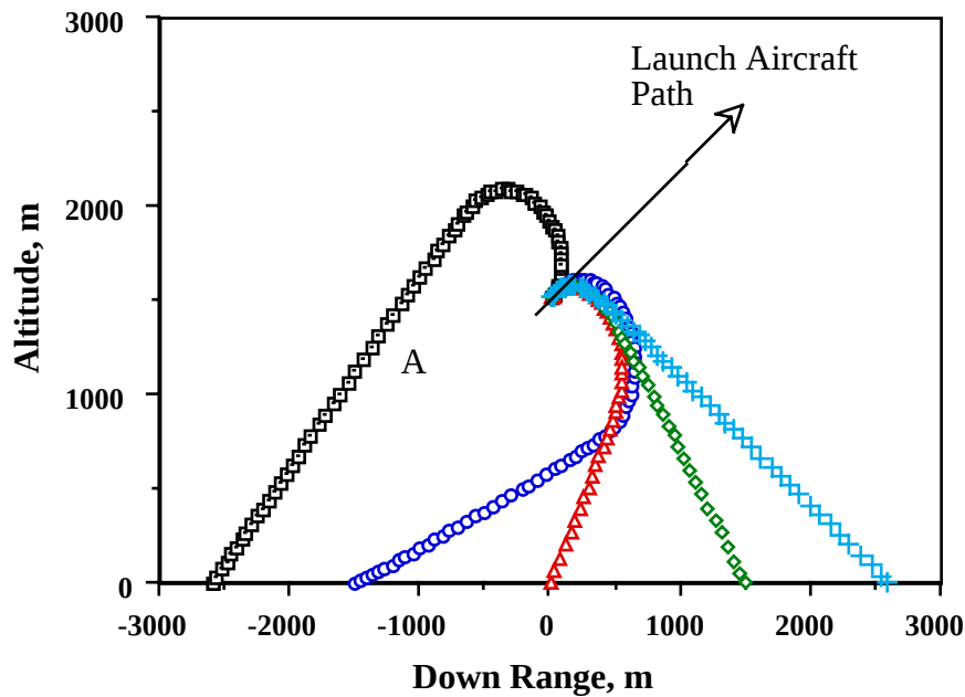
Fig. 4. A Family of Trajectories for the Air-to-Surface Mission
