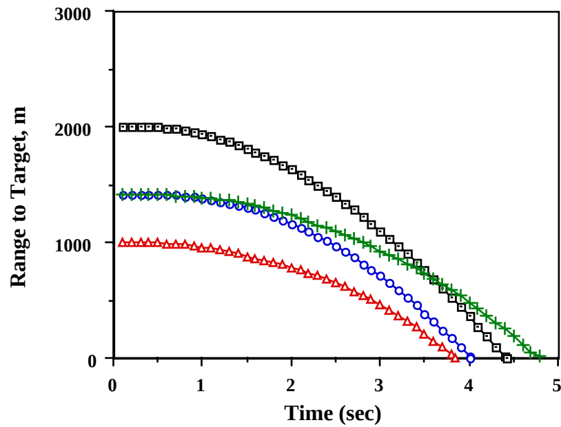
Fig. 5.21. Range-to-Target as a Function of Time for the Air-to-Air Missile Trajectories given in Figure 5.18.
