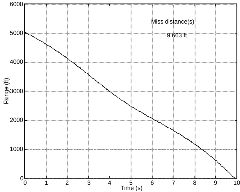
Fig. 9. Range to the Target using the Fuzzy Proportional Navigation Guidance Law
