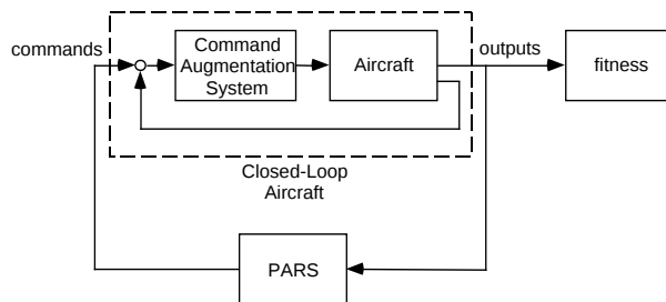
Figure 1. Closed-Loop System
