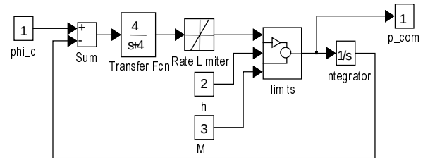
Figure 3. Roll Rate Command Generator
