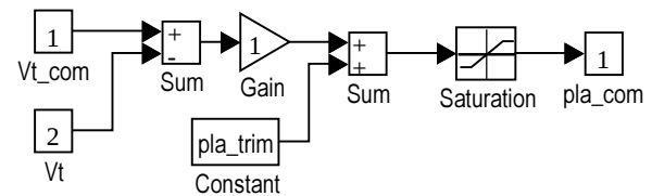
Figure 5. Velocity Controller
