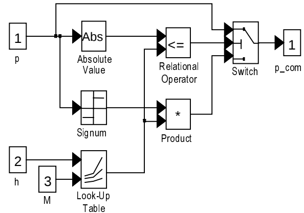
Figure 4. Limit Block
