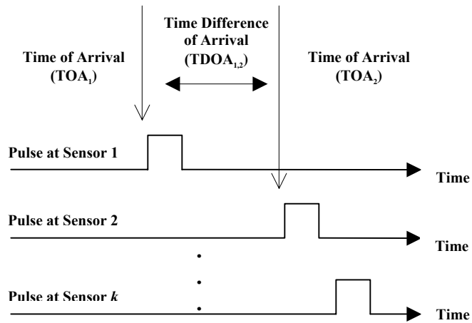
Figure 2. Time of arrivals (TOA) and time differences of arrival (TDOA)
