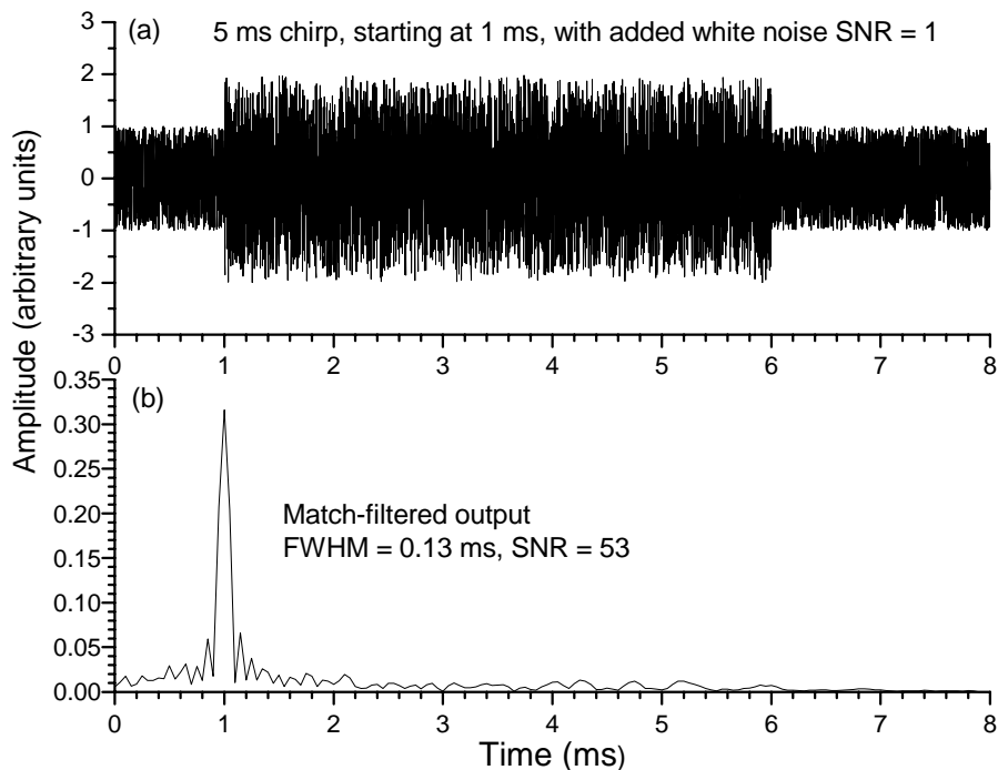
Figure 19 Results of synthetic chirp pulse analysis: (a) simulating a 5-ms x 10-kHz chirp pulse with 1-ms delay and added white noise of equal amplitude, (b) match-filtered output showing time compression to 0.13 ms pulse with processing gain of 53 (17.2 dB).
