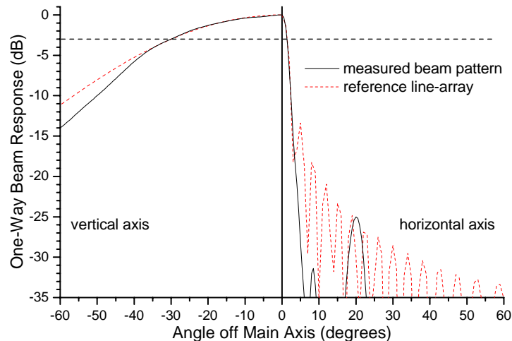
Figure 1: 100kHz EDO Western model 6400 sidescan beam pattern, compared to reference patterns calculated using line-array model with array length chosen to match measurement a -3dB level.
