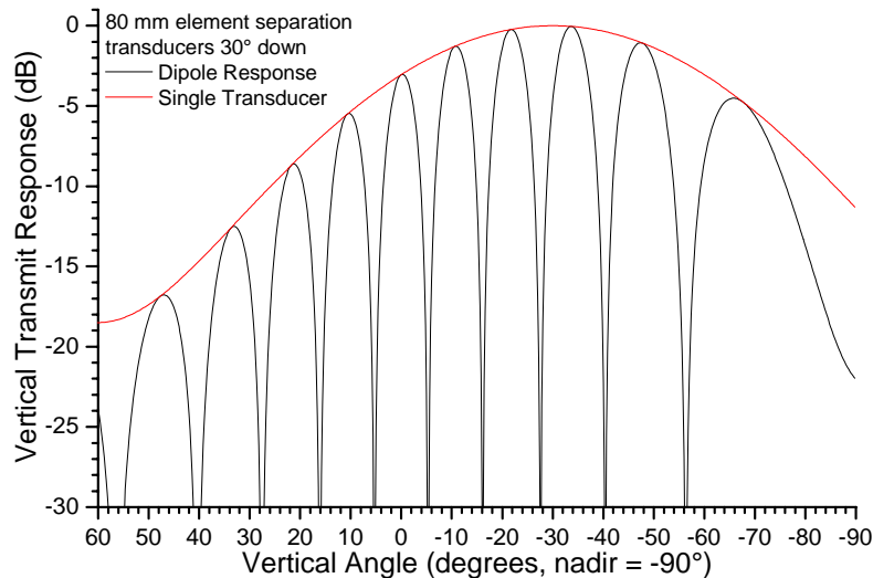
Figure 15: Comparison of single and dipole vertical transmit response. Assumes transducer vertical separation of 80 mm and 30° depression angle.
