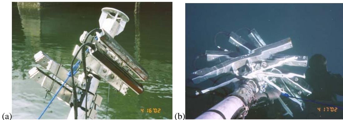
Figure 2: photographs of 4 \times 100\text{kHz} transducer mounting on RV Tayut . (a) interferometric dipoles used on April 16 th ; photo with pole swung upwards and out of water (b) looking down into the water at multi-azimuth configuration used on April 17 th (left is forward).
