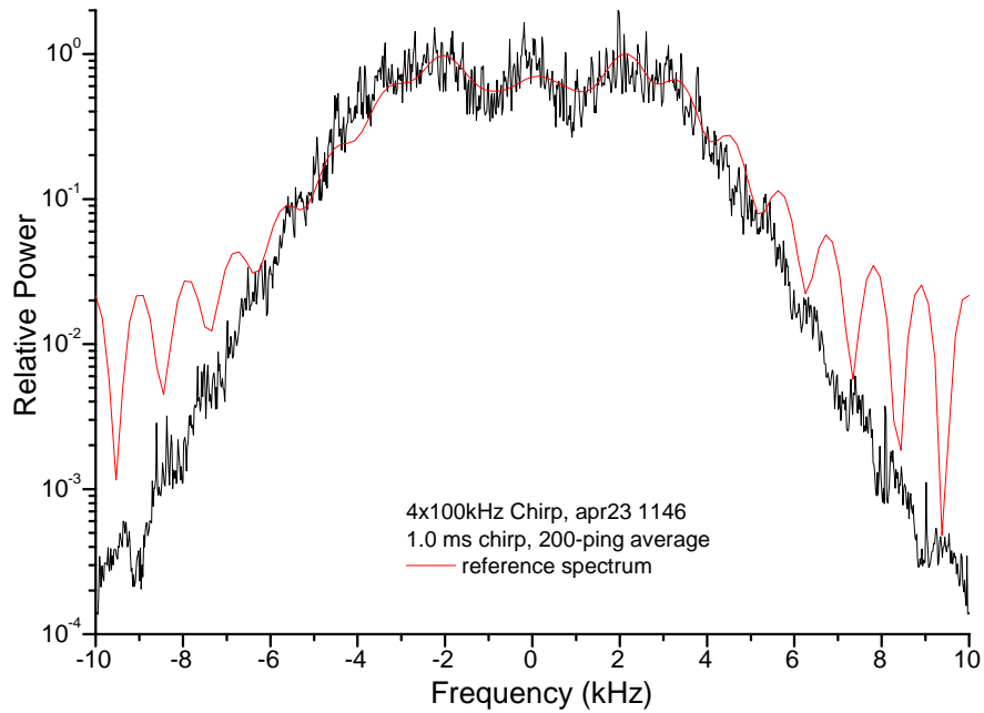
Figure 21 Comparison of measured and reference frequency spectra for 1.0 ms chirp pulse. Data averaged over 200 x 8192-pt FFT taken at IOS pier at 1146h April 23 rd , 2002. Reference pulse replica was synthesized using 20 frequency steps of 500 Hz from 95 to 105 kHz, coherently homodyned.
