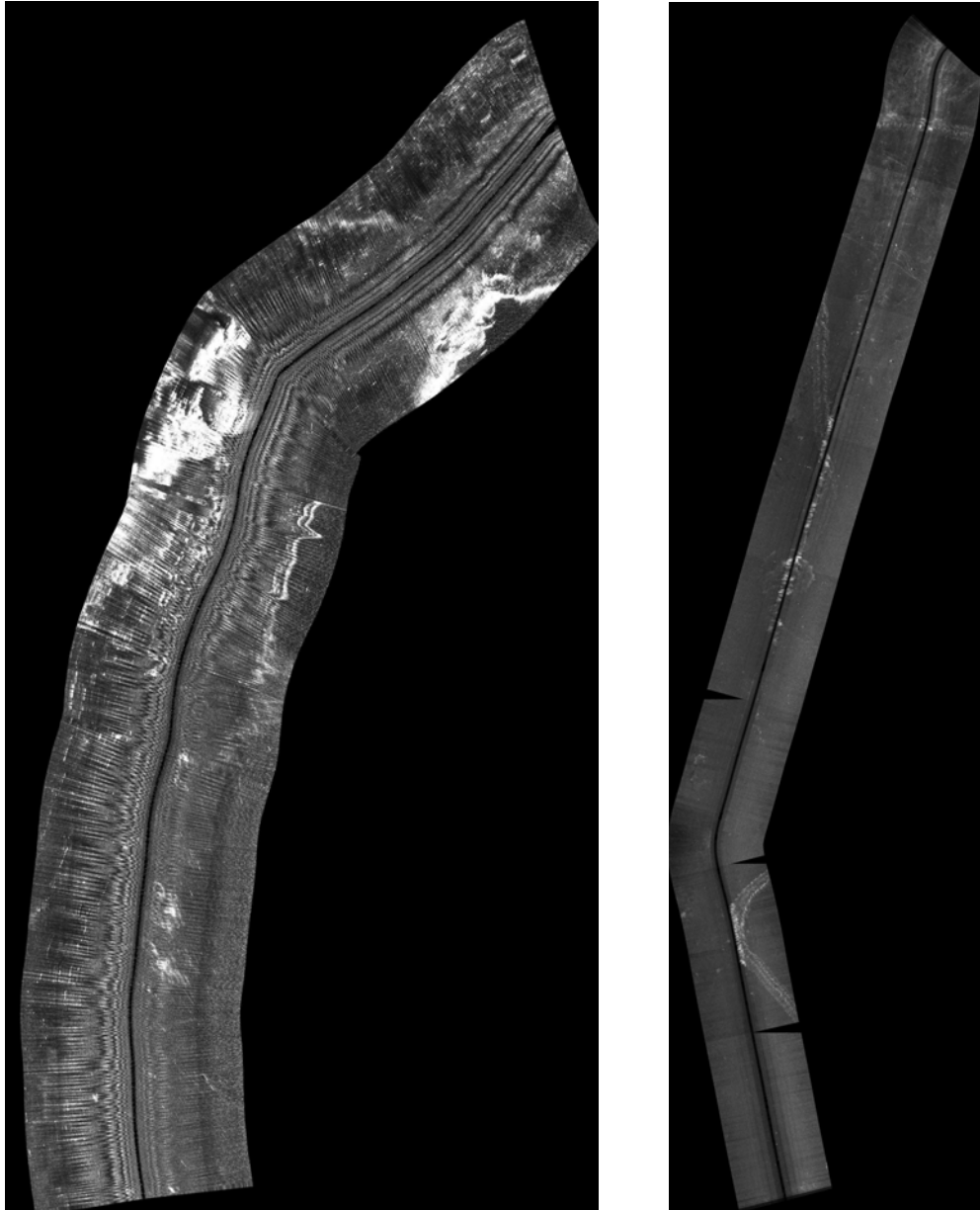
Figure 10: Comparison of sidescan mosaics near the mouth of Esquimalt Harbour using the 100-kHz sonar (left) and Klein 5500 sonar (right). 100-kHz swath width was 185 m per side, while the Klein sidescan swath width was 75 m per side.
