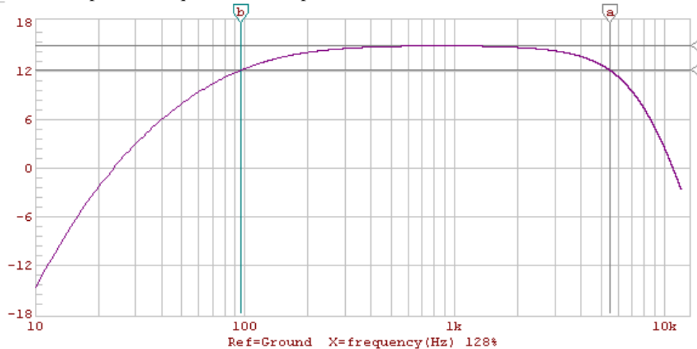
Figure 6: frequency response of typical receiver channel after mix-down and low-pass filtering.
