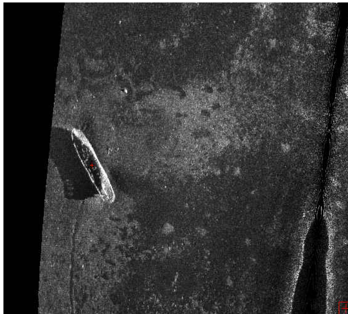
Figure 14 Klein 5500 sidescan geo-coded image of the 65-m deep ship-wreck SSE of Esquimalt, B.C., from April 2002 surveys. Wreck located at N48^\circ 23.094' , W123^\circ 25.584' , and is 30 m long by 5.5 m wide. This is the same ship-wreck as in Fig. 13.
