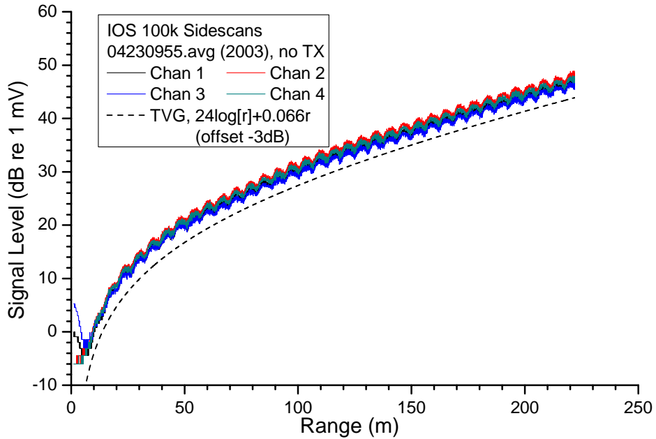
Figure 7 Signal intensity vs. range for TVG test, averaged over 100 pings taken 0955h, Apr. 23, 2003 at IOS. TVG control parameters were t_0 = 2 ms, t_1 = 300 ms, and G_0 = -20 dB, with a 0.4 ms pulse length. Transmit power was disabled. Best-fit TVG curve offset by -3 dB for clarity.
