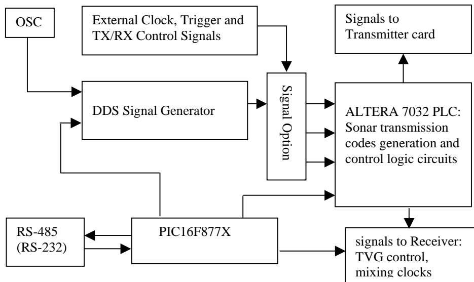
Figure 3: block diagram of the sonar Controller card.
