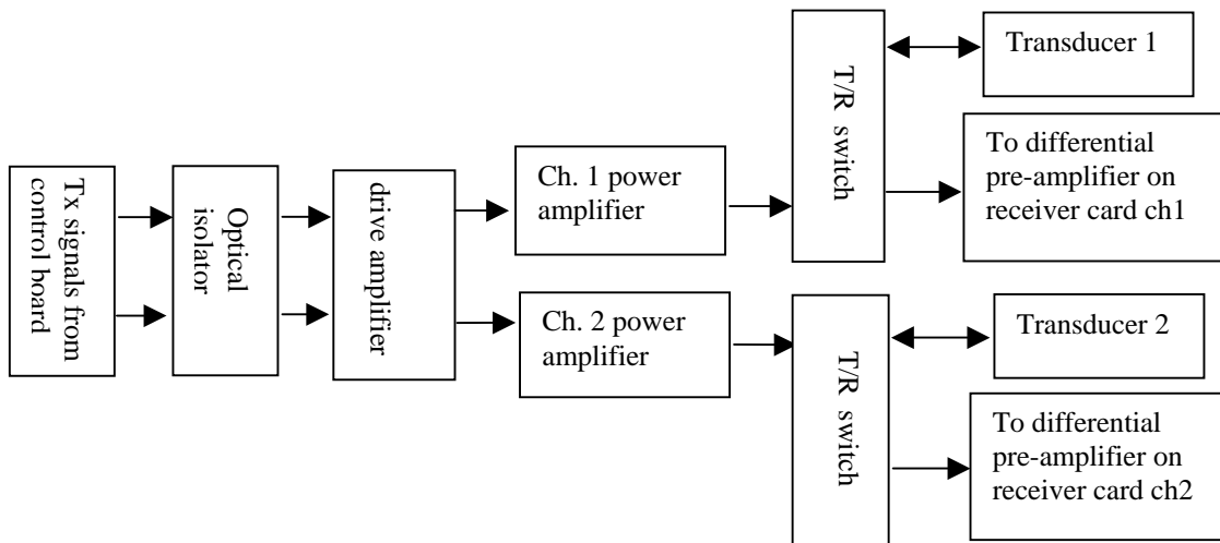
Figure 5: block diagram for two channels on the sonar Transmitter card.
