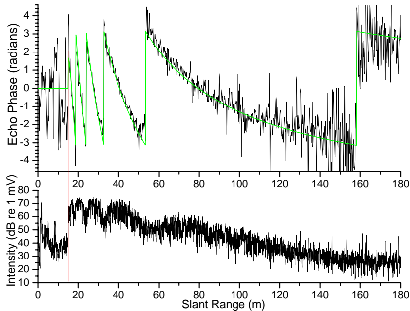
Figure 17 Single-ping phase and intensity vs. slant range for the 100-kHz port-side interferometric dipole, taken at 1401h, April 16 th , 2002 near the entrance to Esquimalt harbour. Red line is range to seabed. Green line is reference phase computed assuming flat seabed at 15 m depth.
