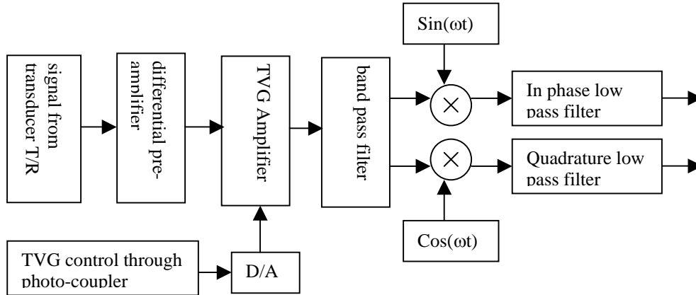
Figure 4: Block diagram for one channel on Receiver card (two channels per board); output to A/D card on data acquisition PC.
