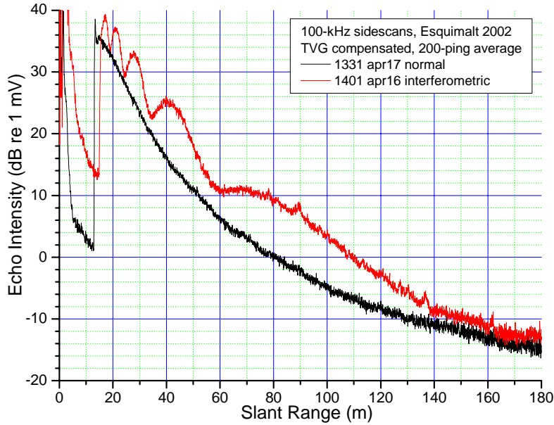
Figure 16 Comparison of normal (single-channel) and interferometric sidescan intensity vs. range curves, taken in April 2002 surveys near the entrance of Esquimalt harbour.
