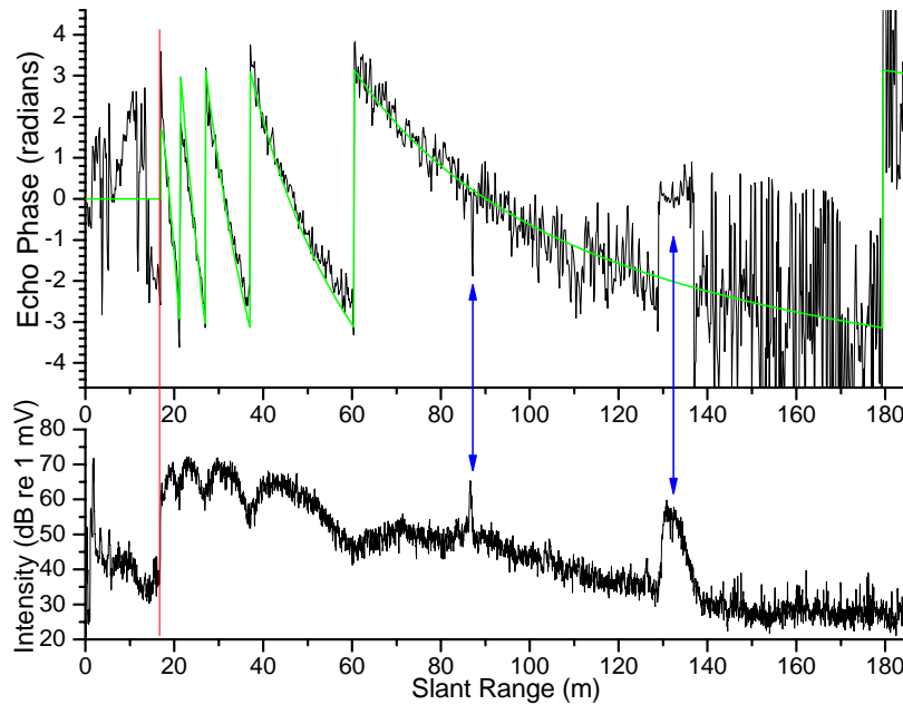
Figure 18 Single-ping phase and intensity vs. slant range for the 100-kHz port-side interferometric dipole, taken at 1350h, April 16 th , 2002 near the entrance to Esquimalt harbour. Red line is range to seabed. Green line is flat seabed reference phase. Blue arrows denote intensity-phase anomalies.
