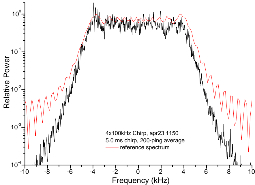
Figure 20 Comparison of measured and reference frequency spectra for 5.0 ms chirp pulse. Data averaged over 200 pings taken at IOS pier at 1150h April 23 rd , 2002. Reference pulse replica was synthesized using 100 frequency steps of 100 Hz from 95 to 105 kHz, coherently homodyned.
