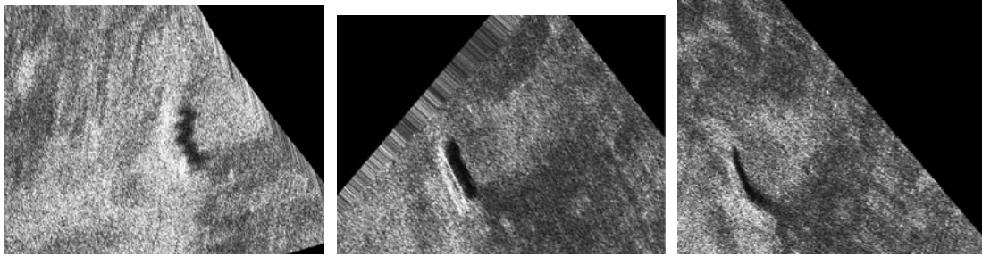
Figure 13 Multiple 100-kHz sidescan geo-coded views of 65-m deep ship-wreck SSE of Esquimalt, B.C. taken at 1102h, April 17 th , 2002: (left) Chan. 2 oriented 39^\circ aft of beam, (middle) Chan. 3 oriented 4^\circ aft of beam, and (right) Chan. 4 oriented 18^\circ forward of beam.
