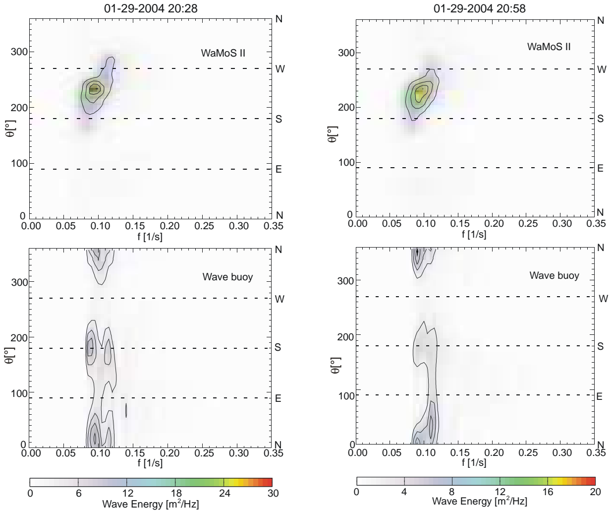
Fig. 13c: Directional spectra E(f, \theta) of WaMoS II and wave buoy on January 29, 2004, 20:28.
