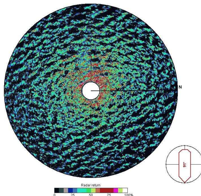
Fig. 4: Nautical radar image as obtained by WaMoS II onboard CFAV Quest, January 30, 2004, 18:59 . The colour coding corresponds to the radar back scatter strength where black indicates no return and white maximum return. The ship course is indicated by the ship bow arrow (bottom right).
