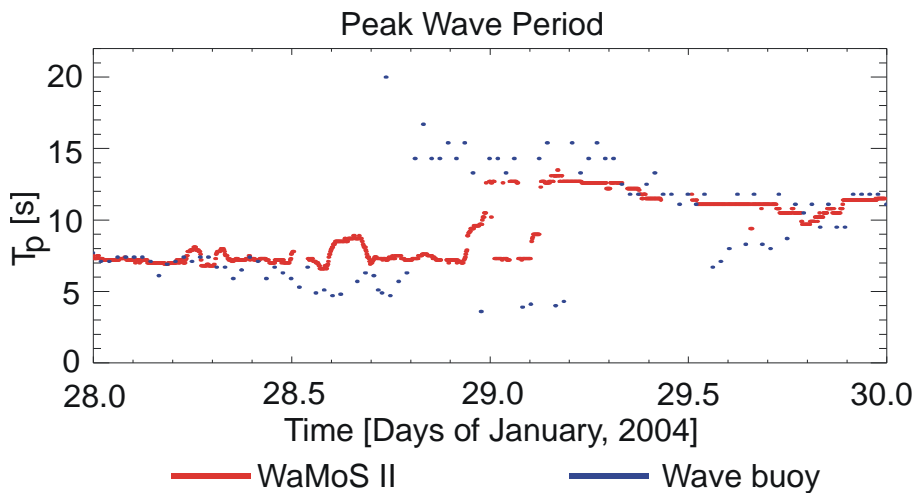
Fig. 8: Section B of the peak wave period as measured onboard CFAV Quest from January 28 to 30, by WaMoS II and the wave buoy
