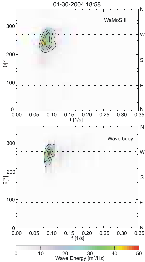
Fig. 16: Directional spectra E(f, \theta) of WaMoS II and wave buoy on January 30, 2004, 18:58 .
