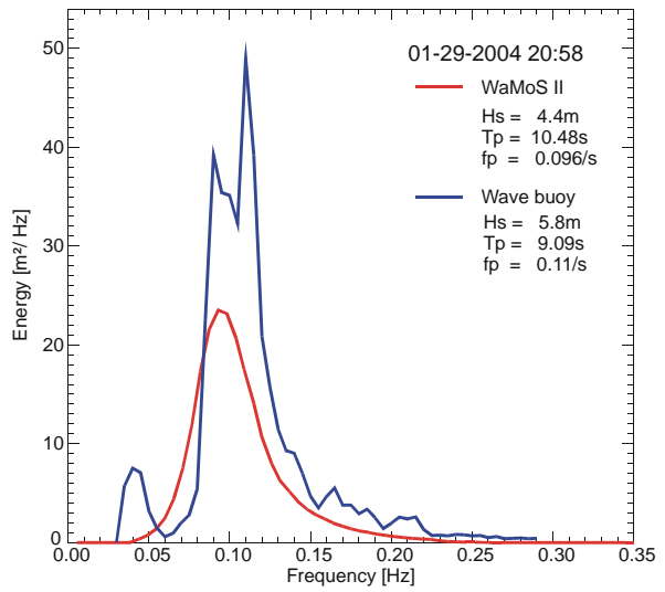
Fig. 11d: Frequency spectra S(f) of WaMoS II and the wave buoy on January 29, 2004, 20:58.
