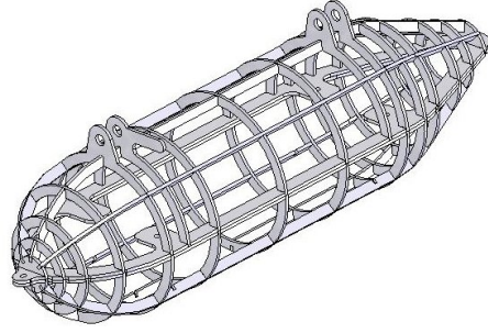
Figure 4: The modular design of the Pod allows for fast production time using CNC machines and for easy assembly.
