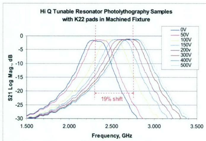
Figure 20. S_{21} parameters with applied voltage in the range of 0 to 500 Volts.
