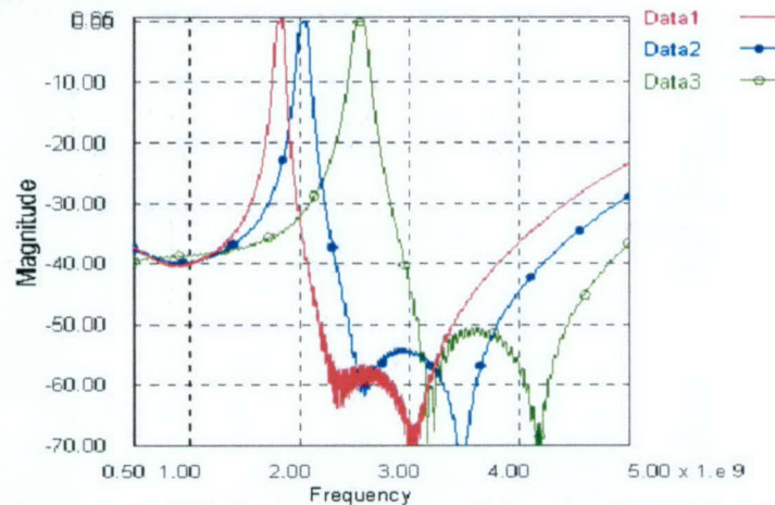
Figure 17. Frequency shift for S_{21} with four dielectric plates (Data1: \epsilon_r=50 , Data2: \epsilon_r=20 , Data3: none).
