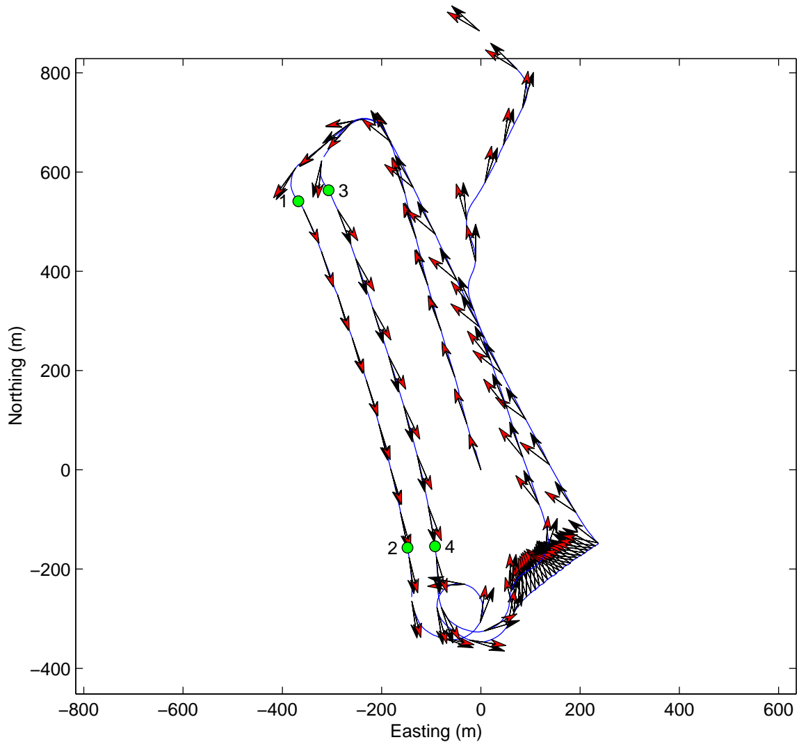
Figure 2: Plan view of vehicle track associated with the time series shown in the previous Figure with instantaneous heading indicated by the arrows: red arrows are Octans and black are “compass”. The labelled green dots correspond to the numbered vertical dashed lines in the previous Figure.
