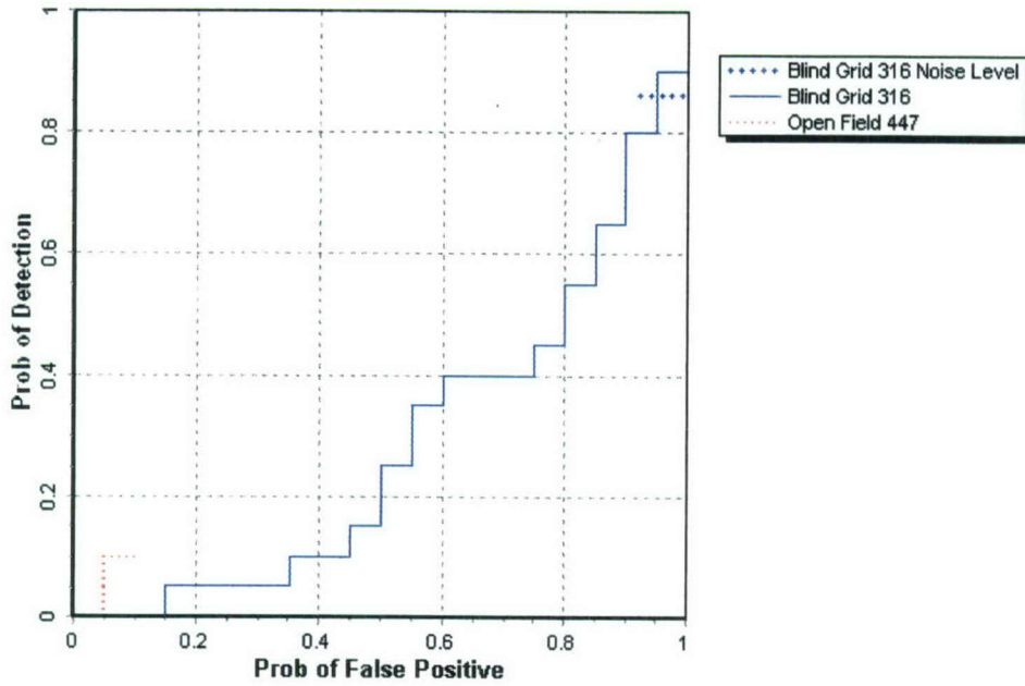
Figure 6. UXO MAPPER G856 MAG/pushcart P_d^{res} stages versus the respective P_{fp} over all ordnance categories combined.
