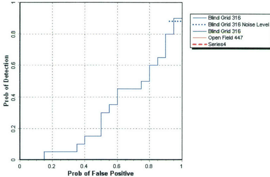
Figure 8. UXO MAPPER G856 MAG/pushcart P_d^{res} versus the respective P_{fp} for ordnance larger than 20 mm.
