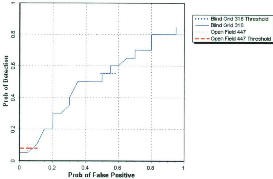
Figure 7. UXO MAPPER G856 MAG/pushcart P_d^{disc} versus the respective P_{fp} over all ordnance categories combined.
