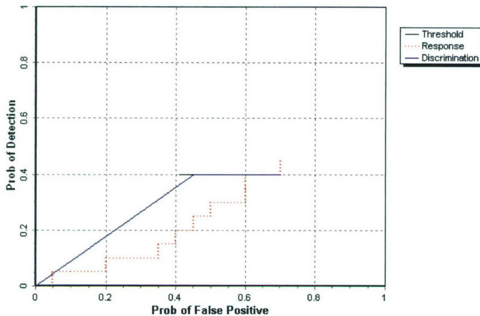
Figure 2. EM TM-5/sling desert extreme probability of detection for response and discrimination stages versus their respective probability of false positive over all ordnance categories combined.
