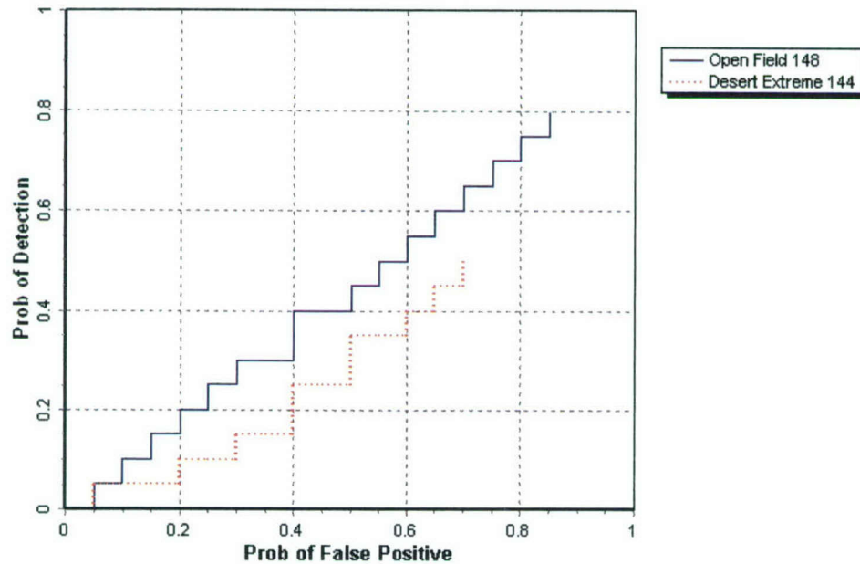
Figure 8. EM TM-5/sling P_d^{\text{res}} versus the respective P_{\text{fp}} for ordnance larger than 20 mm.
