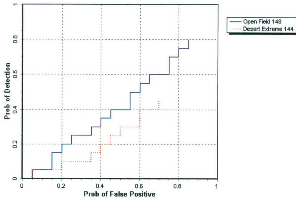
Figure 6. EM TM-5/sling P_d^{\text{res}} stages versus the respective P_{\text{fp}} over all ordnance categories combined.
