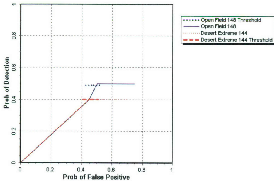
Figure 7. EM TM-5/sling P_d^{\text{disc}} versus the respective P_{\text{fp}} over all ordnance categories combined.
