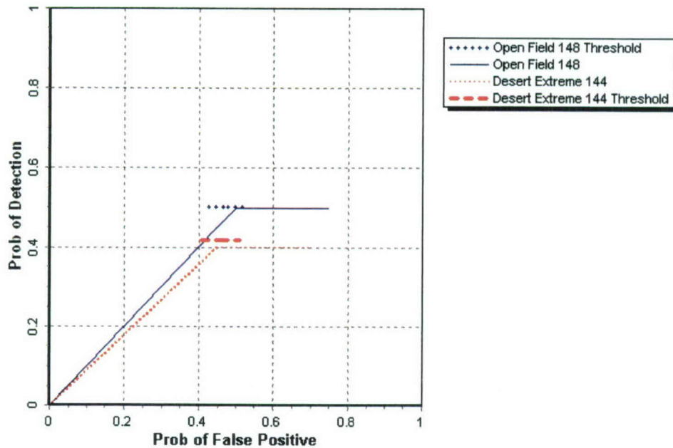
Figure 9. EM TM-5/sling P_d^{disc} versus the respective P_{fp} for ordnance larger than 20 mm.
