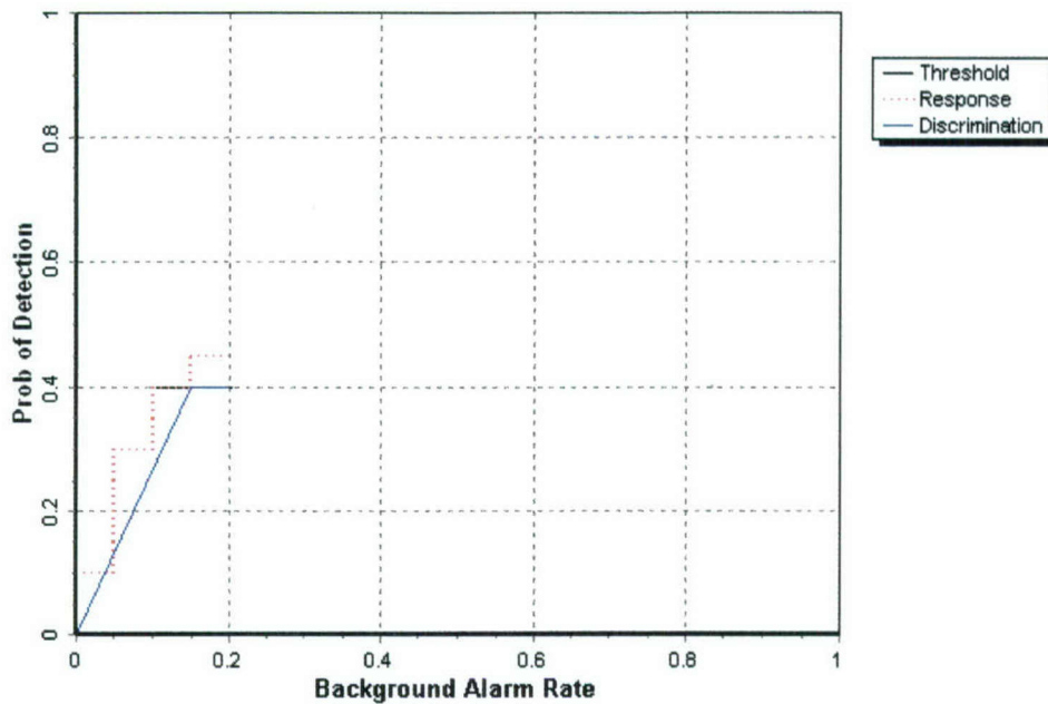
Figure 3. EM TM-5/sling desert extreme probability of detection for response and discrimination stages versus their respective background alarm rate over all ordnance categories combined.
