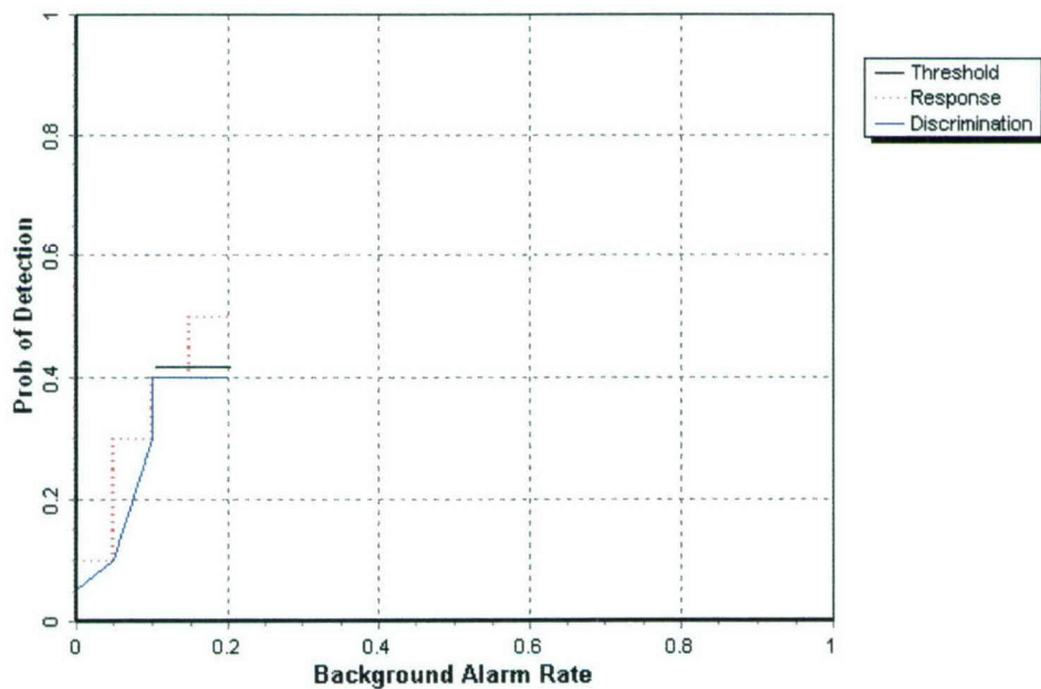
Figure 5. EM TM-5/sling desert extreme probability of detection for response and discrimination stages versus their respective background alarm rate for all ordnance larger than 20 mm.
