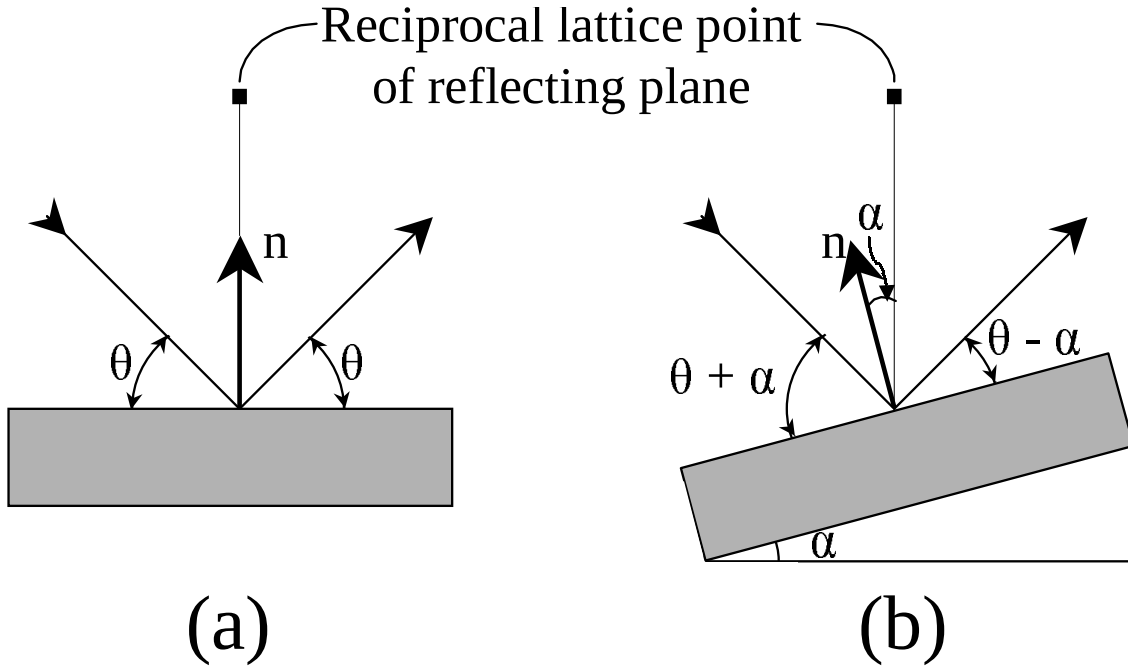
Figure 3.4 Configuration for XRD measurements on a single crystal thin film when: (a) the reciprocal lattice vectors of the reflecting planes are parallel to the surface normal; and (b) the asymmetrical case where reciprocal lattice vectors are aligned at an angle \alpha to the sample surface normal (after Hammond [41, Fig. 9.16]).
