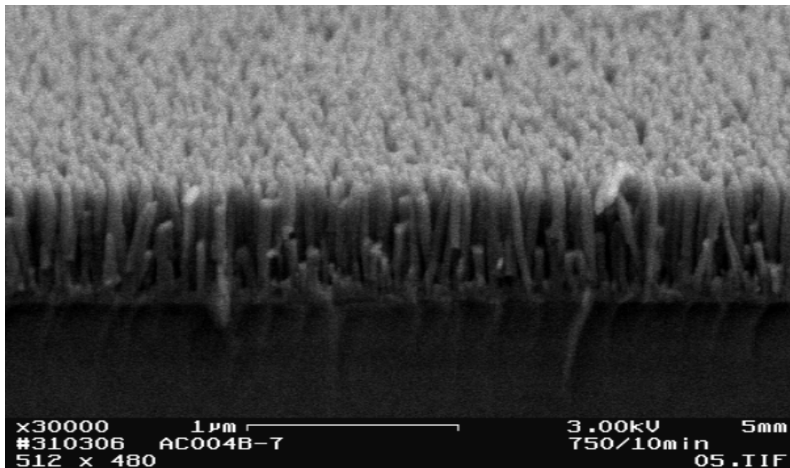
Figure 7.27 An SEM image of ZnO nanotips as-grown on a glass substrate.
