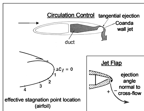
Figure 2. Circulation control airfoil configuration: rounded trailing edge with tangential mass ejection; a jet-flap configuration is shown for comparison. A change in effective stagnation point location increments lift as indicated.
