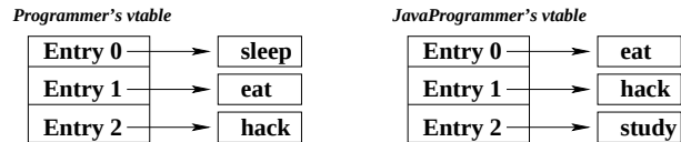
Figure 1: The vtables.
