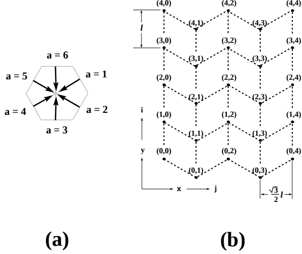
Figure 3: (a) Lattice vector label convention; (b) Hexagonal lattice convention with lattice directions a = 3 up and a = 6 down. Coordinates above the lattice nodes are (i, j) memory array indices.
