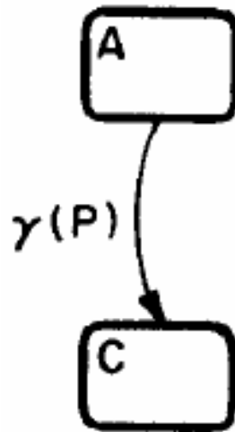
Figure 3.9: State D [17]
