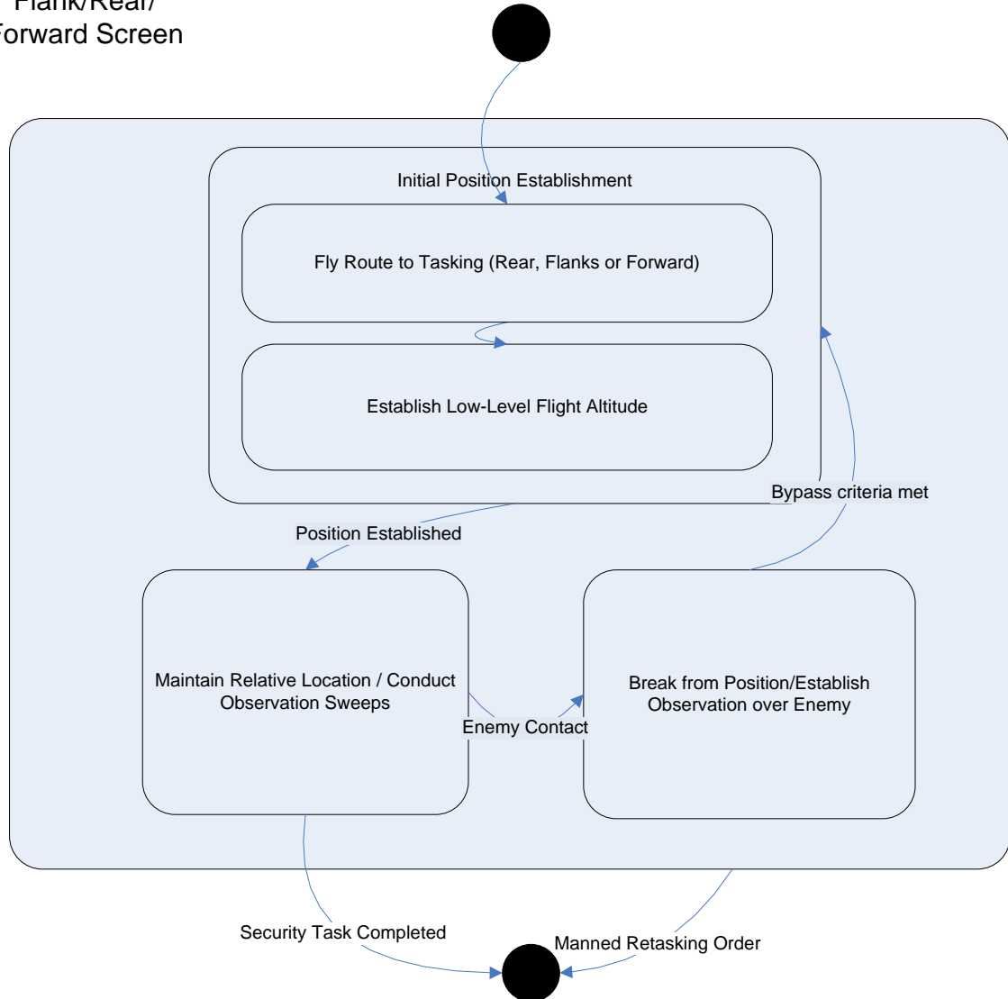
Figure 4.21: Screening Statechart
