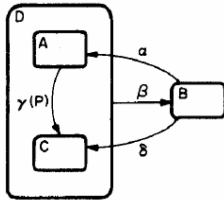
Figure 3.5: Statechart Representation [17]
