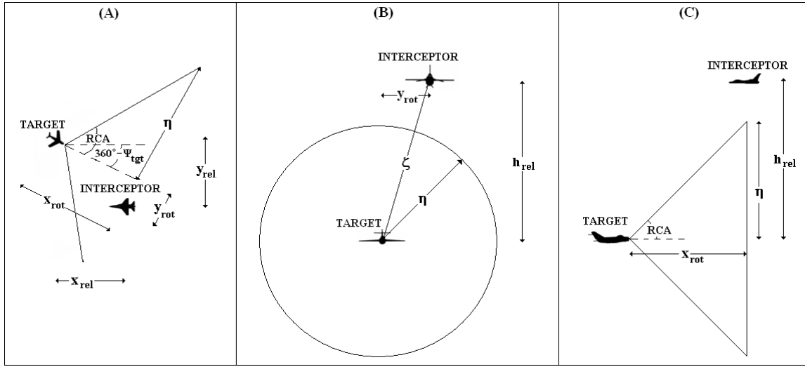
Figure 5-5: (x_{rot}, y_{rot}) are (x_{rel}, y_{rel}) rotated by the negative of the target's heading angle \Psi_{tgt} . RCA is the target's radar cone angle, and \eta is the radius of the radar cone at x_{rot} . h_{rel} is the interceptor's altitude relative to the target's. \zeta is the distance from the target to the interceptor in the plane containing altitude and the rotated relative y position y_{rot} .
