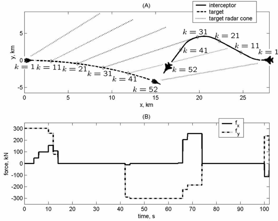
Figure 4-9: Beam intercept using MILP where interceptor is required to fly to a distance of at least 12.2km along the target's radar cone. Figure (A) shows the aircrafts' trajectories along with the radar cone limit of the target, and Figure (B) is the interceptor's control history. The target is turning at a constant rate of 0.3^\circ/s . The interceptor performs the maneuver in a similar manner as Figure 4-8 but with exaggerated turns in order to fly around the stronger radar.
