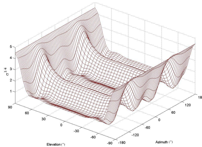
Figure 2-6: Generic aircraft radar cross section model [23]
