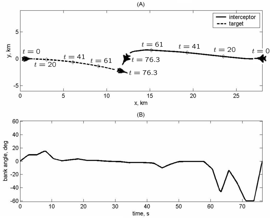
Figure 5-17: Figure (A) shows a beam intercept trajectory in the (x, y) plane where the target is turning at a constant rate of 0.3^\circ/\text{s} . The interceptor begins with a slight turn away from the target and travels along an approximately straight line for the majority of the maneuver. The trajectory is completed with a final turn towards the target. Figure (B) is the interceptor's bank angle history.
