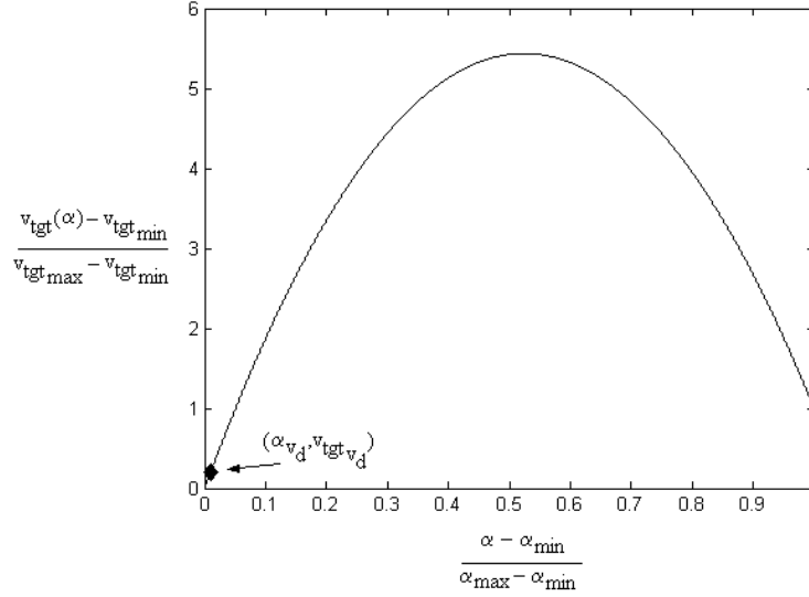
Figure 6-9: Curve describing problem with single interpolation approach
