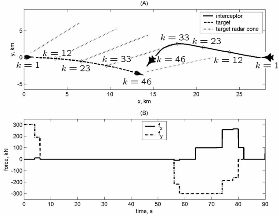
Figure 4-8: Beam intercept using MILP where interceptor is required to fly to a distance of at least 9.2km along the target's radar cone. Figure (A) shows the aircrafts' trajectories along with the radar cone limit of the target, and Figure (B) is the interceptor's control history. The target is turning at a constant rate of 0.3^\circ/s . The interceptor begins the maneuver with a right turn in order reach the end of the target's radar cone. Shortly before reaching this point, a hard left turn is executed to wrap around the radar cone and to point the interceptor towards the desired endstate.
