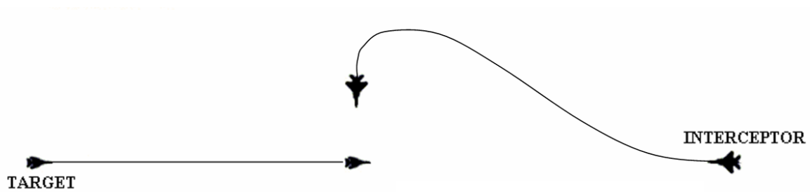
Figure 2-5: The beam intercept usually consists of two turns. The first is a turn away from the target to obtain the desired separation range. The second is a turn towards the target to point the interceptor's velocity vector at the target.
