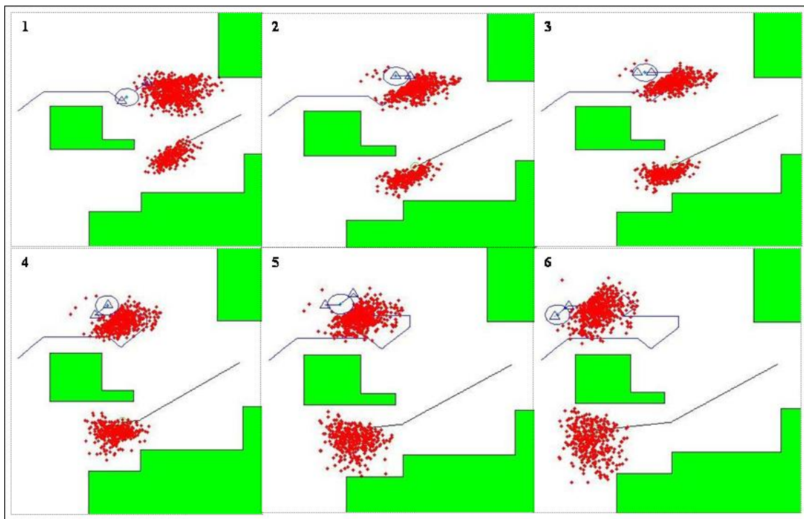
Figure 6.12: Path Planning Search Algorithm (Search Depth = 1) Initial Sequence of Events for Scenario 2
