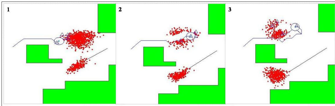
Figure 6.16: Illustration of Poor Search Performance Due to Low Resampling Frequency
