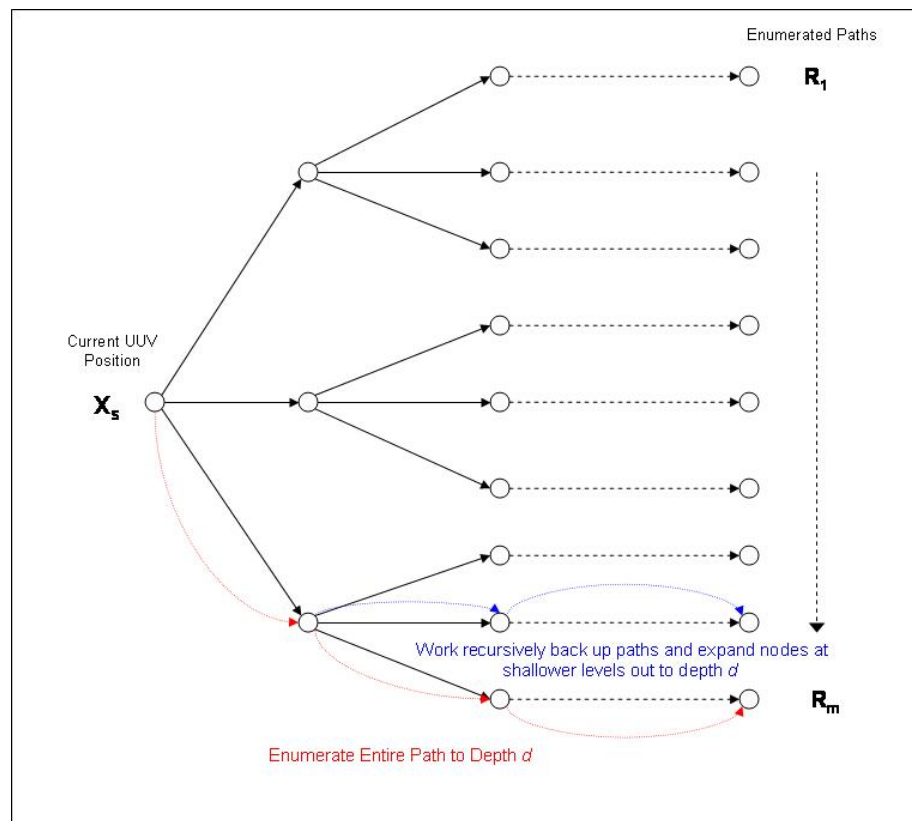
Figure 5.13: Depth-First Path Enumeration Illustration
