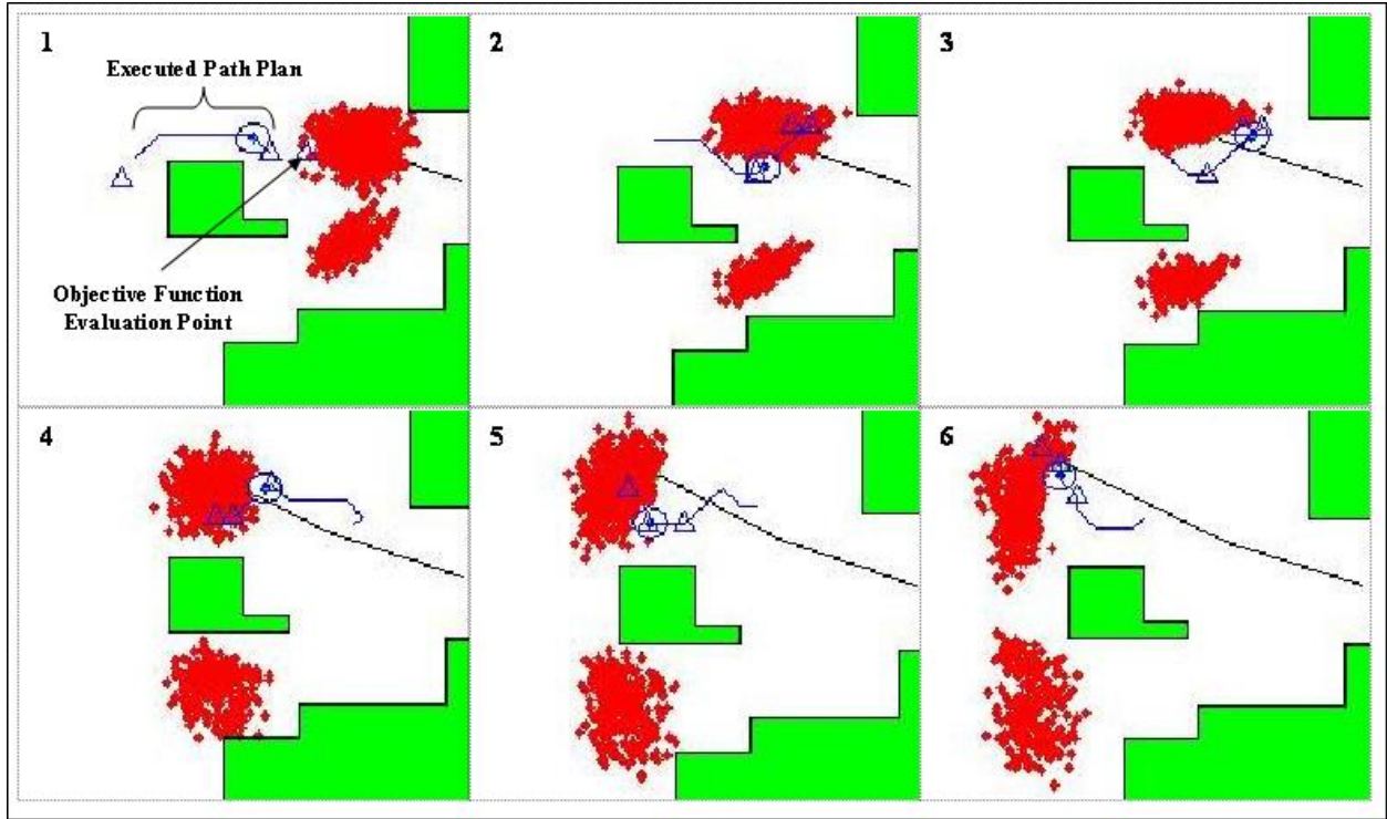
Figure 6.14: Path Planning Search Algorithm (Search Depth = 2), Sequence of Scenario 1 Events
