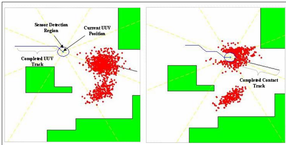
Figure 6.2: Contact Detection Using Sector-Based Search
