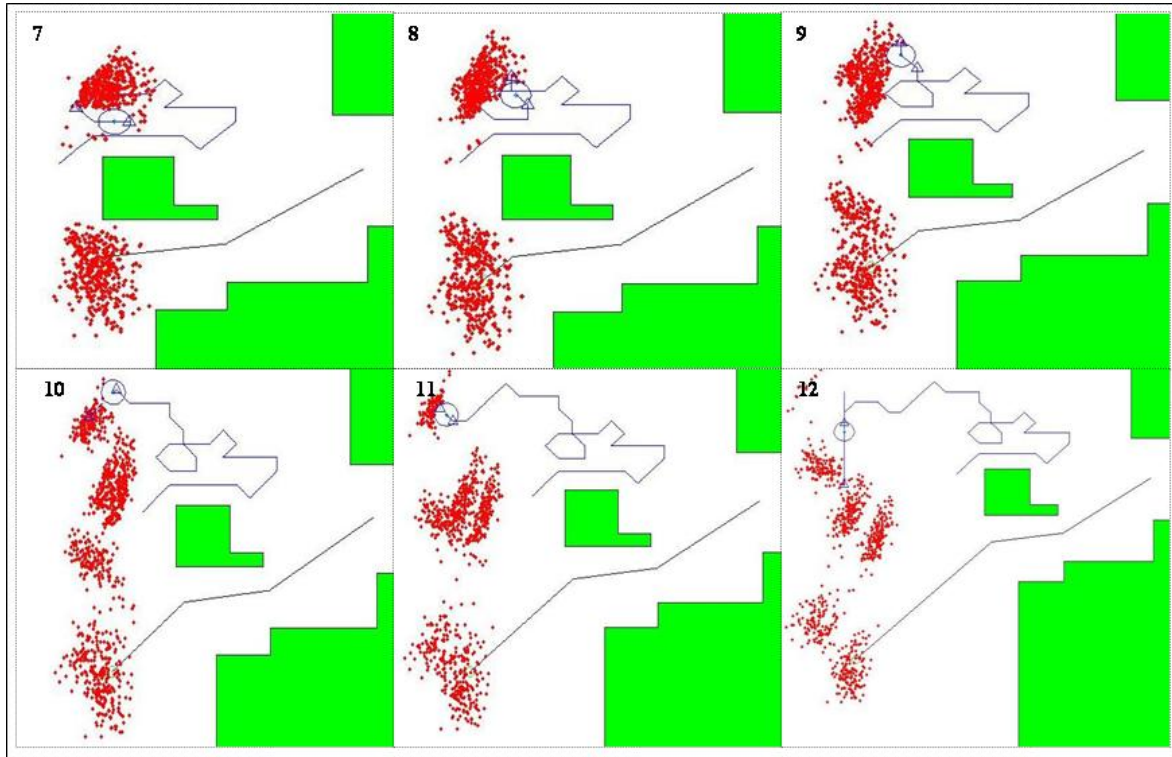
Figure 6.13: Path Planning Search Algorithm (Search Depth = 1) Remaining Sequence of Events for Scenario 2
