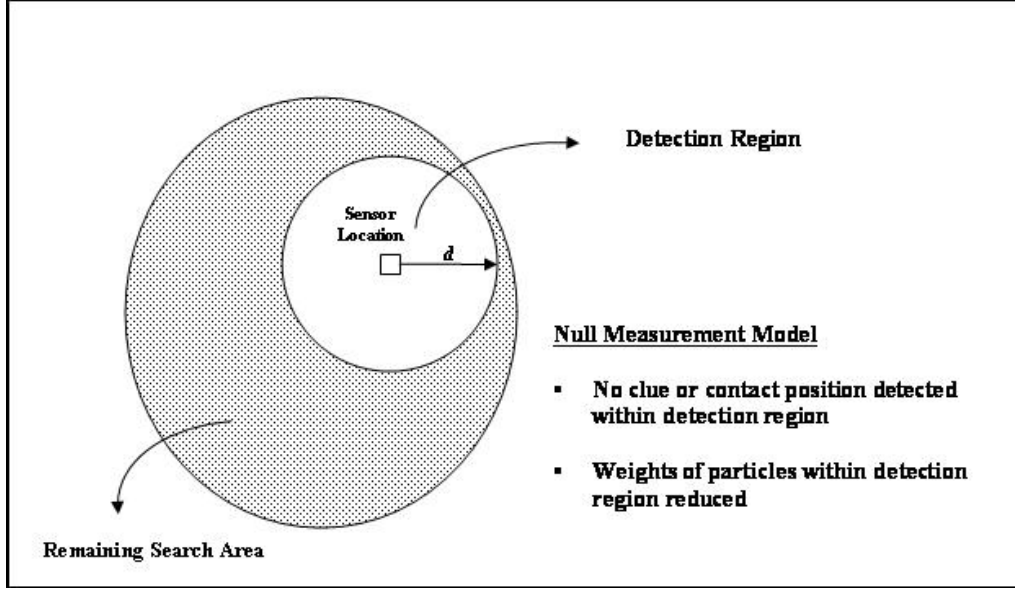
Figure 4.8: Illustration of Null Measurement Model
