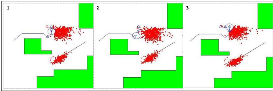
Figure 6.17: Improved Search Performance Due to Increased Sampling Frequency
