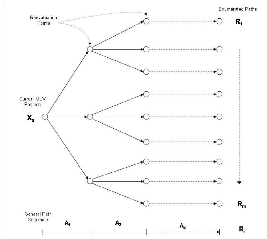
Figure 5.11: Path Enumeration Illustration
