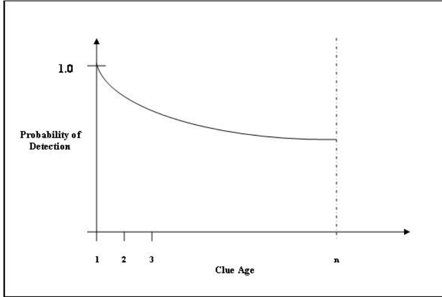
Figure 4.3: Sensor Detection Rate - Probability of Clue Detection Given that a Clue Exists
