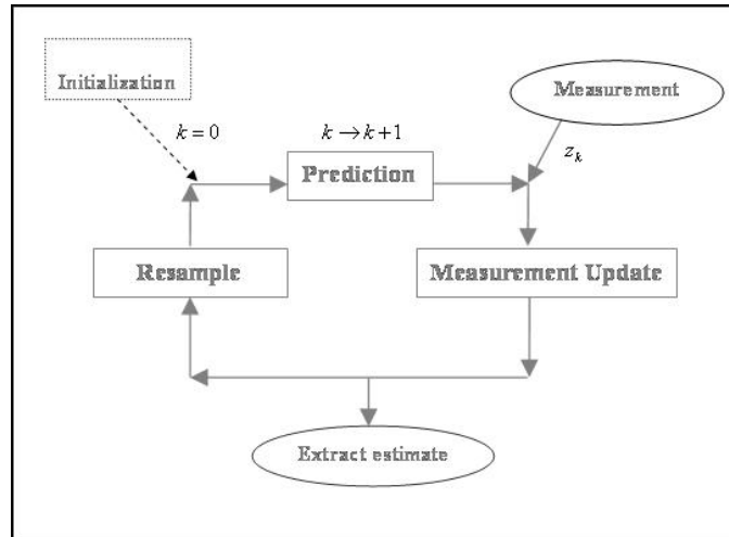
Figure 3.2: Recursive Particle Filter Algorithm
