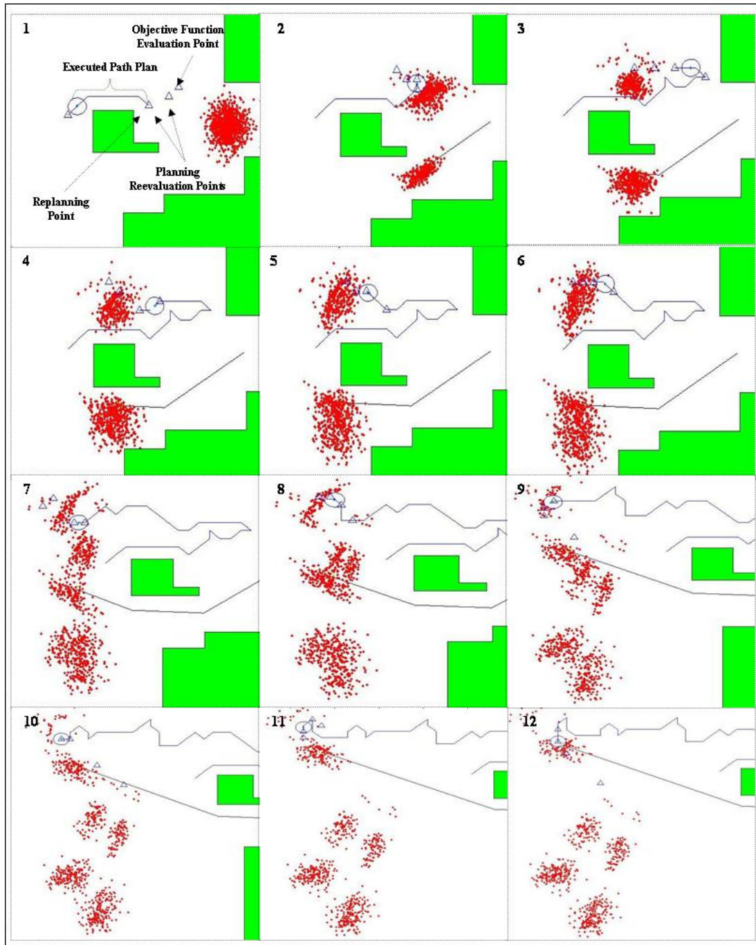
Figure 6.15: Path Planning Search Algorithm (Search Depth = 3), Sequence of Scenario 2 Events
