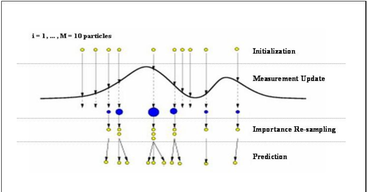
Figure 3.3: Particle Filter Illustration
