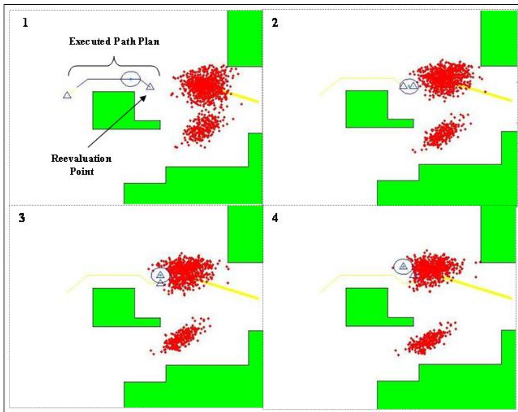
Figure 6.10: Initial Sequence of Actions using the Dynamic Action Space Path Planner
