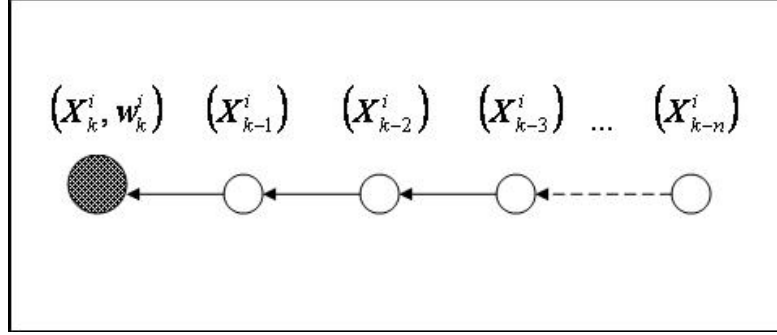
Figure 4.6: Particle Array Illustration
