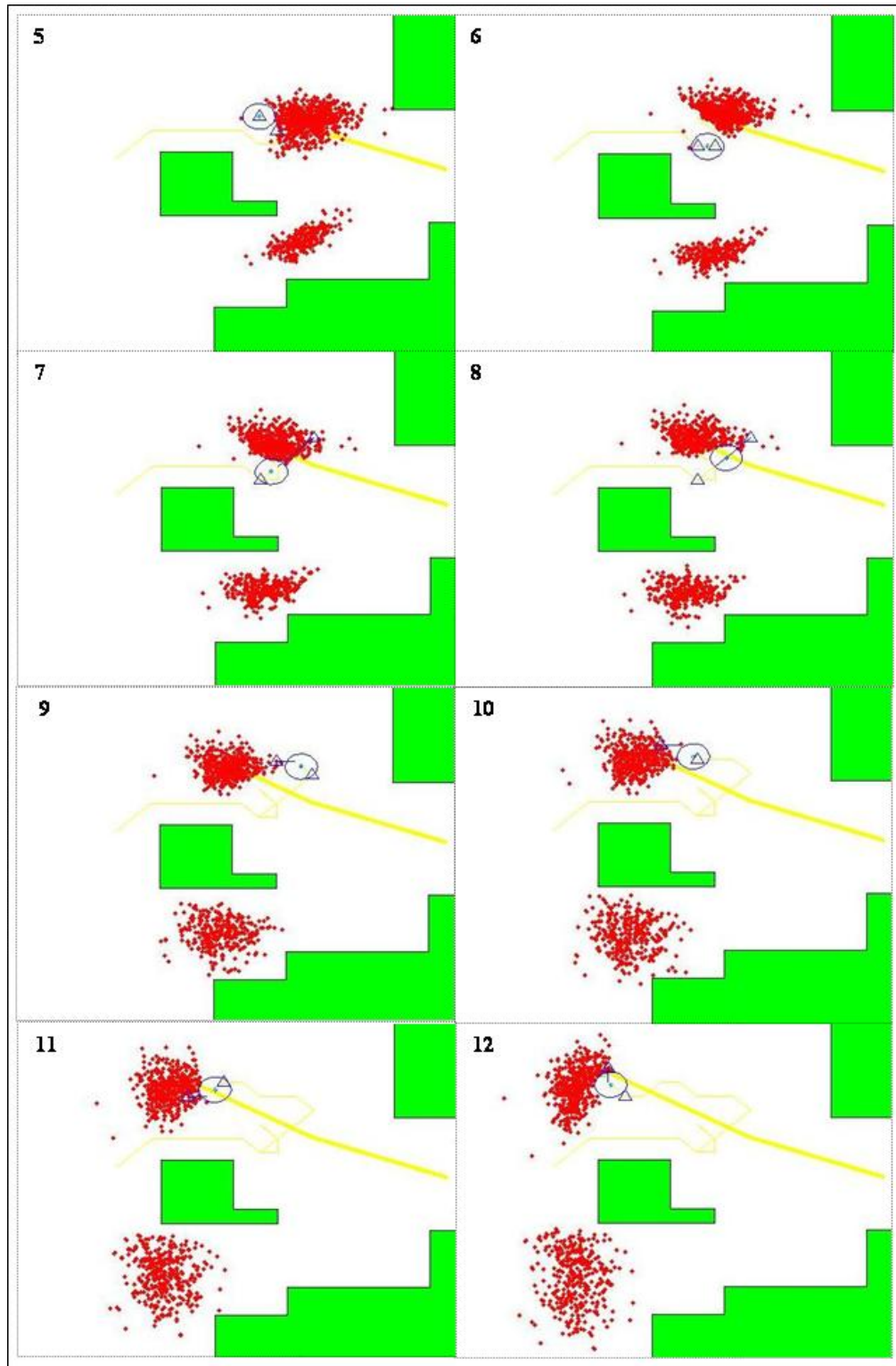
Figure 6.11: Continued Sequence of Dynamic Actions Leading to Detection
