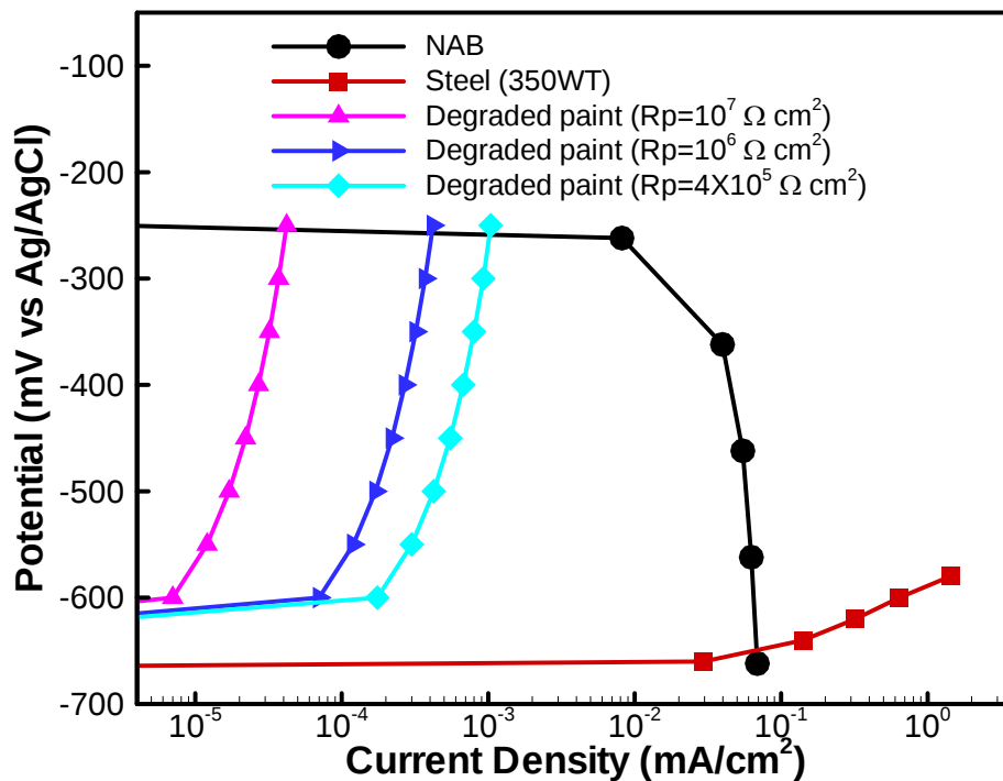
Figure 2. Polarization curve data for NAB, 350WT steel and degraded paint coating.
