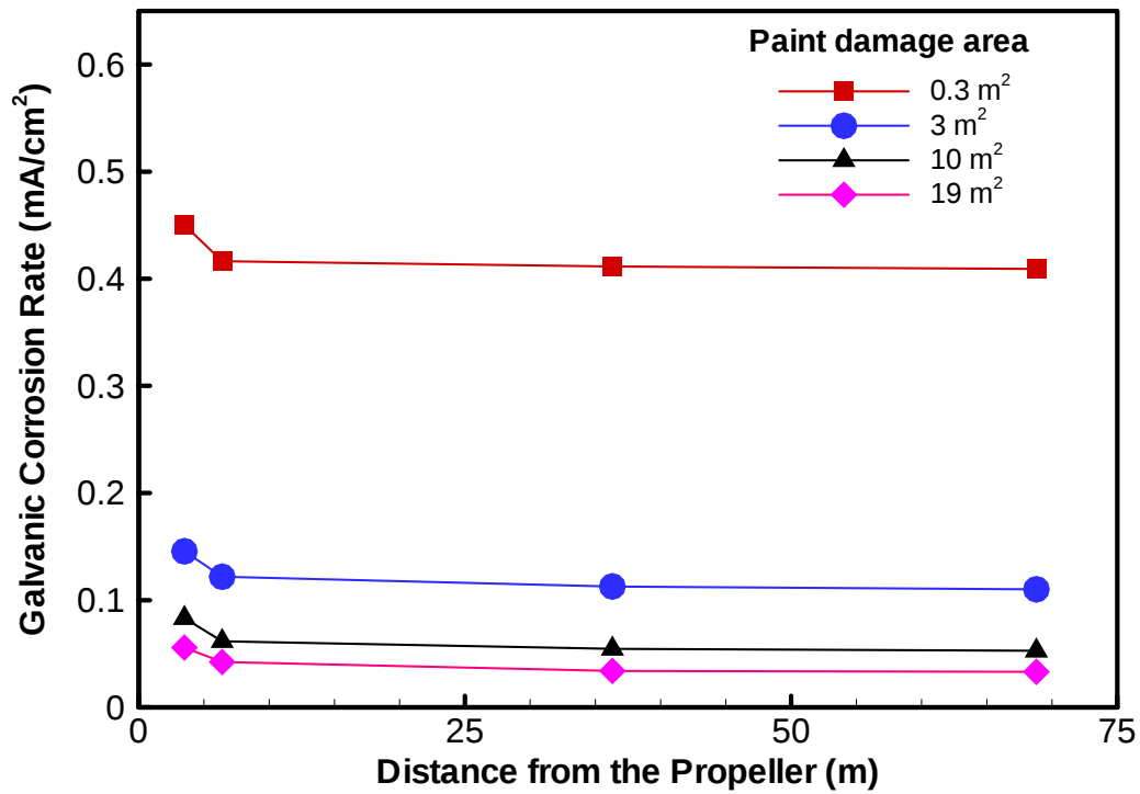
Figure 3. Galvanic corrosion rates as a function of distance from the propeller
