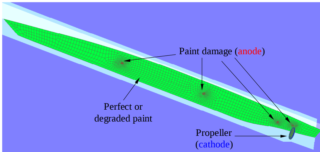
Figure 1. Ship model for galvanic corrosion modelling.
