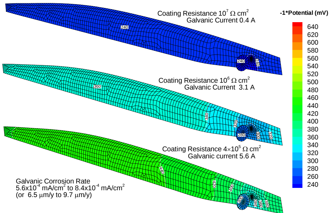
Figure 7. Potential contours on the ship hull computed at various stages of paint degradation.
