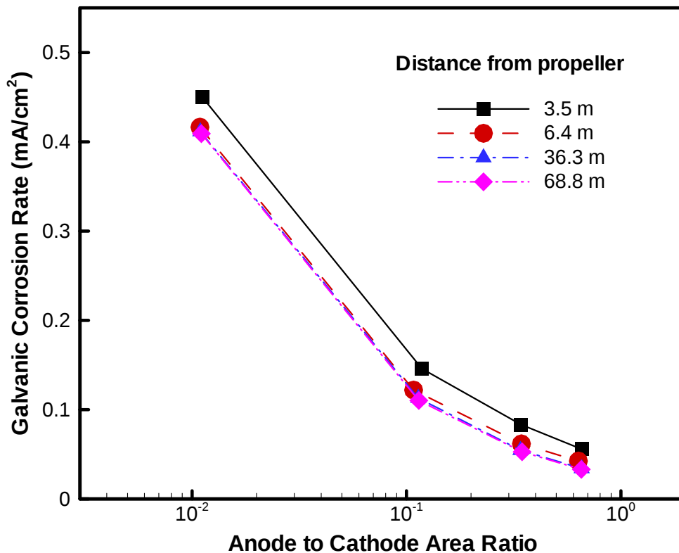
Figure 6. Effect of paint damage area on galvanic corrosion rate.
