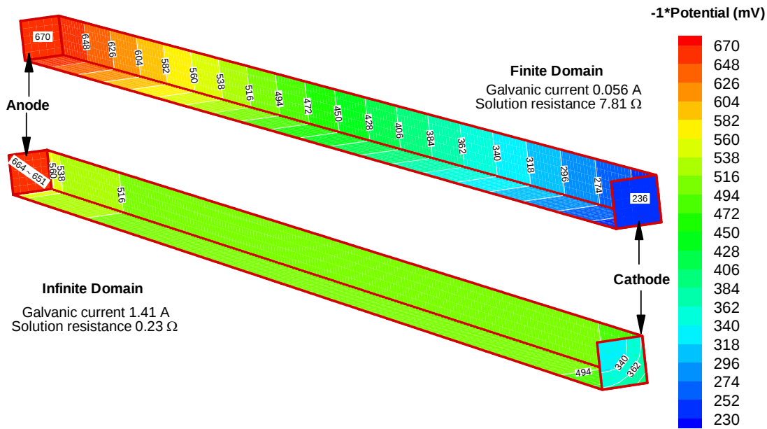
Figure 5. Potential contours on the box surface in both finite and infinite domains.
