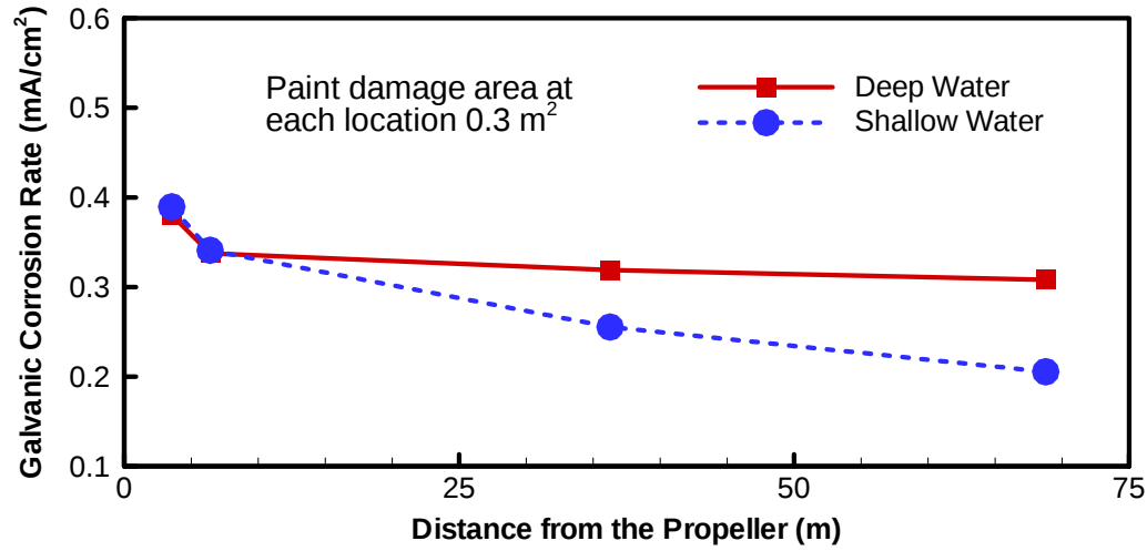
Figure 4. Distribution of the galvanic corrosion current among the four paint damage sites (0.3 m 2 paint damage at each site).
