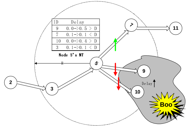
Figure 3. Back-pressure rerouting case one
