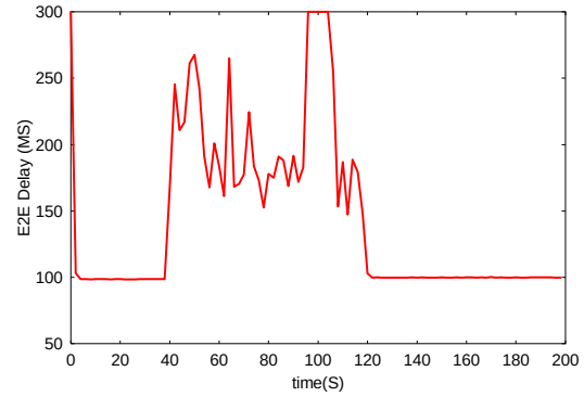
Figure 5.A. E2E delay profile of DSR
