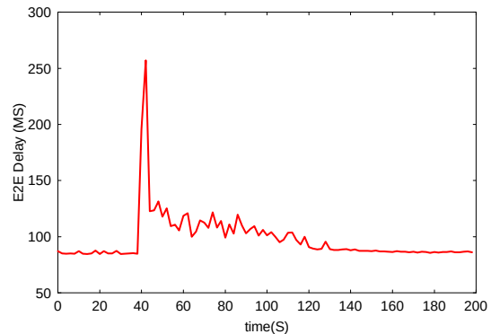
Figure 5.D E2E delay profile of SPEED
