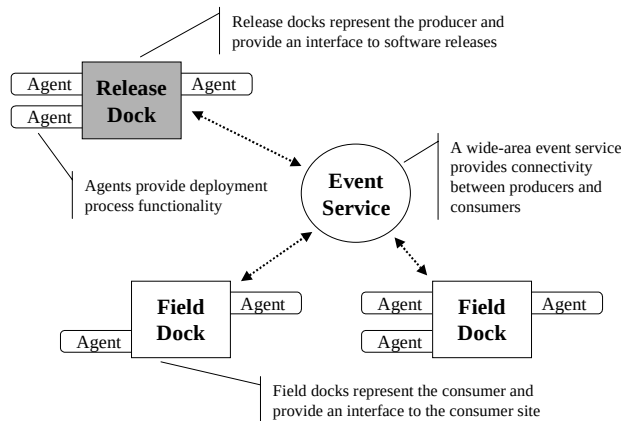
Figure 1: Software Dock Architecture
