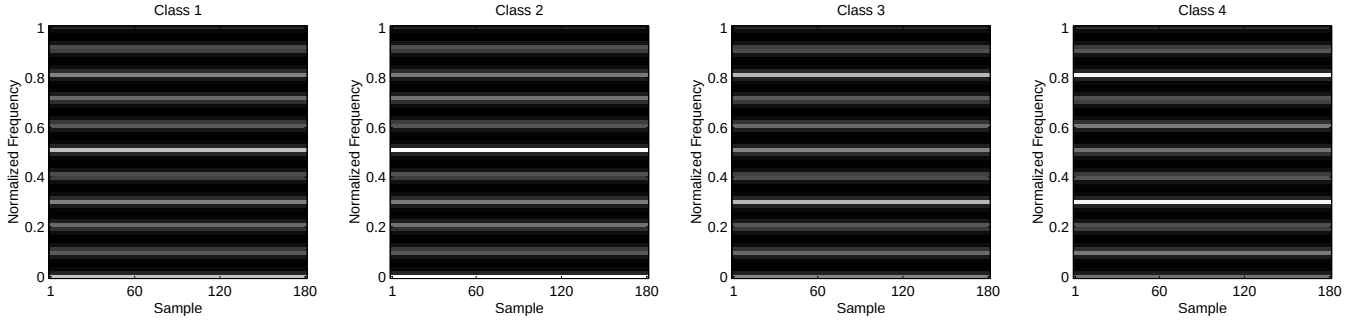
Figure 6. Example of the log magnitude of the class-dependent TFR ( 20 \log_{10}|CD| ) from each class under Case 2. These are generated using two kernel points. The largest magnitude is represented by the darkest gray-scale value.
