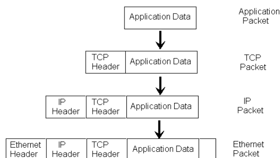
Figure 4: Data Encapsulation 3
