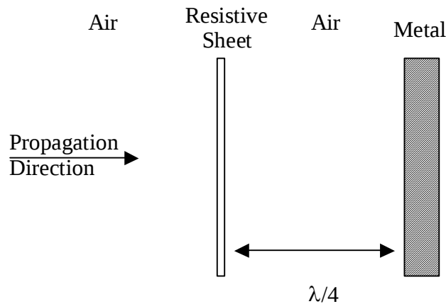
Figure 2. Salisbury Screen
