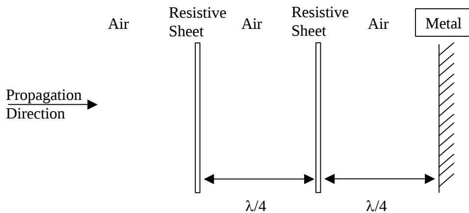
Figure 3. Jaumann Layers
