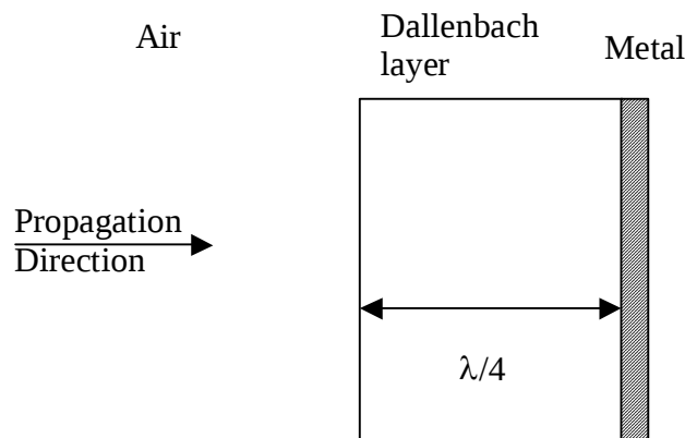
Figure 1. Dallenbach Layer
