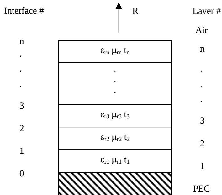
Figure 4. Reflectivity from Jaumann absorber layers
