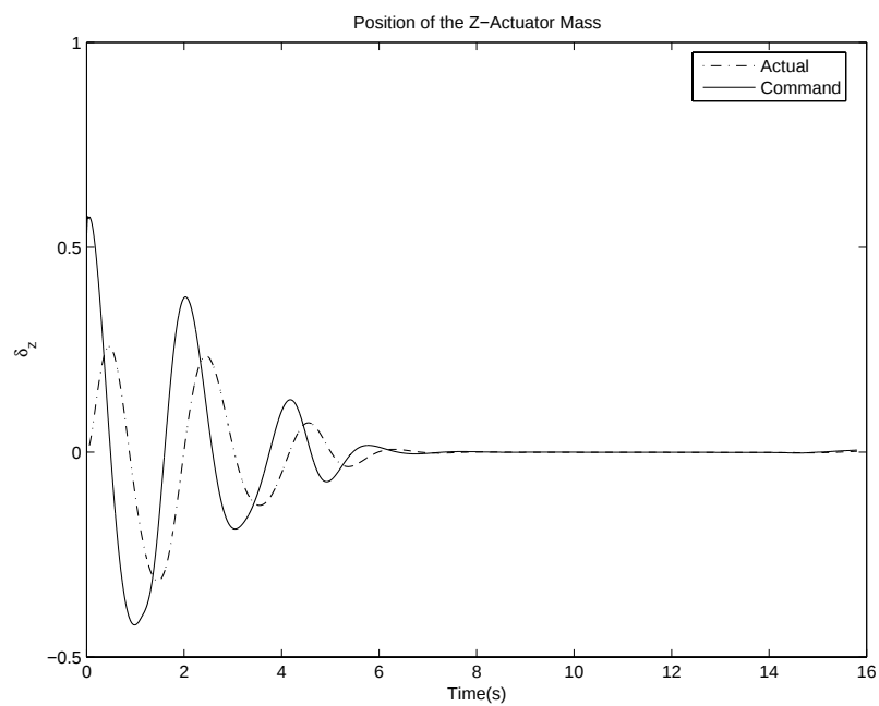
Figure 8. Displacement of the Z-Actuator Moving Mass
