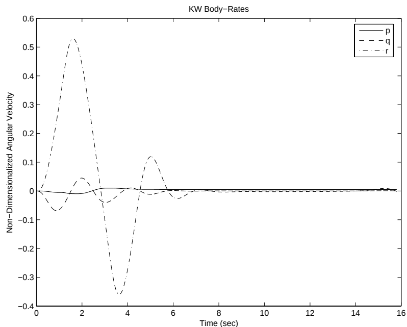
Figure 9. Body Rates of the KW
