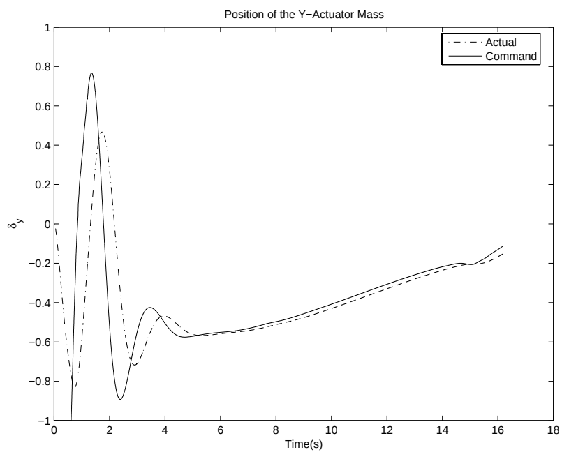
Figure 14. Displacement of the Y-Moving Mass
