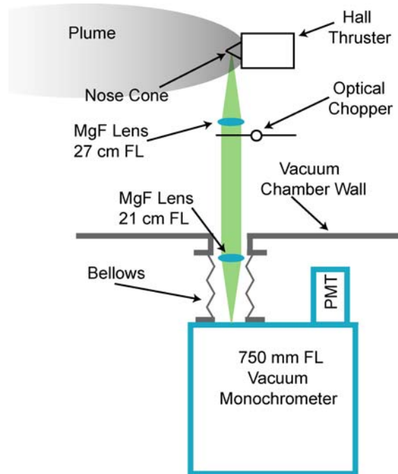
Fig. 2. Experimental apparatus for measurement of boron emission from the nose cone of a 200 W Hall thruster.
