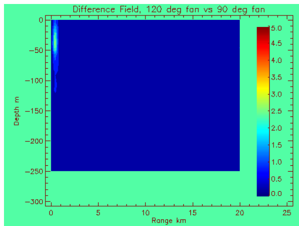
Figure 3. Comparison of the difference in dB between the full field transmission loss predictions using a 120° angle fan and a 90° angle fan.
