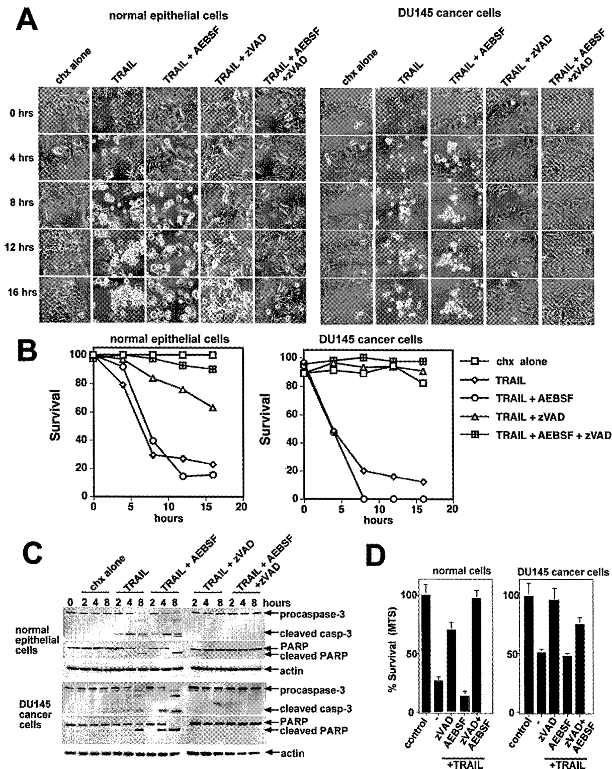
Figure 1. TRAIL can kill normal and cancerous epithelial cells by different mechanisms. (A) Time-lapse microscopy of normal prostate epithelial cells or prostate cancer cells treated with TRAIL plus AEBF and zVAD.fmk. TRAIL kills both cell types, but zVAD.fmk alone can protect only the cancer cells; the combination of zVAD.fmk and AEBF is required to protect normal cells from TRAIL-induced death. (B) The number of dead cells for each time point was determined by counting rounded cells in individual frames for each treatment. Treatment with zVAD.fmk in the normal cells altered the slope of the line, indicating that the caspase-independent cell death response in normal cells occurred more slowly than caspase-dependent cell death. (C) Normal or cancerous prostate cells were treated with TRAIL in the presence of the protease inhibitors and harvested for Western blot analysis of caspase-3 and PARP cleavage. In both cell types, caspase-3 was activated, leading to PARP cleavage, and the caspase inhibitor zVAD.fmk completely blocked the response. (D) MTS assays of TRAIL treated cells were performed. ZVAD.fmk only partially protected normal cells but completely protected cancer cells. The combination of zVAD.fmk and AEBF completely protected normal cells.
