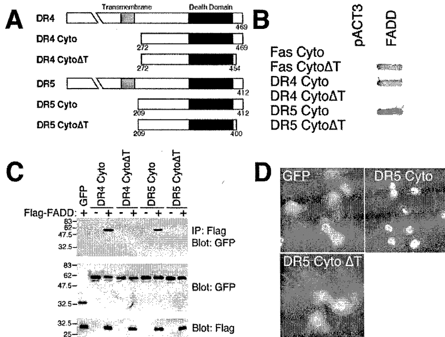
FIG. 1. The C terminus of DR4 and DR5 binds directly to FADD and is required for induction of apoptosis. A , graphical representation of DR4 and DR5 constructs. The indicated fragments were cloned into GFP or two-hybrid vectors. B , binding of Fas, DR4, and DR5 constructs to empty vector (pACT3) or FADD was measured by directed two-hybrid. FADD binds only to Fas when the 15 C-terminal amino acids are removed, but binds to DR4 and DR5 only when the C-terminal tail is present. C , HeLa cells were transfected with GFP or GFP-DR5 constructs. After 14 h, green cells expressing DR5 Cyto (green) show typical signs of apoptosis while cells expressing GFP alone or DR5 CytoΔT do not, indicating that the C-terminal tail of DR5 is required for apoptosis. D , HeLa cells were transfected with GFP-DR constructs along with empty FLAG vector (FLAG) or FLAG-FADD. FLAG complexes were immunoprecipitated and blotted with a GFP-specific antibody. Consistent with the results in two-hybrid assays, only DR4 Cyto and DR5 Cyto but not DR5 CytoΔT or DR5 CytoΔT bind FADD.
