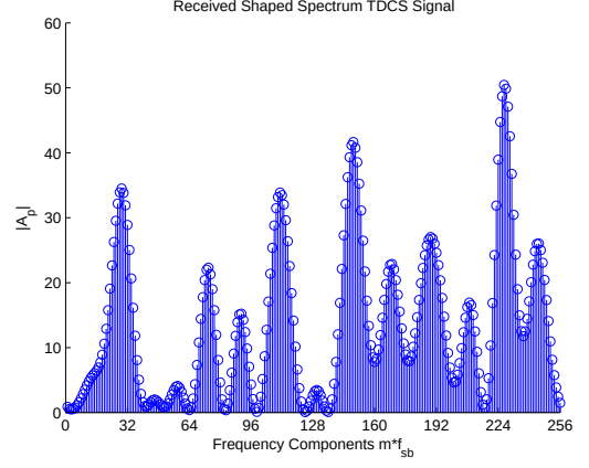
Figure A.5: Received Shaped Spectrum TDCS Signal
