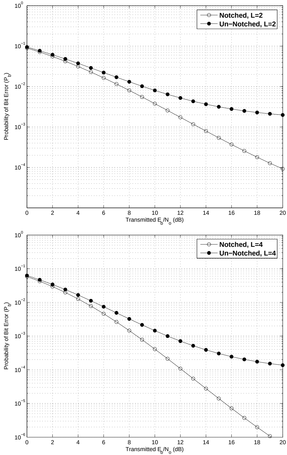
Figure 3.18: Notched vs Un-notched Analytical Results, L = 2, 4 . These figures demonstrate the predicted interference avoidance capability of the notching algorithm applied to spectrally encoded, shaped spectrum TDCS signals using an L -diversity RAKE receiver. For these plots, J/S = 64 and the notching algorithm attenuates average interferer power by 11.8dB
