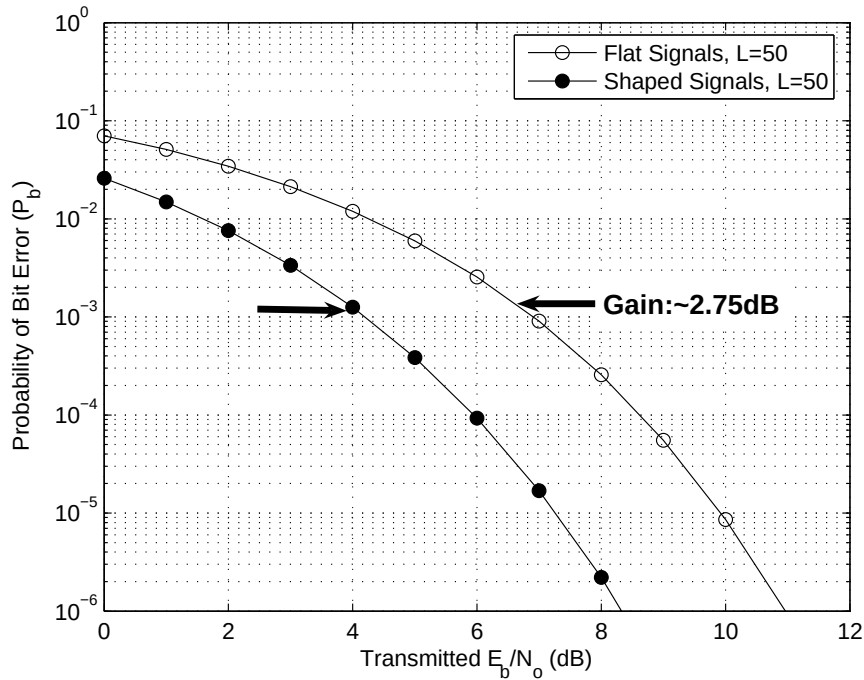
Figure 3.9: Analytical P_b Comparison for Spectrally Encoded and Un-encoded Signals, L = 20, 50 . These figures demonstrate the benefit of spectral encoding applied to the RAKE receiver at equivalent diversities L .
