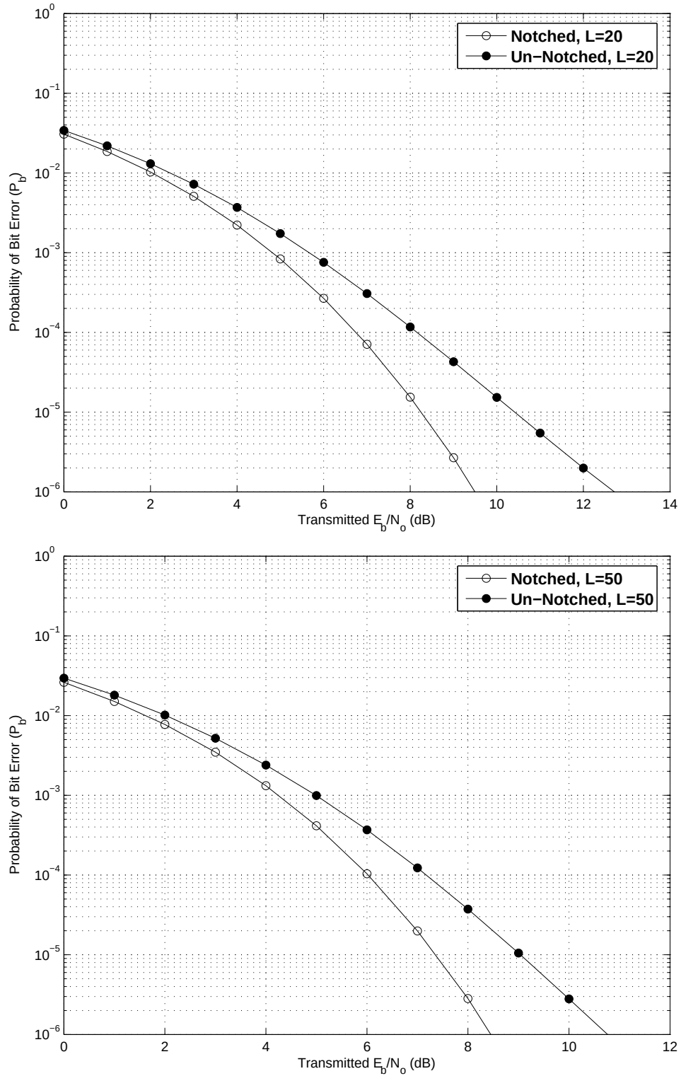
Figure 3.19: Notched vs Un-notched Analytical Results, L = 20, 50 . These figures demonstrate the predicted interference avoidance capability of the notching algorithm applied to spectrally encoded, shaped spectrum TDCS signals using an L -diversity RAKE receiver. For these plots, J/S = 64 and the notching algorithm attenuates average interferer power by 11.8dB
