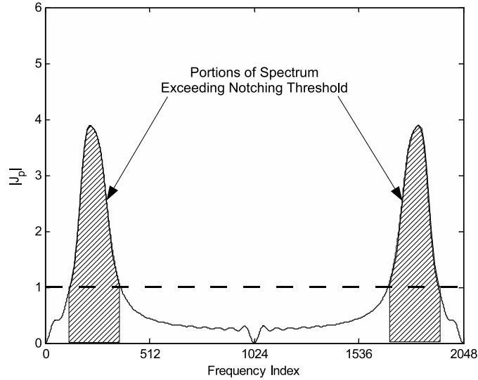
Figure 3.10: Conceptual Transmitted Interference Spectrum. This figure demonstrates the effect of the notching algorithm when no multipath fading occurs on the interference channel.
