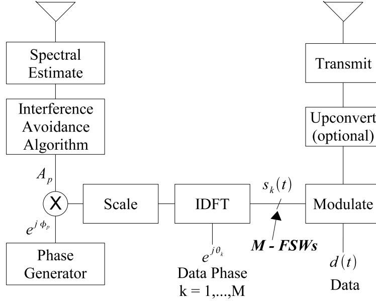
Figure 2.1: Conceptual TDCS Transmitter
