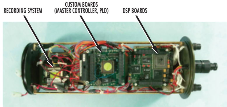
FIGURE 6. Hydra/Kelp node. The node design has evolved over 3 years and now forms a simple, yet powerful, flexible, modular, and expandable platform for evaluating advanced algorithms. Furthermore, reliable forward and backlinks, implemented through an underwater modem, provide scientists and engineers with solid control over mission execution.
