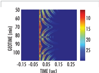
FIGURE 10. Modeled multipath at a single Hydra array element during two array crossings. The model accurately reconstructs the measured multipath shown in Figure 9.
