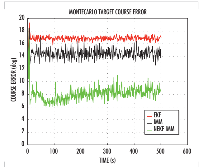
FIGURE 4. NEKF IMM, IMM, and EKF course errors for 100 Monte Carlo runs.
