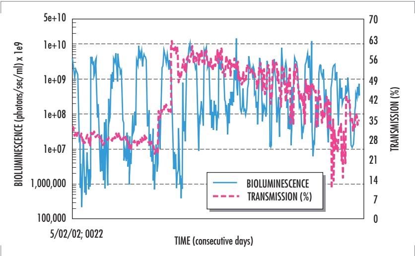
FIGURE 4. BioBuoy 1 bioluminescence data, San Diego Bay, 2±29 May 2002.
