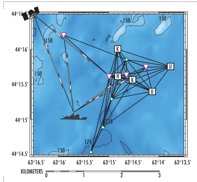
FIGURE 3. The October 2002 RDS-4 Seaweb network in the Approaches to Halifax supported the RDS-4 Rapidly Deployable Sensors Trials. Seaweb networking integrated U.S. and Canada experimental autonomous ASW sensors deployed on the seafloor. Gateway buoys supported FreeWave line-of-sight radio links and Iridium satellite links to the shipboard command center. Legend: ▽ – U.S. and Canada gateway buoys; H – U.S. Hydra HLA sensor; K – U.S. Kelp VLA sensors; U – Canada UCARA HLA sensors; ○ – U.S. Seaweb repeater nodes.
