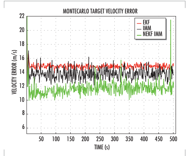
FIGURE 2. NEKF IMM, IMM, and EKF velocity errors for 100 Monte Carlo runs.
