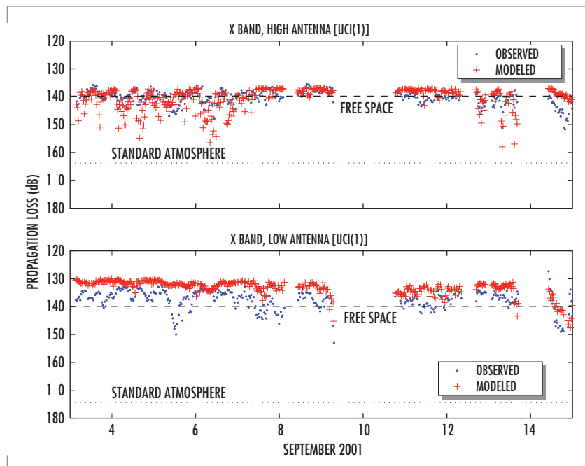
FIGURE 3. Comparison of modeled (red crosses) to measured (blue dots) propagation loss for both the high- and low-sited X-band (9.6 GHz) transmitters during RED. The modeled data are derived from meteorological measurements at level 1 (5.1 m asl) of the UCI array.
