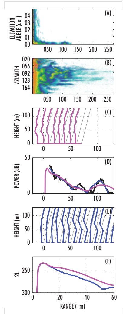
FIGURE 5. RFC-SBD (A) vertical scan, (B) horizontal scan, (C) helicopter-measured refractivity, (D) observed clutter [black], RFC best fit [blue] and clutter predicted using "c" [magenta], (E) RFC-inferred profiles, (F) two-way loss prediction for RFC [blue] and helicopter [magenta].
