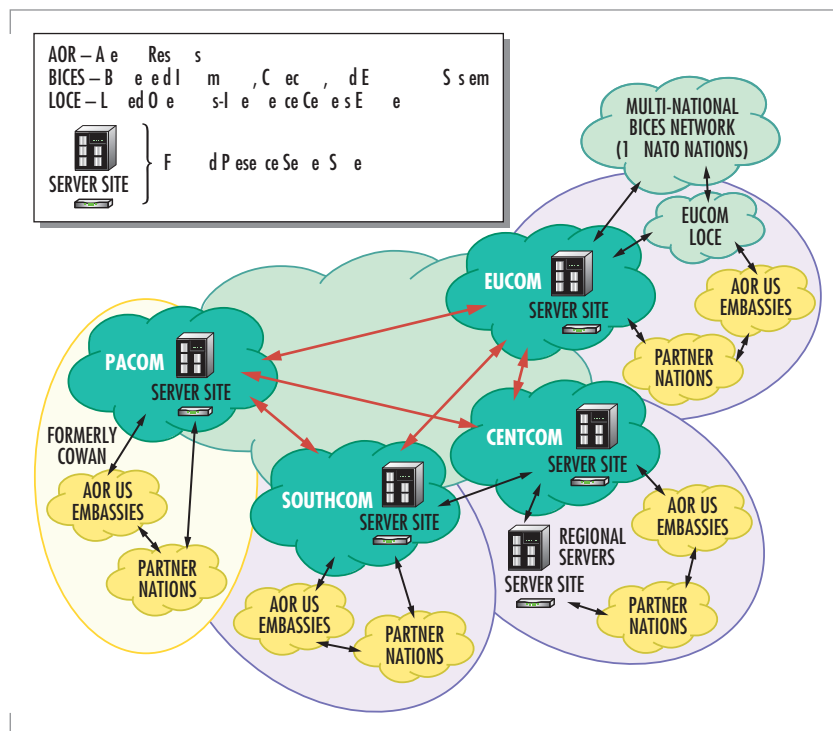
FIGURE 2. CENTRIXS architecture.
