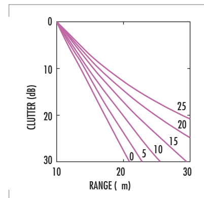
FIGURE 3. Clutter power (relative to power at 10 km) parametric in evaporation duct height.
