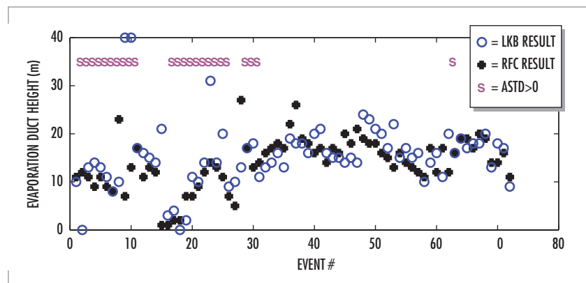
FIGURE 4. RFC-ED event series using data from USS Normandy (CG 60). Magenta "S" indicates matched pairs where surface layer is stable and LKB output is questionable.
