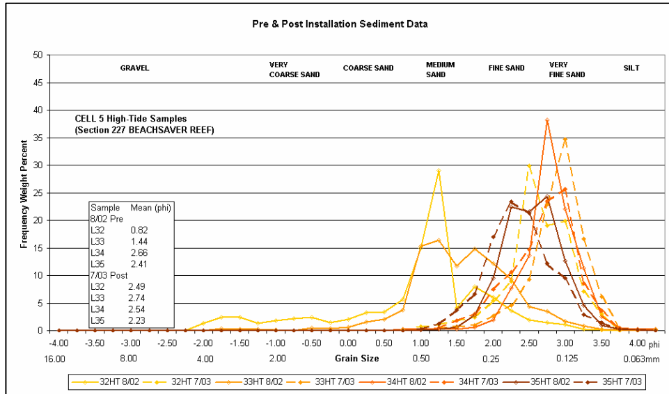
Figure A14. Sediment distribution change between 8/02 and 7/03 of high tide samples in cell 5
