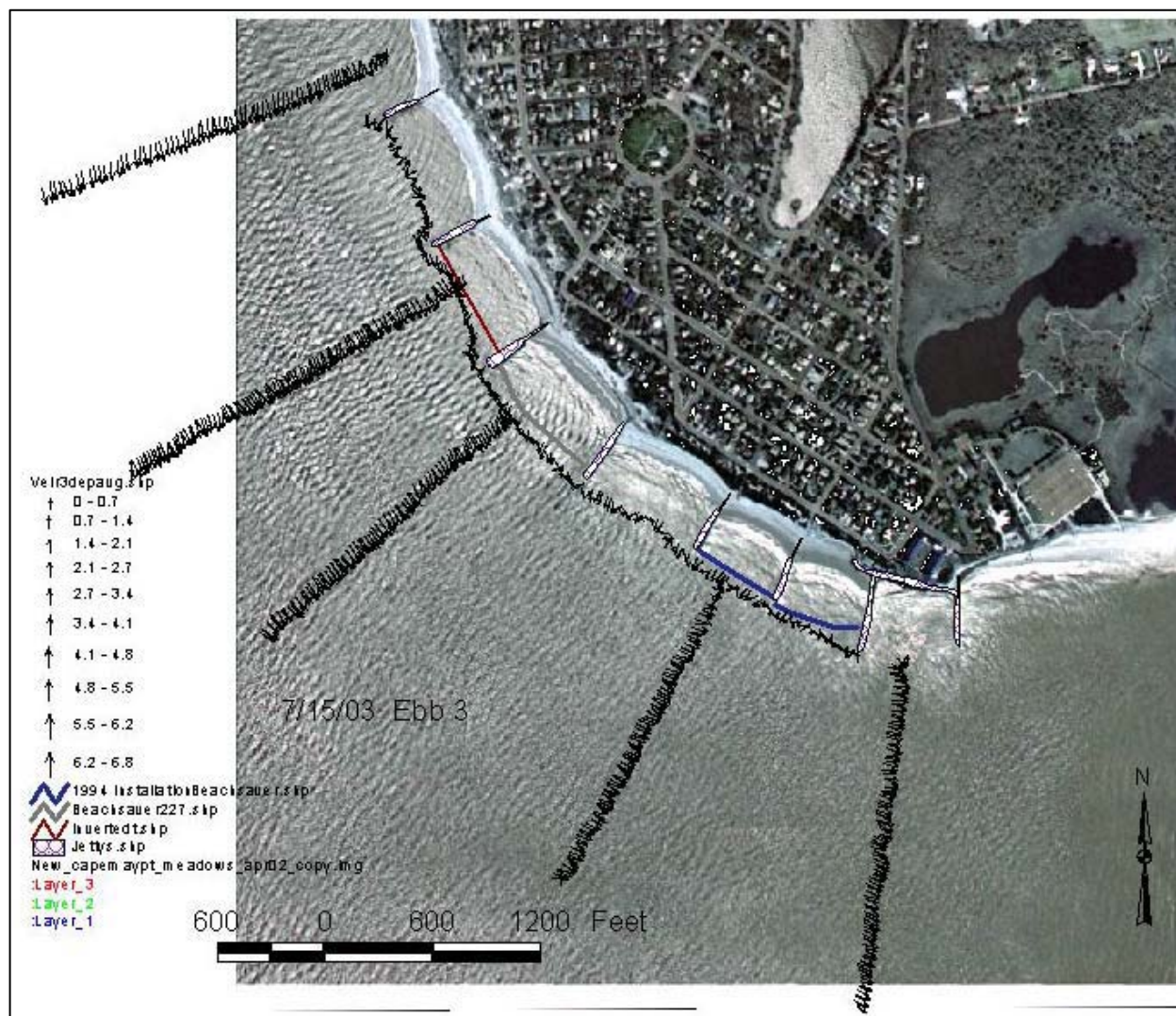
Figure 50. Depth averaged ADCP current velocity vectors for third ebb current survey on 7/15/03 at 1400. Velocity in feet per second
