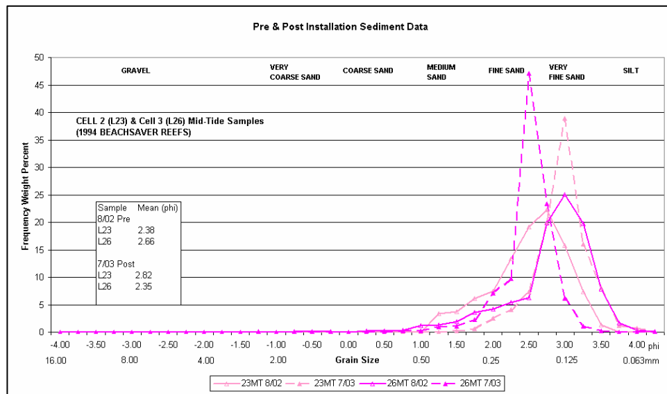
Figure A20. Sediment distribution change between 8/02 and 7/03 of midtide samples in cells 2 and 3
