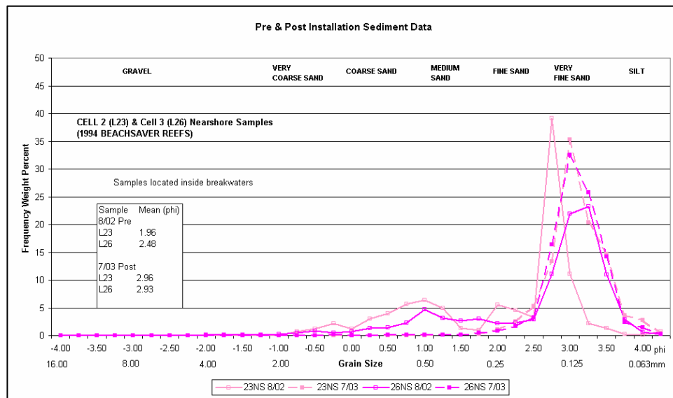
Figure A24. Sediment distribution change between 8/02 and 7/03 of nearshore samples in cells 2 and 3
