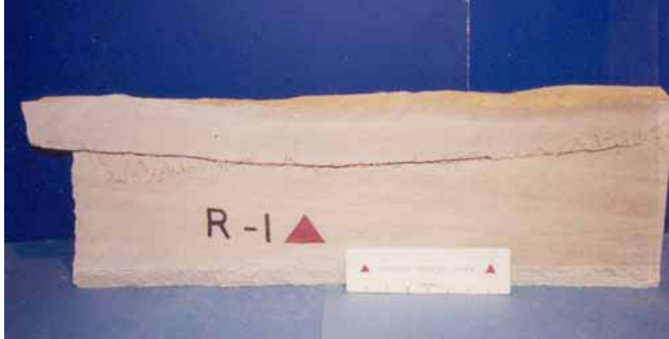
Figure 39. Reed Quarry Salem formation limestone accelerated weathering durability Test Block R-1-FT
