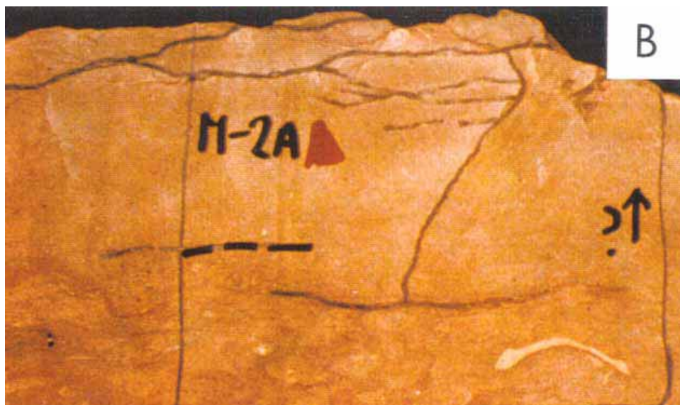
Figure 81. Marblehead Quarry Sample M-2A-WD showing fractures that are perpendicular and parallel to bedding. Dashed line indicates inferred orientation of bedding (after Agar)
