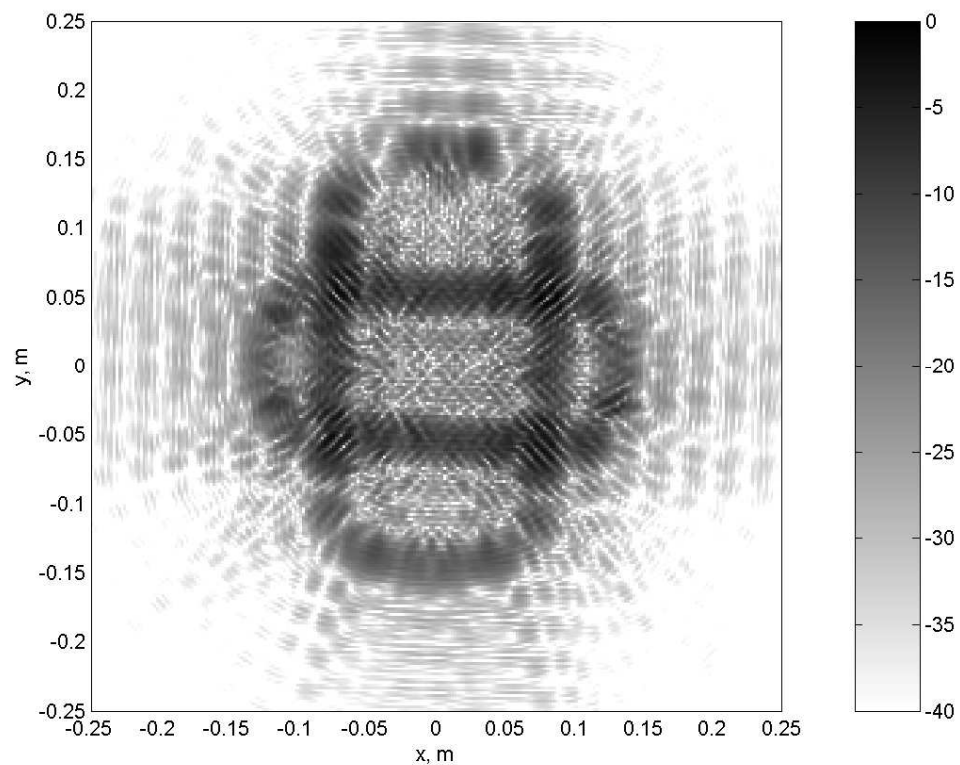
Figure 9.19: Fused LFM waveform images of true and aliased Civic targets. The aliased Civic was rotated 90^\circ and mismatched in Doppler by f_d = \text{PRF} . Range-Doppler coupling causes apparent expansion of the aliased target.
