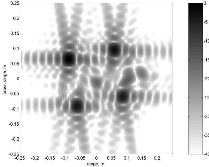
Figure 3.10: Focused ISAR image of four point scatterers. Scatterers are well focused. Sidelobes reflect the polar nature of the collected data ( \Delta\theta = 20^\circ , B = 6 GHz, 40.0 dB dynamic range).
