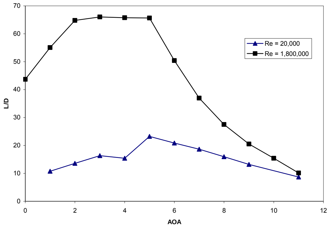
Figure 5.11 Efficiency comparison at wind tunnel and flight Reynolds numbers
