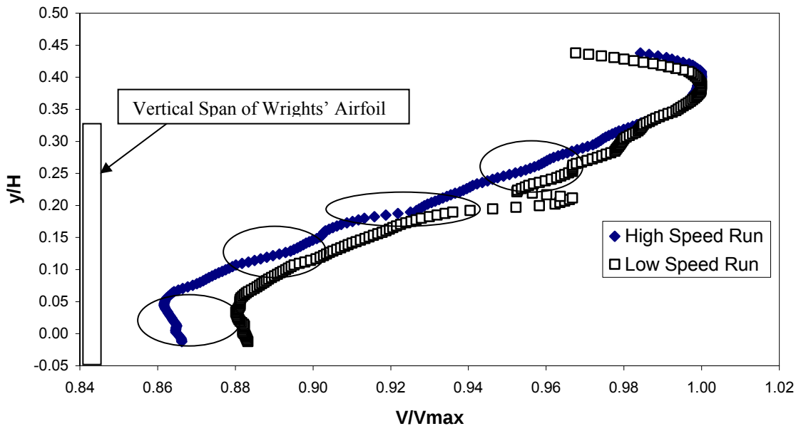
Figure 6.11 Comparison of high and low speed PIV data for the vertical centerline of the empty tunnel
