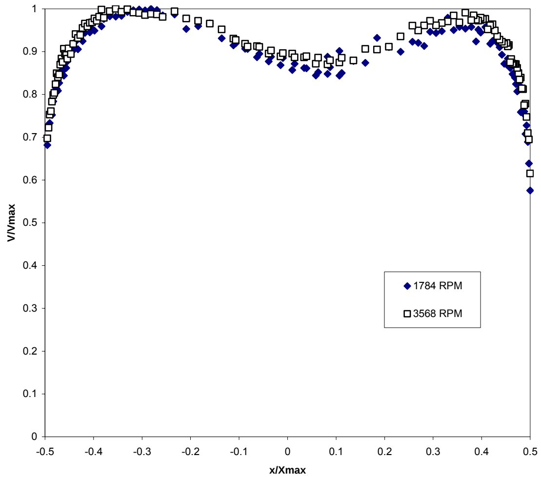
Figure 6.4 Overlay of nondimensional horizontal flow surveys at half and maximum RPM
