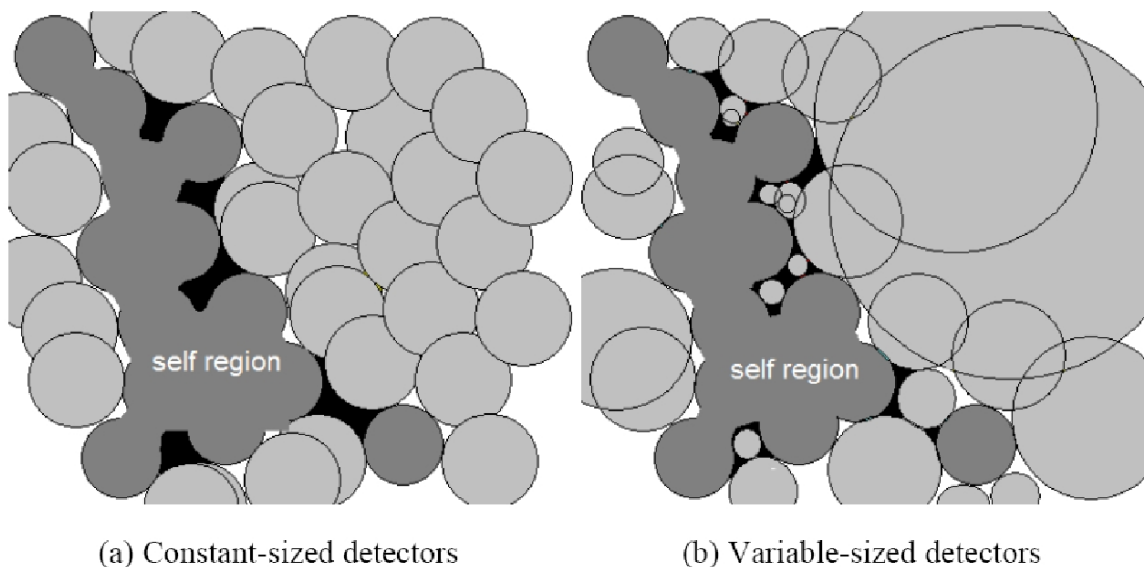
Figure 3: Covering nonself space with (a) constant-sized detectors and (b) variable-sized detectors. The black is uncovered space (as a result of the detectors not being granular enough), dark grey is self region and light grey is nonself detectors [40].
