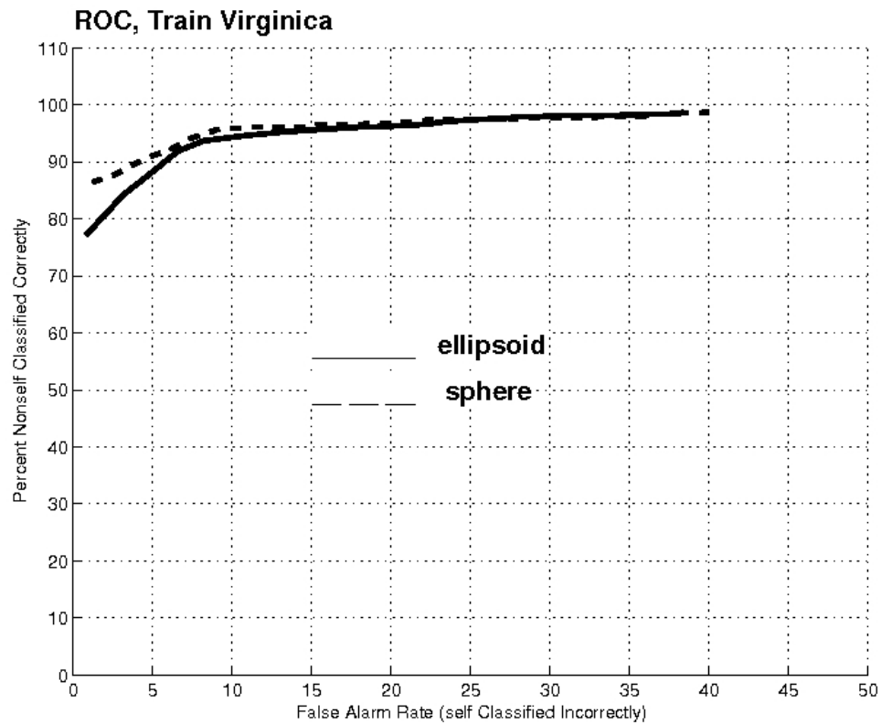
Figure 46: The ROC curve for ellipsoids and spheres when training on virginica (self). Nonsell is setosa and versicolor. The abscissa is the false alarm rate (percent of self points incorrectly classified). The ordinate is the percent of nonsell points correctly classified.
