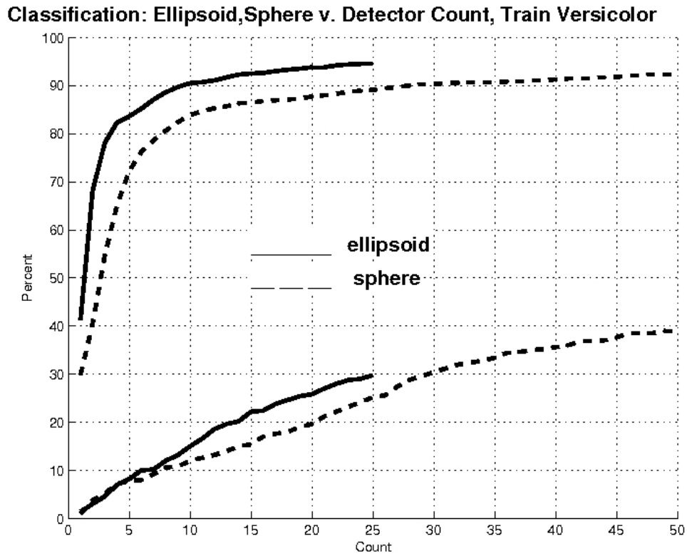
Figure 42: The upper two lines represent the percent of nonself (setosa and virginica) test points classified correctly using ellipsoids and spheres. The lower two lines represent the percent of self (versicolor) test points classified incorrectly using ellipsoids and spheres. The abscissa is the number of detectors that achieve the results shown.
