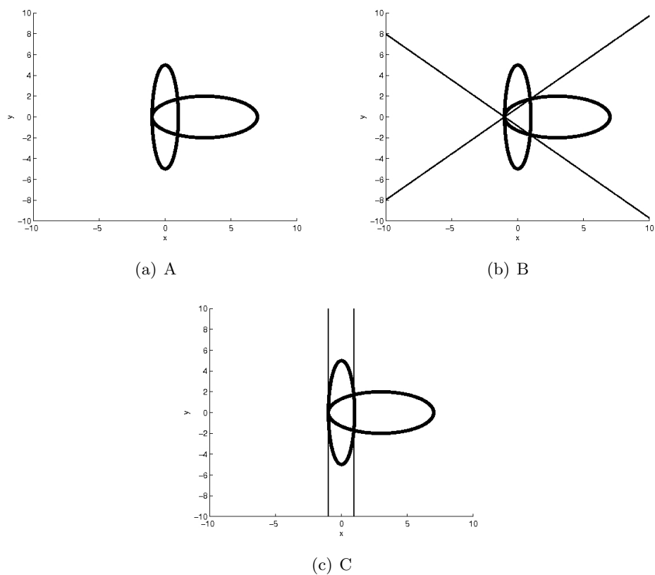
Figure 11: (A) shows 2 ellipsoids that intersect at exactly three points. (B) shows one degenerate conic, two intersecting lines, that passes through the three points of intersection. (C) shows a second degenerate conic, two parallel lines, that passes through the three points of intersection.
