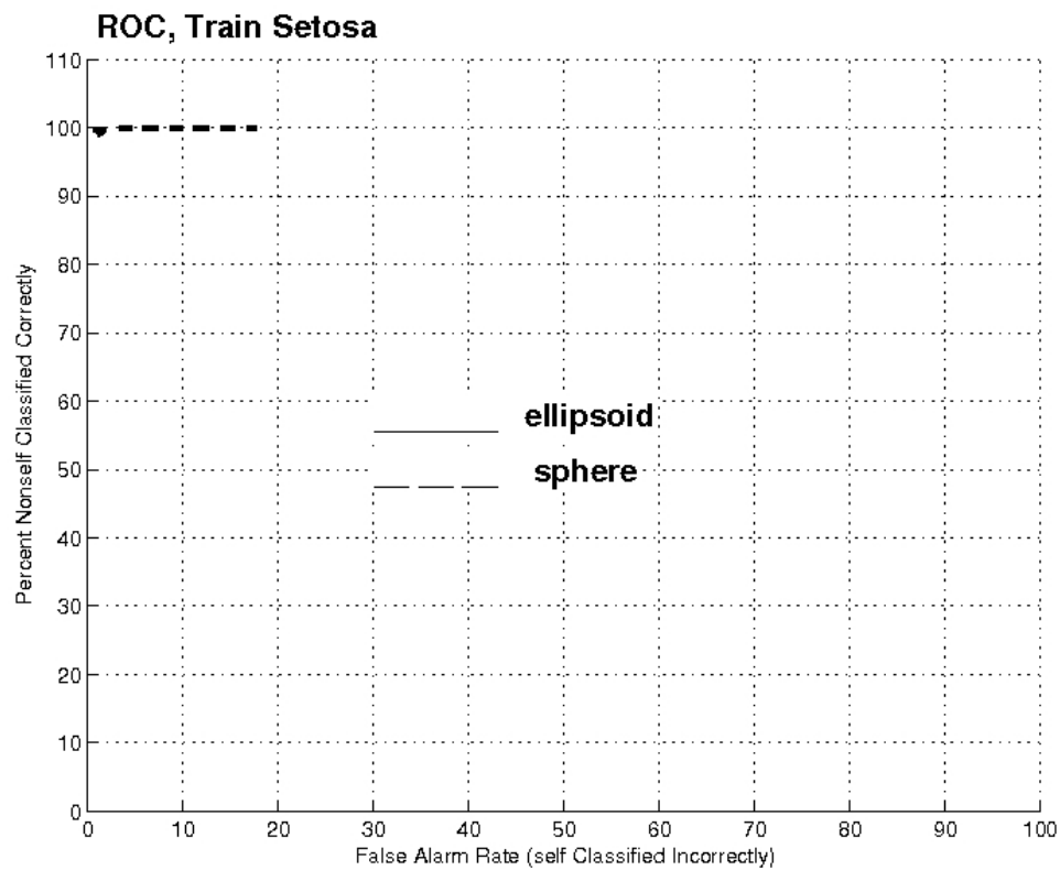
Figure 44: The ROC curve for ellipsoids and spheres when training on setosa (self). Nonsell is versicolor and virginica. The abscissa is the false alarm rate (percent of self points incorrectly classified). The ordinate is the percent of nonsell points correctly classified.
