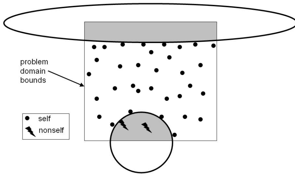
Figure 34: The ellipsoid has a better objective value than the sphere in the EA. However, the sphere performs “better” in classification because the nonself test happen to fall within the area it covers.
