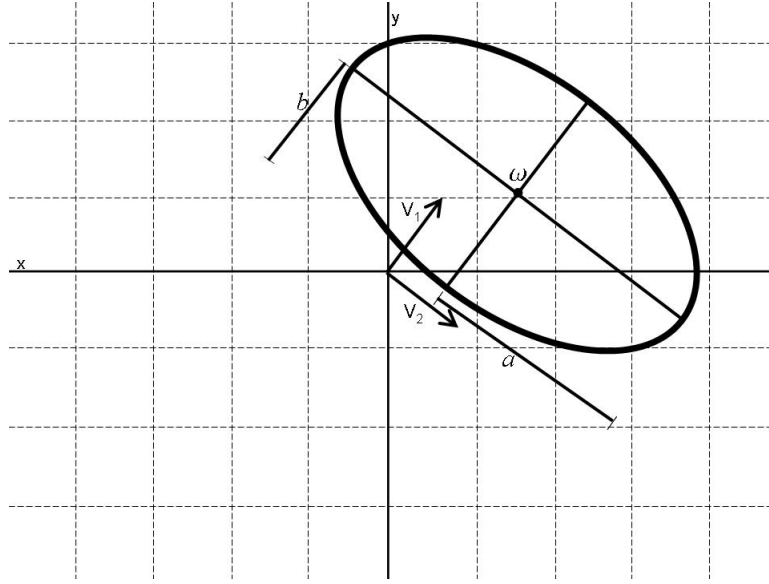
Figure 5: A graphical illustration of variables that define an ellipsoid.
