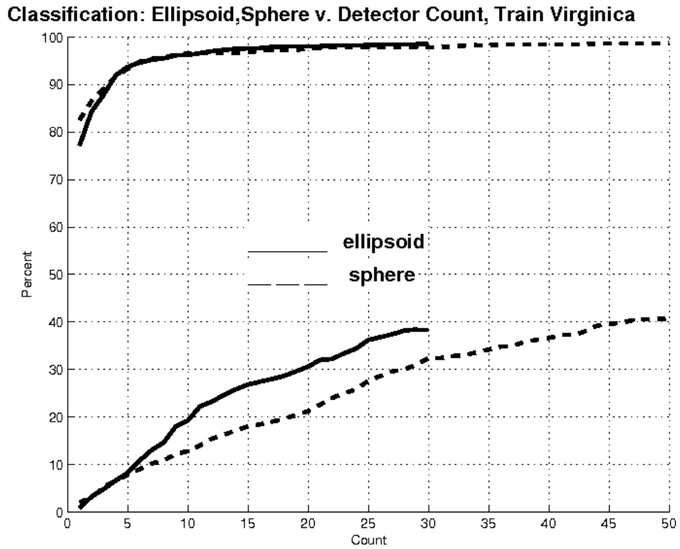
Figure 43: The upper two lines represent the percent of nonself (setosa and versicolor) test points classified correctly using ellipsoids and spheres. The lower two lines represent the percent of self (virginica) test points classified incorrectly using ellipsoids and spheres. The abscissa is the number of detectors that achieve the results shown.
