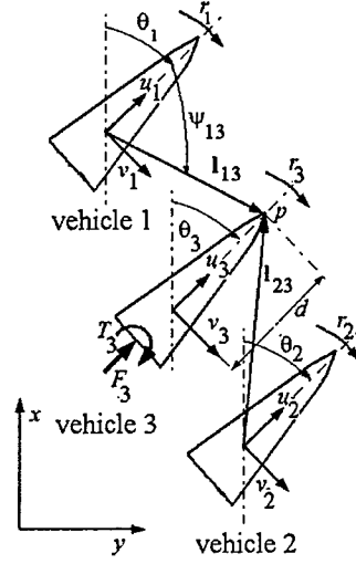
Figure 3: l-l Control Configuration
