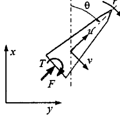
Figure 1: A 3 DOF Dynamic Model of a Vehicle
