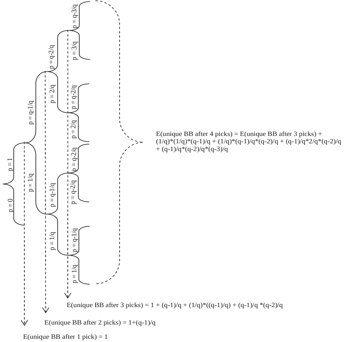
Figure 9: This figure illustrates the calculation for the expected number of unique BBs generated by a builder having q number of BBs available |\mathbb{BB}^*| .
