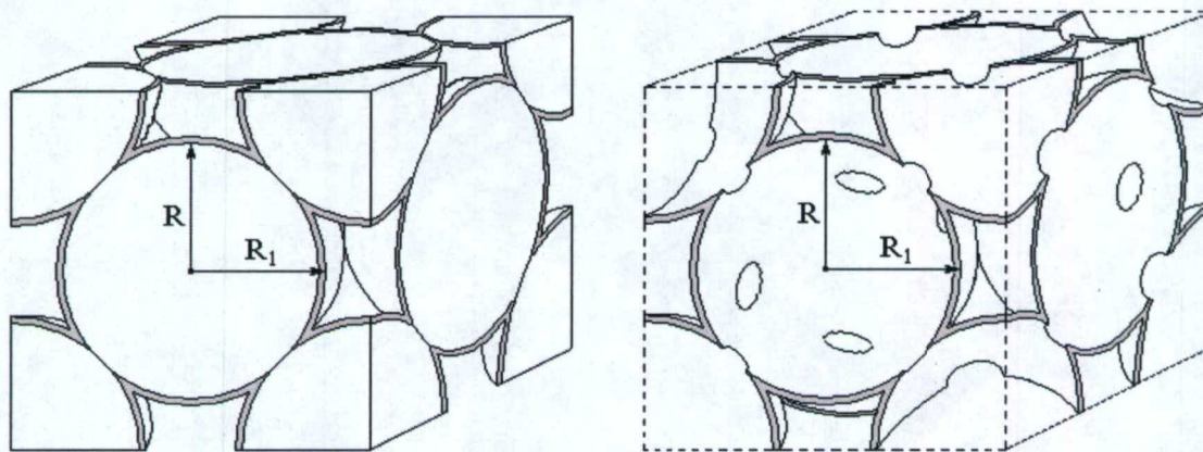
Fig.3.11: Schematic representation of surface-templated inverse opal.
