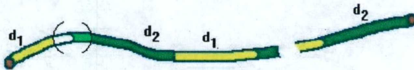
Fig.1.11: One-dimensional periodical chain. Tags d_1 and d_2 mark the length of alternating chain parts. Brackets show the physically small ranges of integration near the boundary.
